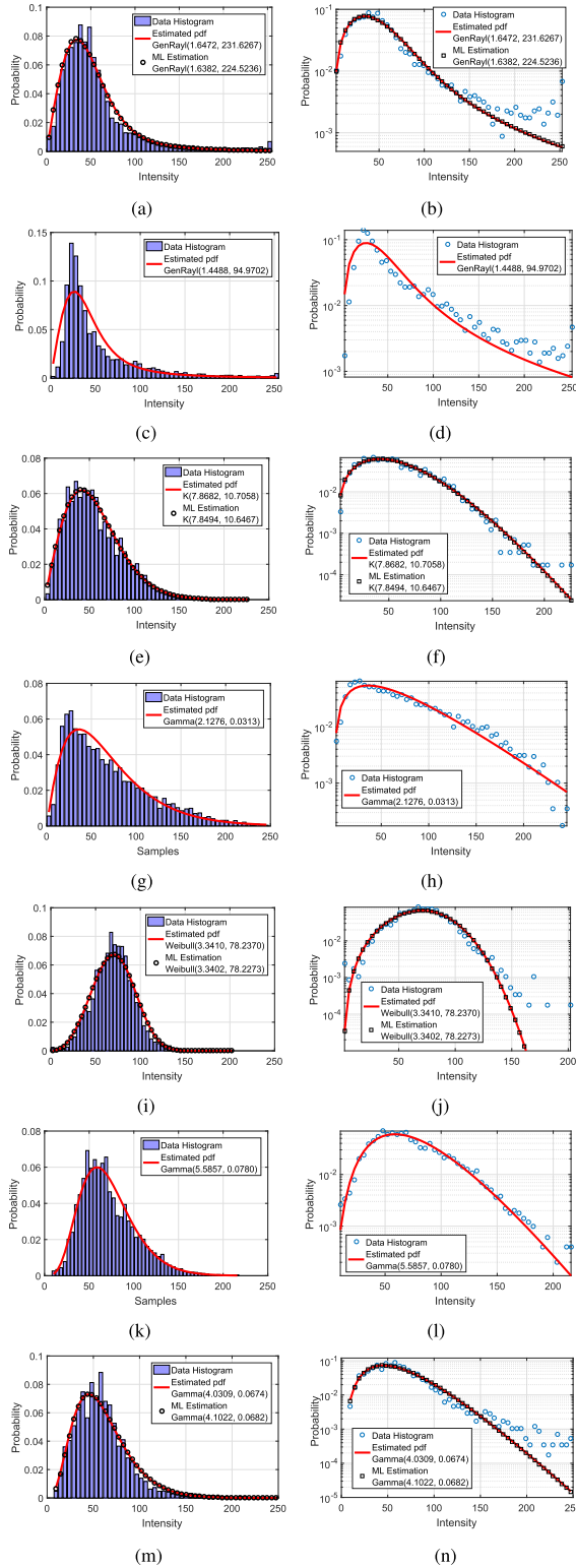
Fig. 4. SAR image distribution modeling results. Sub-figures on the left column refer to the estimated pdfs in linear scale, whereas the ones on the right column are in logarithmic scale. (a)-(b) Urban-X. (c)-(d) Urban-L. (e)-(f) Forest-X. (g)-(h) Forest-UHF. (i)-(j) Agricultural-X. (k)-(l) Agricultural-L. (m)-(n) Mixed-X.
