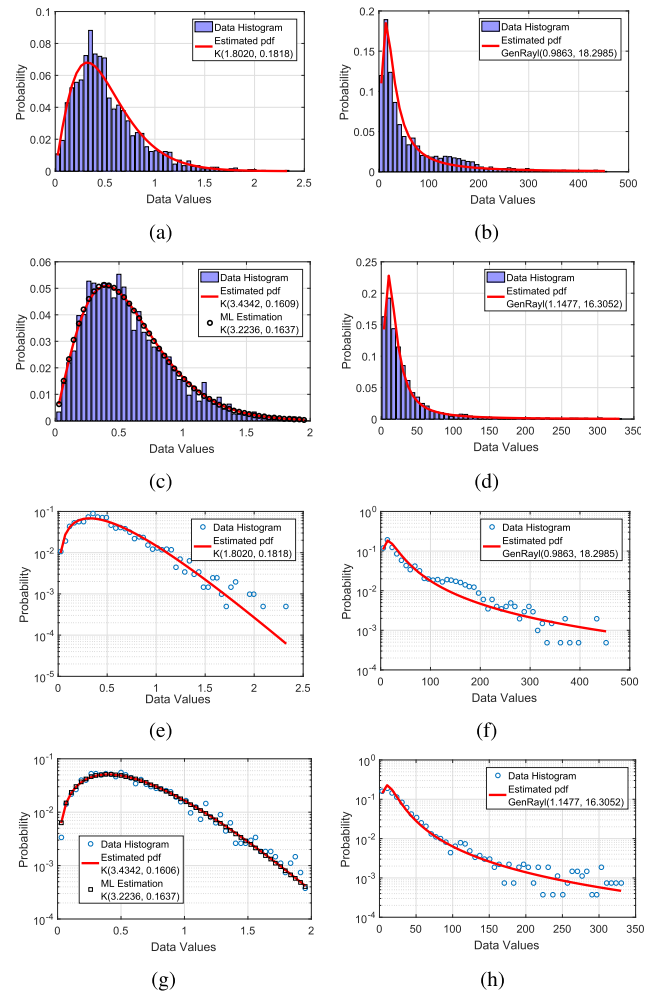
Fig. 5. US image distribution modeling results. (a)-(d): Estimated pdfs in linear scale, (e)-(h): Estimated pdfs in logarithmic scale. (a), (e) Cross (B). (b), (f) Cross (T). (c), (g) Long (B). (d), (h) Long (T).
