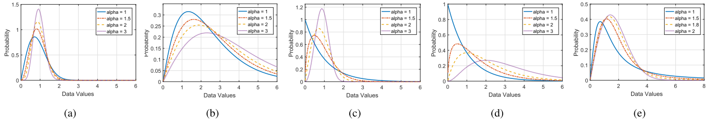
Fig. 1. Pdf of envelope distribution families for different values of the shape parameter \alpha . For all the families the scale parameter, \gamma = 1 . (a) Nakagami. (b) \mathcal{K} . (c) Weibull. (d) Gamma. (e) Generalized Rayleigh.
