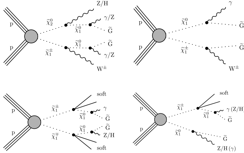
Fig. 1. In the context of GGM, several production and decay channels are possible. The diagram of the dominant process \tilde{\chi}_2^0 - \tilde{\chi}_1^\pm production is shown (upper left), where the gaugino decays depend on the mass configuration under study. In the TChiWg model (upper right), the gauginos are mass degenerate. The TChiNg model comprises \tilde{\chi}_1^\pm pair production (lower left) and \tilde{\chi}_1^\pm \tilde{\chi}_1^0 production (lower right), where the \tilde{\chi}_1^\pm is only slightly heavier than the \tilde{\chi}_1^0 , so only low-momentum (soft) particles appear in the decay of \tilde{\chi}_1^\pm to \tilde{\chi}_1^0 .
