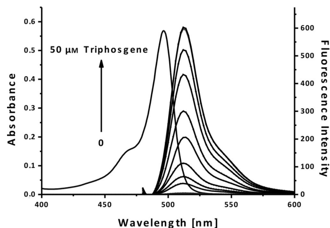
Figure 1. Absorbance and fluorescence spectra of BOD-SYR (10 \mu M) upon gradual addition of a solution of triphosgene (0–50 \mu M) in acetonitrile (CH 3 CN, with 0.1 % Et 3 N), \lambda_{ex} = 460 nm.
