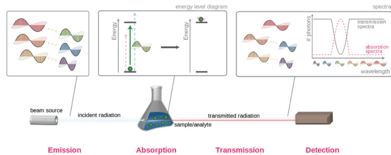
Figure 3.2. Experimental setup of absorption spectroscopy, from Wikipedia (2019)
