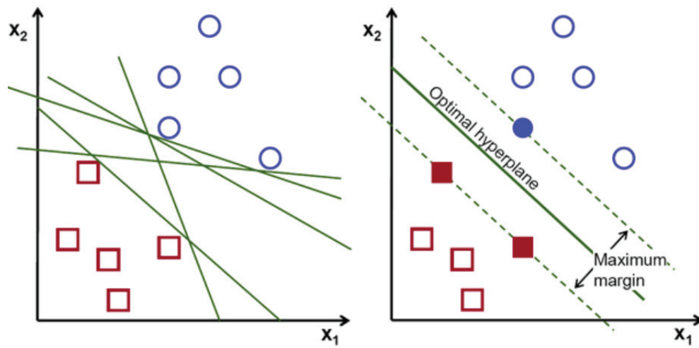
Figure 3.6. An example of support vector machine classification approach, from Towards Data Science (2019b)
