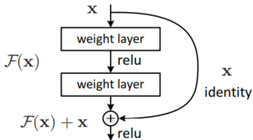
Figure 4. Residual learning: a building block from ResNet (Source: [9])
