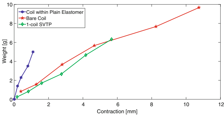
Fig. 5. The results of averaging 3 trials of compression for three separate individual coiled nylon actuators within either no elastomer (red), a plain elastomer sheet coating (blue) or an SVTP coating (green). (Color figure online)
