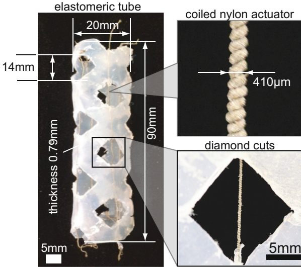
Fig. 1. Elastomeric-embedded coiled actuators as a tubular tissue phantom. Details show the coiled nylon actuator, and a portion of the elastomer with a diamond cut where the a coiled nylon actuator is exposed.
