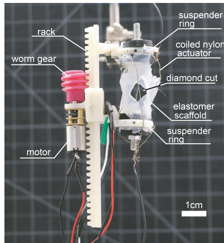
Fig. 4. The robotic implant setup with a 4-coil tubular SVTP.
