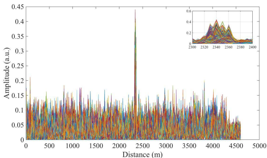
Figure 3: Absolute values of amplitude differences Inset: zoom on the PZT location.
