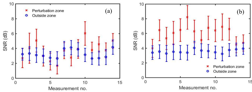
Fig. 5. SNR for measurements made using coherent detection for (a) low and (b) high acceleration.
