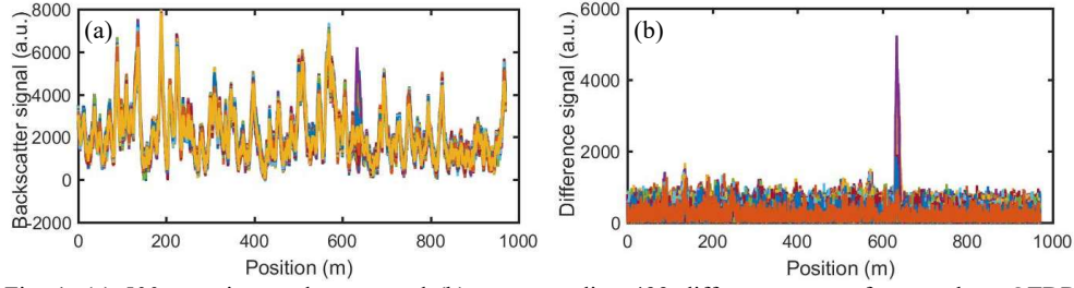
Fig. 1. (a) 500 superimposed traces and (b) corresponding 499 difference traces from a phase-OTDR measurement of a vibration event at the position 635 m.
