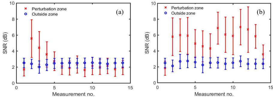
Fig. 3. SNR for measurements made using direct detection for (a) low and (b) high acceleration.
