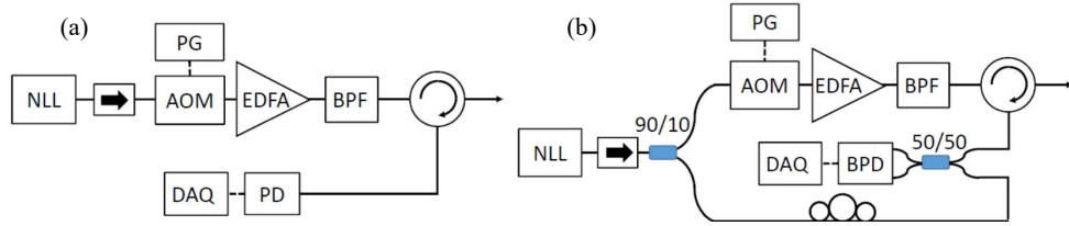
Fig. 2. Phase-OTDR setup using (a) direct detection and (b) coherent detection; NLL = narrow linewidth laser, AOM = acousto-optic modulator, PG = pulse generator, EDFA = fiber amplifier, BPF = band pass filter, PD = photo-receiver, DAQ = data acquisition card, BPD = balanced photo-receiver, \rightarrow = isolator, oOo = polarization controller.
