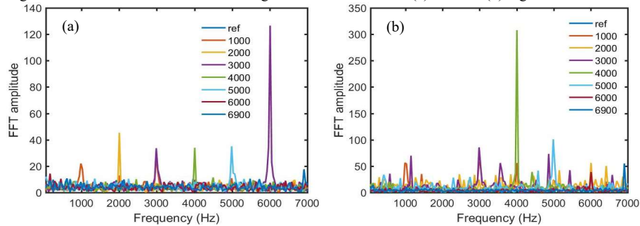
Fig. 6. Frequency spectrum for 800 traces with coherent detection for (a) low and (b) high acceleration.
