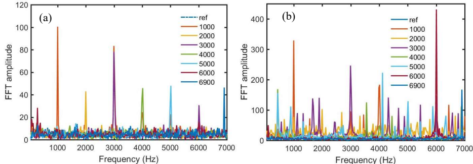
Fig. 4. Frequency spectrum for 800 traces with direct detection for (a) low and (b) high acceleration.
