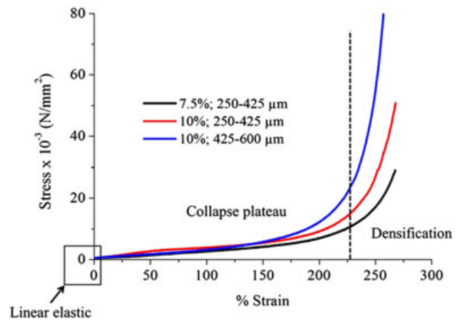
Figure 3. Stress–strain curves from the mechanical test of nanofibrous scaffolds
