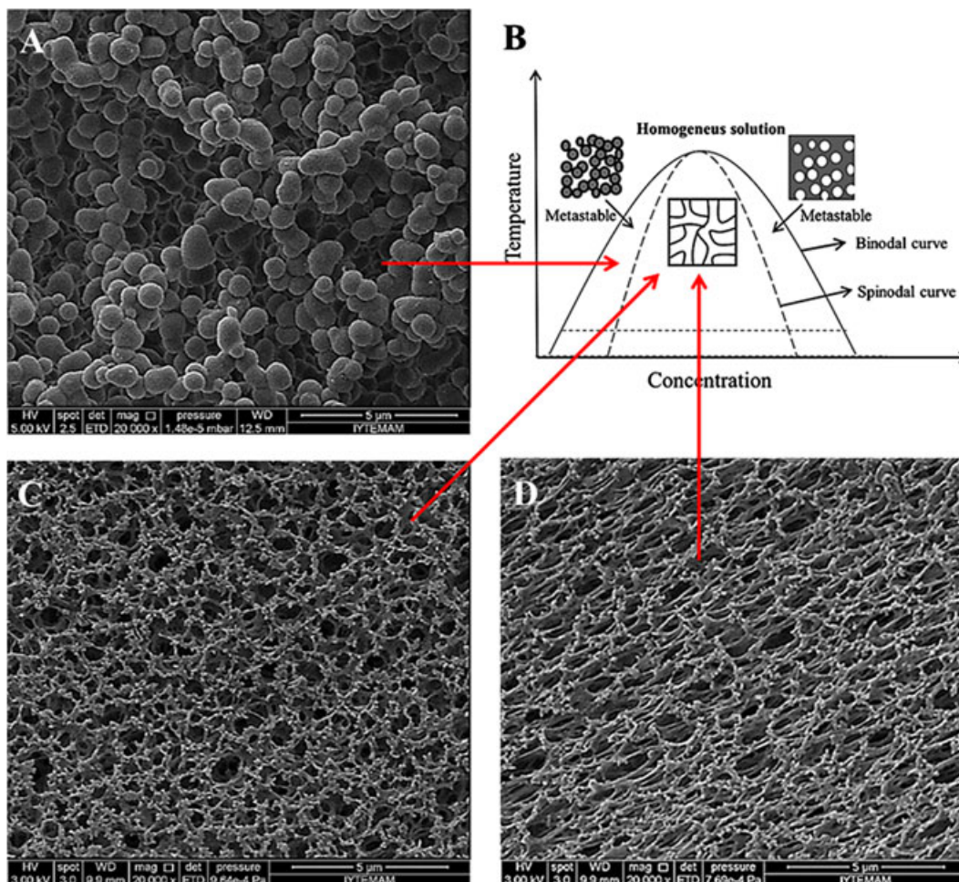
Figure 1. Scaffolds prepared from 5% (A), 7.5% (C) and 10% (D) gelatine solution \times 5000 . (B) Schematic phase diagram of polymer solution
