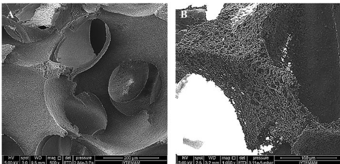
Figure 2. Nanofibrous scaffolds prepared with 10% gelatine concentration, 200 min preheating time and 425–600 \mu\text{m} sized paraffin spheres
