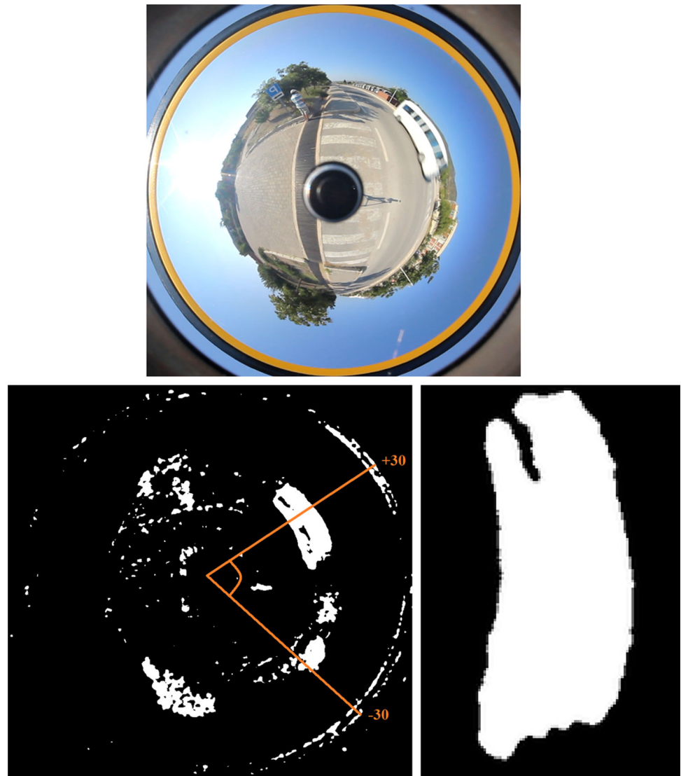
Fig. 2 Top An example omnidirectional video frame containing a van. Bottom-left The same frame after background subtraction. Also the angle range that we used, namely [30^\circ, -30^\circ] , is superimposed on the image. Centroid of the largest blob is at 29^\circ . Bottom-right Rotated blob after morphological operations
