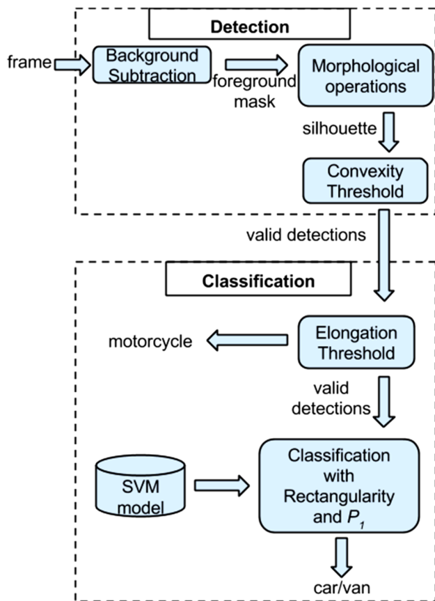
Fig. 4 Block diagram of the detection and classification system. With the proposed method, multiple frames are processed and the extracted average silhouette is used instead of a silhouette from a single frame
