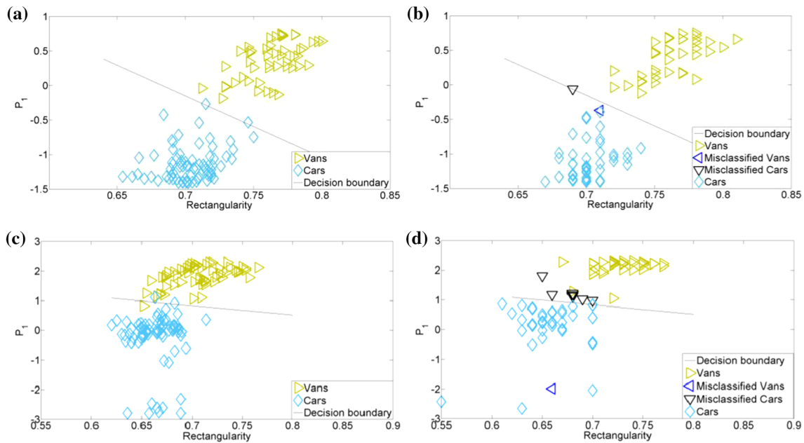
Fig. 6 a Training result of SVM using the average silhouette method. b Test result with the average silhouette method. c Training result of SVM without averaging silhouettes (single-frame method). d Test result without averaging silhouettes, i.e. using single-frame silhouettes
