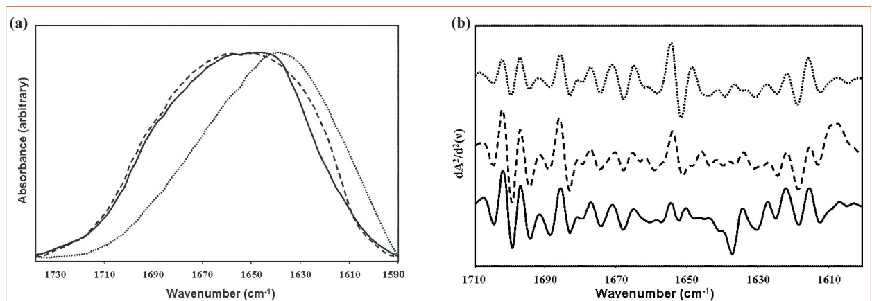
Figure 3. The average (a) absorbance and (b) second derivative spectra of original trypsin, trypsin gel and trypsin aggregate in 1700-1600 \text{cm}^{-1} region (continuous line shows original trypsin, dashed line shows trypsin gel, dotted line shows trypsin aggregate).
