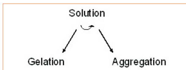
Figure 5. The proposed model for trypsin phase behavior.
