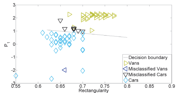
Figure 10: Test result without averaging silhouettes, i.e. using single frame silhouettes.
