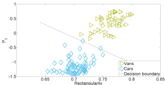
Figure 7: Training result of SVM using the average silhouette method.
