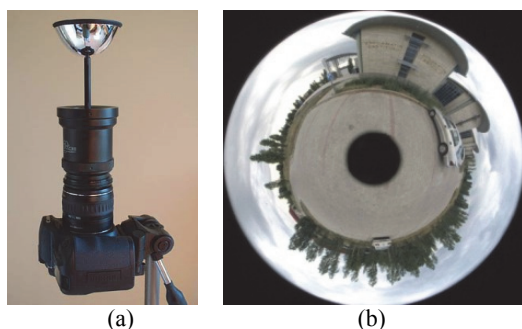
Figure 1: (a) A mirror apparatus is placed in front of a conventional camera to obtain a catadioptric omnidirectional camera. (b) An example image obtained by such a camera.
