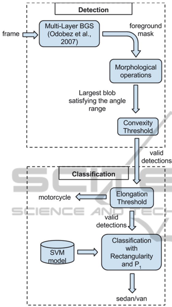
Figure 5: Block diagram of the detection and classification system. With the proposed method, multiple frames are processed and the extracted average silhouette is used instead of a silhouette from a single frame.
