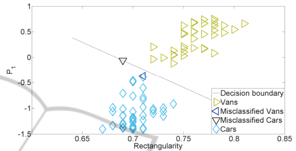
Figure 8: Test result with the average silhouette method.
