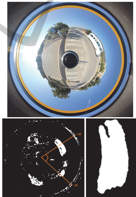
Figure 2: Top: An example omnidirectional video frame containing a van while passing a road. Bottom-left: The same frame after background subtraction. Also the angle range that we used, namely [30^\circ, -30^\circ] , is superimposed on the image. Centroid of the largest blob is at 29^\circ . Bottom-right: Rotated blob after morphological operations.
