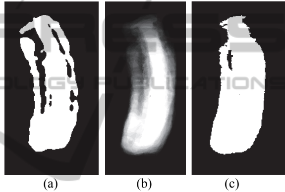
Figure 12: Example van silhouettes (a) silhouette from a single frame which is eliminated since \rho = 0.548 , (b) average silhouette (c) thresholded average silhouette which is not eliminated since \rho = 0.823 .
