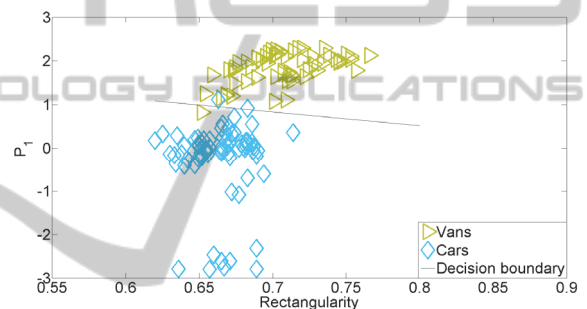
Figure 9: Training result of SVM without averaging silhouettes (single frame method).
