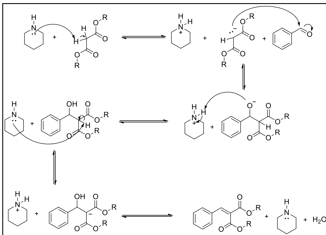
Figure 1.26. Reaction mechanism of Knoevenagel Condensation (Source: Knoevenagel, 1898)
