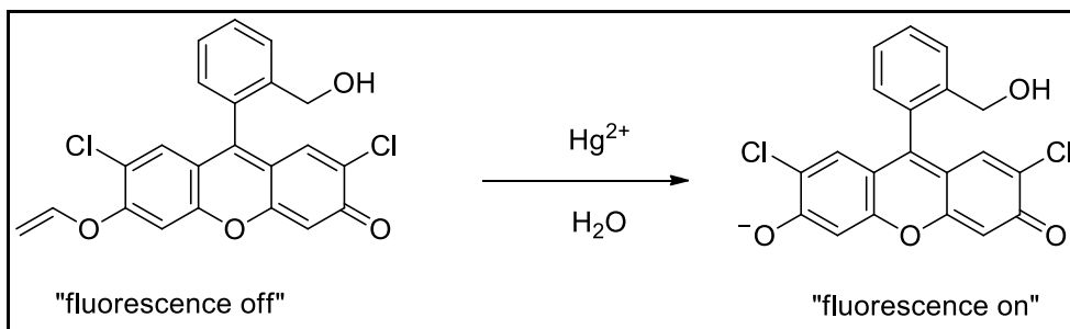
Figure 3.20. \text{Hg}^{2+} selective turn on sensor bearing vinyl ether structure (Source: Santra et al., 2009)
