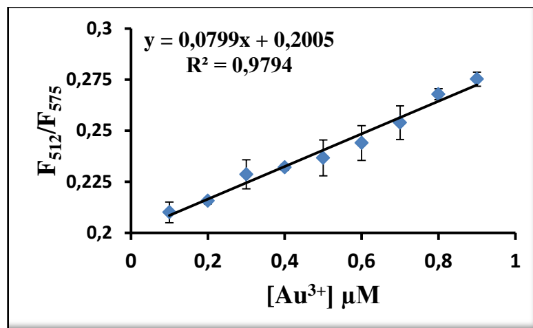
Figure 2.57. Fluorescence changes of BOD-5 (10.0 μM) upon addition of Au 3+ (0.1 to 0.9 μM, 0.01 to 0.09 equiv.) in 0.1M potassium phosphate buffer, pH 7.0/EtOH (v/v, 7:3) ( \lambda_{\text{ex}} : 460 nm, emission wavelengths: \lambda_{512}/\lambda_{575} at 25 °C).
