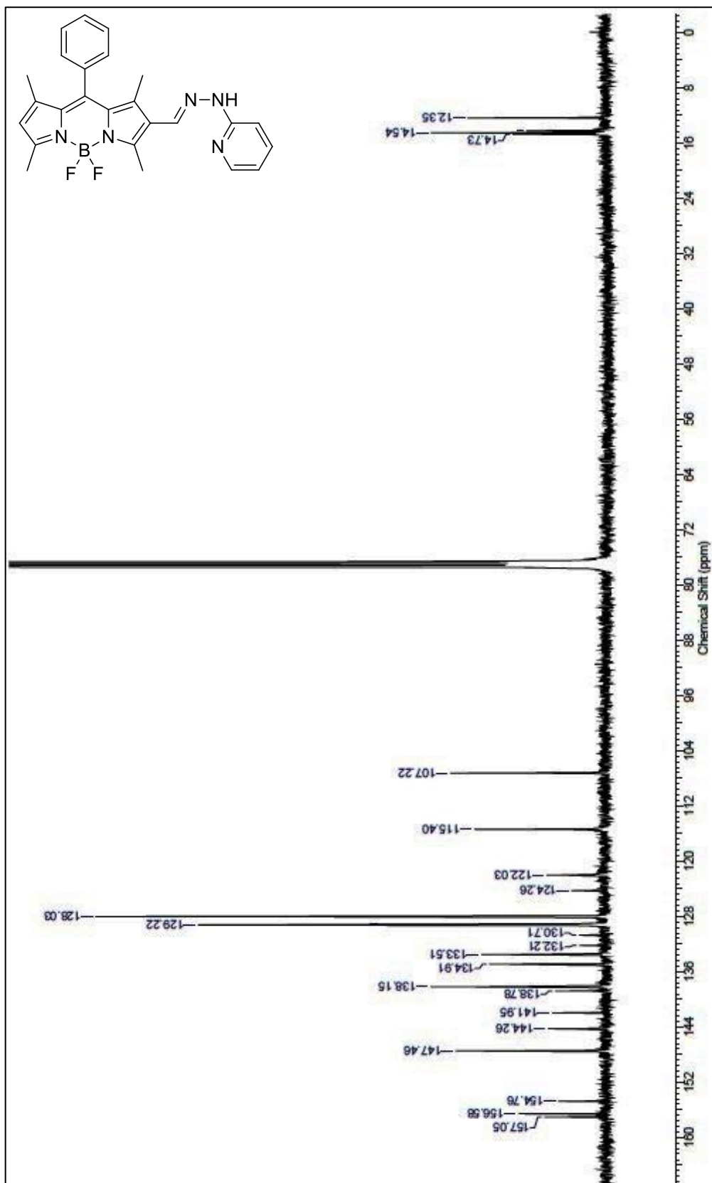
Figure A.6. 13 C NMR of (E)-5,5-difluoro-1,3,7,9-tetramethyl-10-phenyl-8-((2-(pyridin-2-yl)hydrazono)methyl)-5H-dipyrrolo[1,2-c:2',1'-f][1,3,2]diazaborinin-4-ium-5-uide
