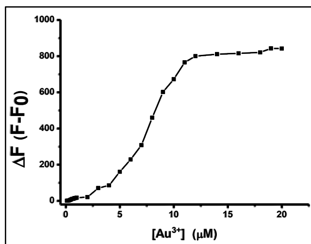
Figure 2.79. Calibration curve of BOD-6 (10 \mu\text{M} ) in the presence of increasing concentrations of \text{Au}^{3+} (0-20 \mu\text{M} , 0-2 equiv.) in dichloroethane ( \lambda_{\text{exc}}=500 \text{ nm} , \lambda_{\text{em}}=570 \text{ nm} at 25 ^{\circ}\text{C} ).
