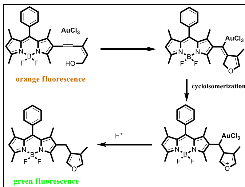
Figure 2.61. Proposed mechanism for \text{Au}^{3+} triggered intramolecular cyclization
