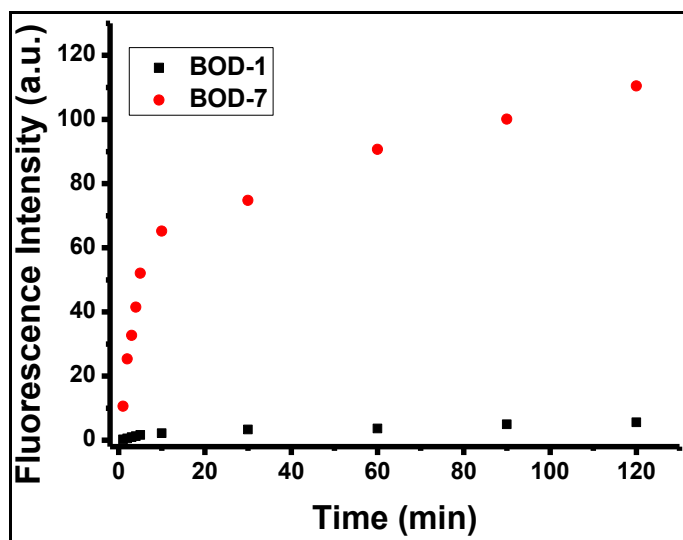
Figure 2.22. Fluorescence responses of BOD-1 (10 \mu\text{M} ) and BOD-7 (10 \mu\text{M} ) in reaction conditions (0.1 M phosphate buffer/EtOH (pH 7.0, v/v, 1:1) without addition of \text{Au}^{3+} . ( \lambda_{\text{exc}}=460 nm, \lambda_{\text{em}}= 512 nm at 25 ^{\circ}\text{C} ).
