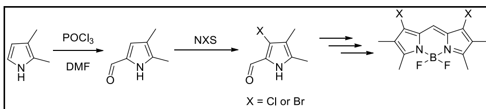
Figure 1.29. Synthesis route of 1,7-bis-halogenated BODIPYs. (Source: Boens et al., 2015)
