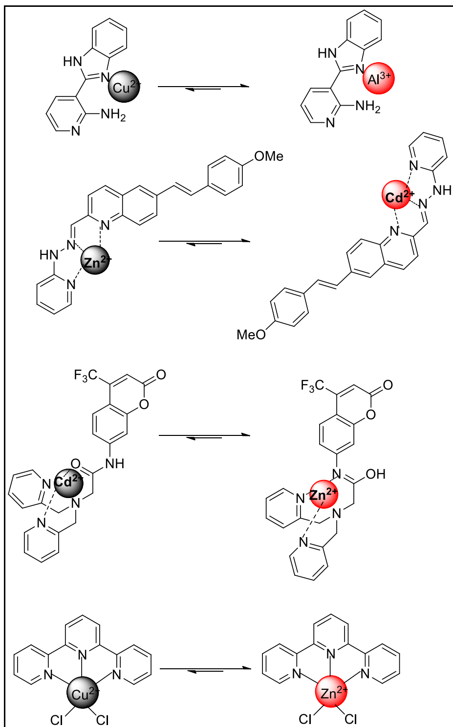
Figure 1.42. Examples of chemosensors working via cation exchange reaction (Source: Cheng et al., 2015)
