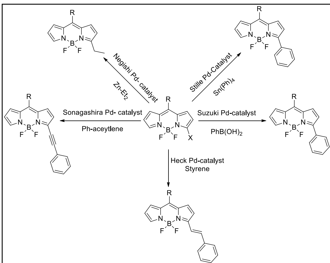
Figure 1.24. Pd catalyzed derivatization of BODIPYs from 3- and 3,5- positions (Source: Lakshmi et al., 2015)
