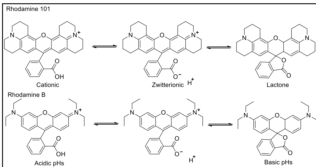
Figure 1.5. The structural forms of Rhodamine 101 and Rhodamine B in acidic and basic media (Source: Beija et al., 2009)
