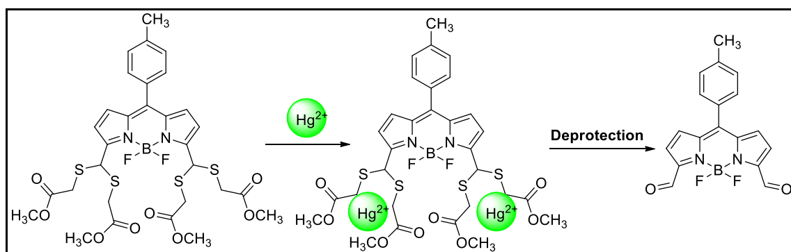
Figure 3.17. BODIPY based chemodosimeter working via deprotection mechanism (Source: Madhu et al., 2012)
