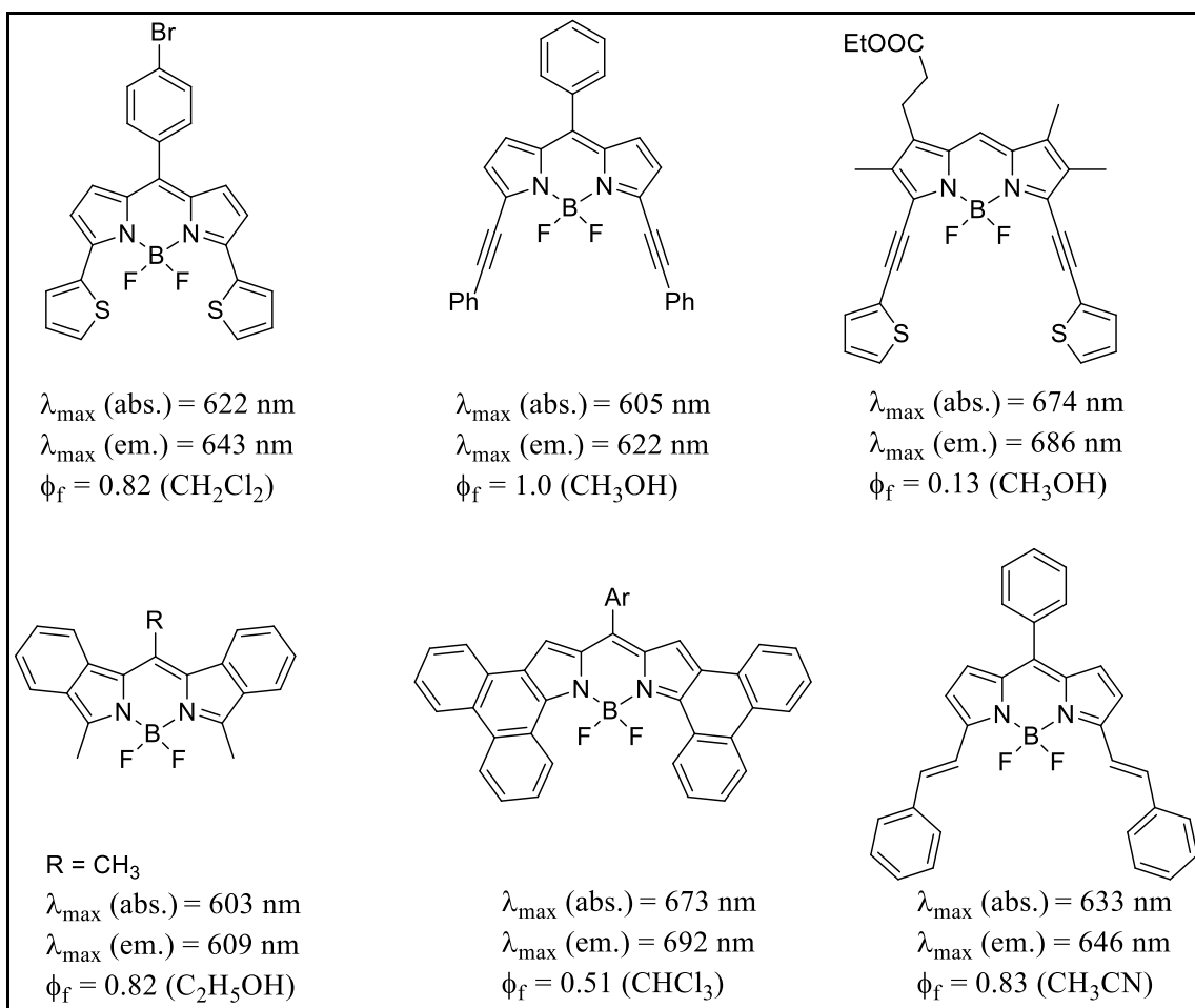
Figure 1.19. BODIPY structures with extended conjugation (Source: Ni and Wu, 2014)
