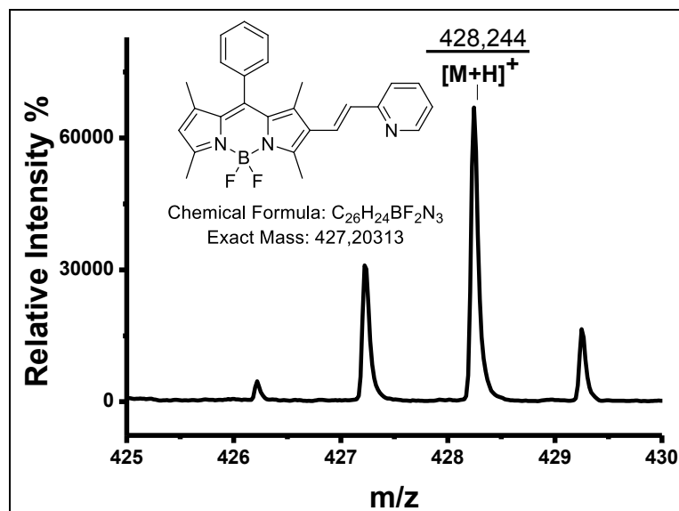
Figure B.9. Mass Spectrum of BOD-6 ((E)-5,5-difluoro-1,3,7,9-tetramethyl-10-phenyl-8-(2-(pyridin-2-yl)vinyl)-5H-dipyrrolo[1,2-c:2',1'-f][1,3,2]diazaborinin-4-ium-5-uide)
