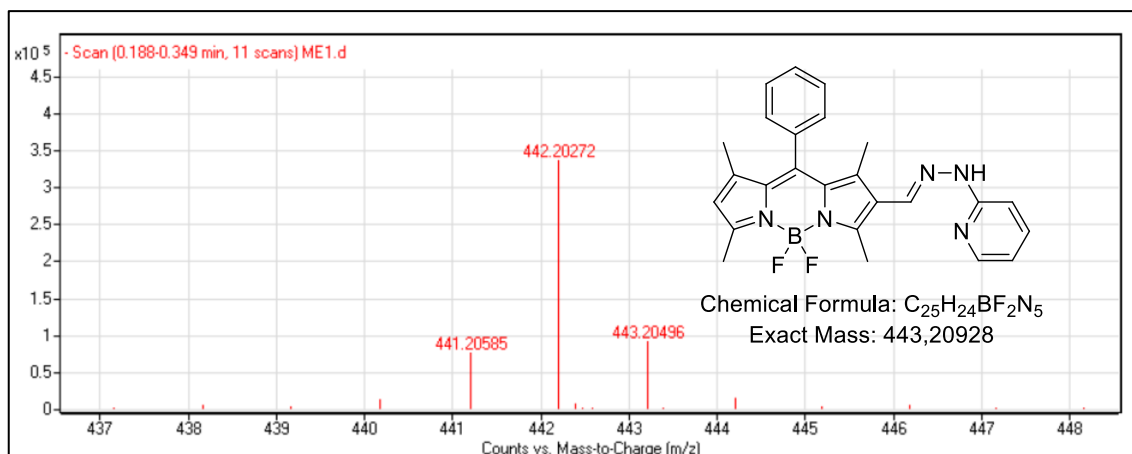
Figure B.1. (E)-5,5-difluoro-1,3,7,9-tetramethyl-10-phenyl-8-((2-(pyridin-2-yl)hydrazono)methyl)-5H-dipyrrolo[1,2-c:2',1'-f][1,3,2]diazaborinin-4-ium-5-uide
