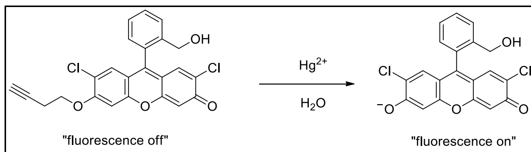
Figure 3.18. First example of \text{Hg}^{2+} sensor bearing alkyne moiety (Source: Song et al., 2008)
