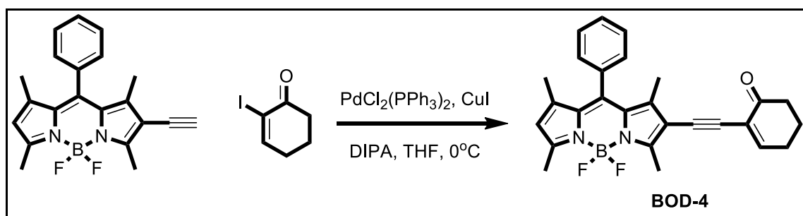
Figure 2.44. Synthesis route of BOD-4
