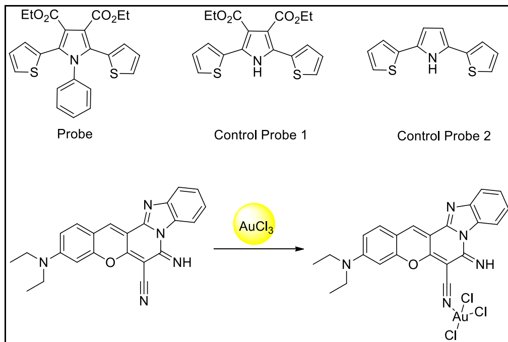
Figure 2.11. Non-reaction based \text{Au}^{3+} ion sensors (Source: Öztaş et al., 2013; Yang et al., 2013)
