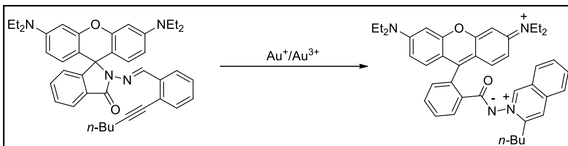
Figure 2.6. Rhodamine based gold ion sensor developed by Emrullahoglu research group (Source: Emrullahoglu et al., 2013)
