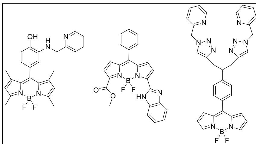
Figure 3.10. BODIPY based chemosensors for \text{Hg}^{2+} ions (Source: Chang et al., 2015)
