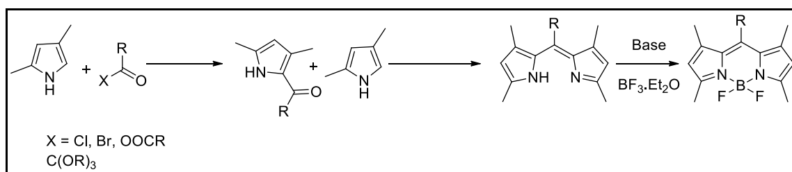
Figure 1.14. Synthesis of BODIPY dyes with the acylation of pyrrole followed by condensation and complexation (Source: Boens et al., 2012)
