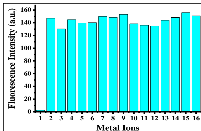
Figure 2.40. Fluorescence intensities of BOD-3 (10 \mu\text{M} ) in 0.1 M phosphate buffer/EtOH (pH = 7.0, v/v, 1:4) in the presence of \text{Au}^{3+} and 20.0 equiv. (200 \mu\text{M} ) of the cations interest: 1, BOD-3 only; 2, \text{Au}^{3+} ; 3, \text{Au}^+ ; 4, \text{Ba}^{2+} ; 5, \text{Ca}^{2+} ; 6, \text{Cd}^{2+} ; 7, \text{Cr}^{3+} ; 8, \text{Cu}^{2+} ; 9, \text{Fe}^{3+} ; 10, \text{K}^+ ; 11, \text{Li}^+ ; 12, \text{Mg}^{2+} ; 13, \text{Ni}^{2+} ; 14, \text{Zn}^{2+} ; 15, \text{Ag}^+ ; 16, \text{F}^- ( \lambda_{\text{ex}} = 460 \text{ nm} , \lambda_{\text{em}} = 480 \text{ nm} ).
