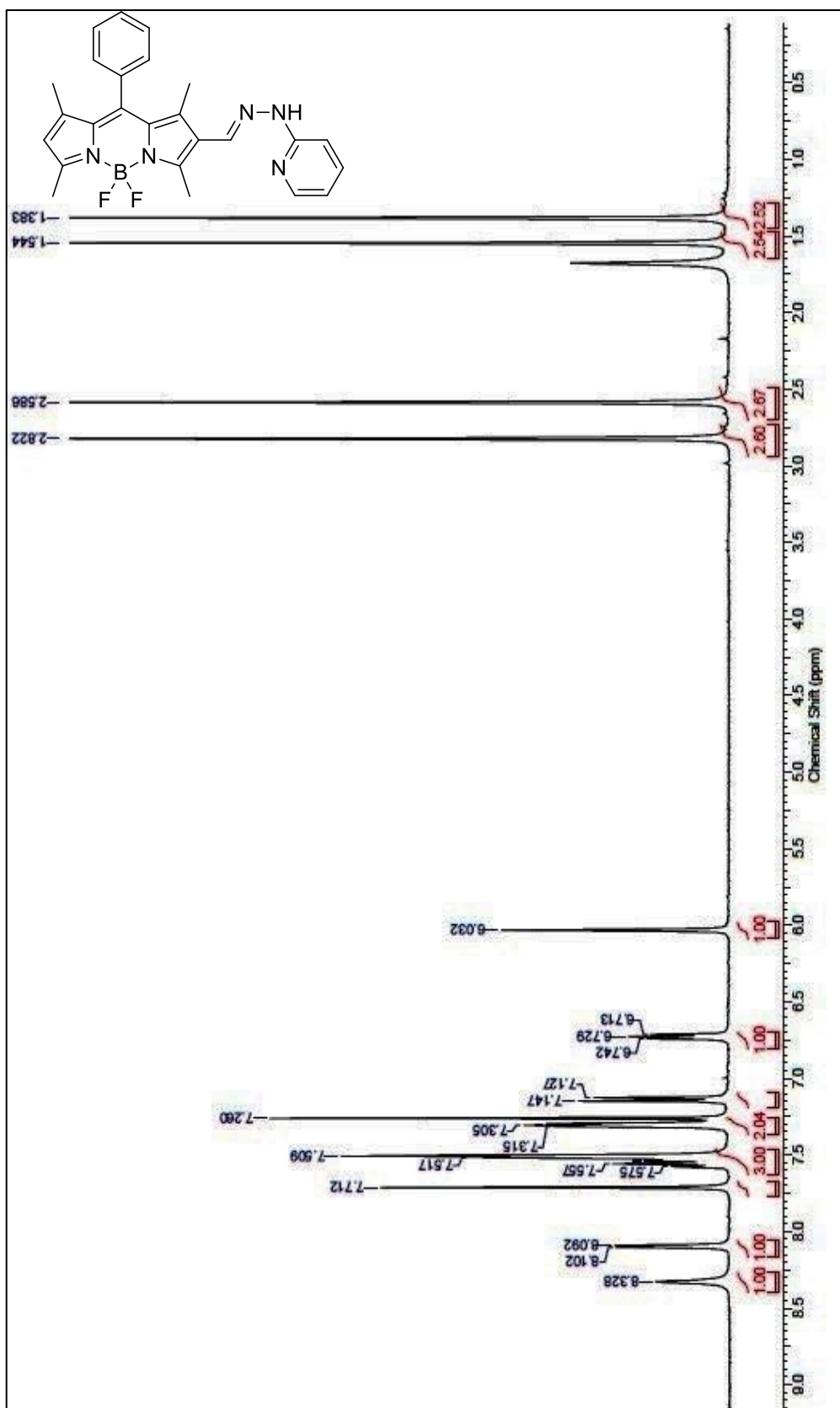
Figure A.5. 1 H NMR of (E)-5,5-difluoro-1,3,7,9-tetramethyl-10-phenyl-8-((2-(pyridin-2-yl)hydrazono)methyl)-5H-dipyrrolo[1,2-c:2',1'-f][1,3,2]diazaborin-4-ium-5-uide
