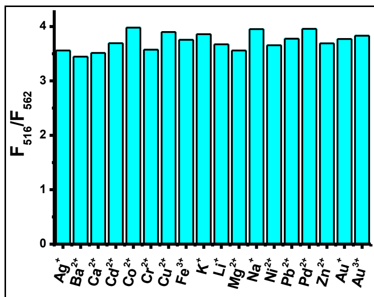
Figure 3.44. Fluorescence intensities of BOD-4 (5 \mu\text{M} ) in the presence of \text{Hg}^{2+} (25 \mu\text{M} , 2 equiv.) and 10 equiv. of other metal ions in 0.1 M phosphate buffer/EtOH (pH 7.0, v/v, 6:4) ( \lambda_{\text{exc}}=460 nm at 25 ^\circ\text{C} ).
