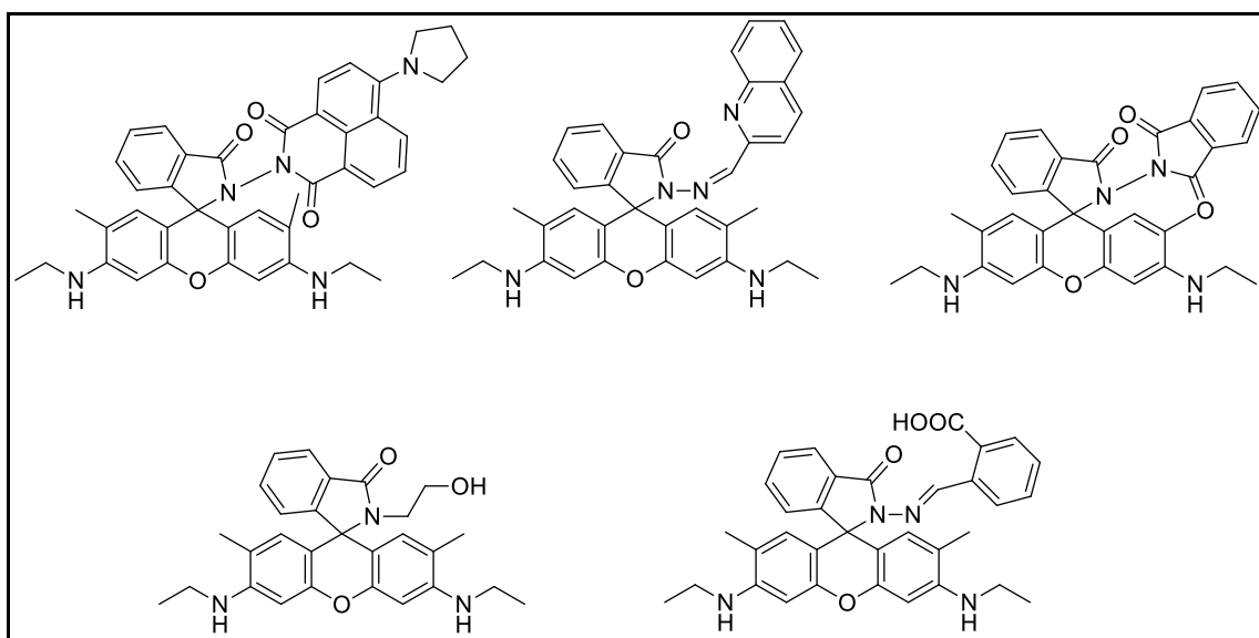
Figure 3.7. Rhodamine based chemosensors for \text{Hg}^{2+} (Source: Chen et al., 2015)
