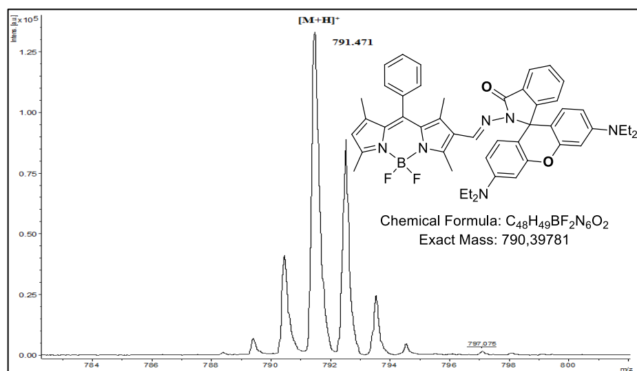
Figure B.2. MALDI-TOF Spectra of BOD-8 ((E)-8-(((3',6'-bis(diethylamino)-3-oxospiro[isoindoline-1,9'-xanthen]-2-yl)imino)methyl)-5,5-difluoro-1,3,7,9-tetramethyl-10-phenyl-5H-dipyrrolo[1,2-c:2',1'-f][1,3,2]diazaborinin-4-ium-5-uide)
