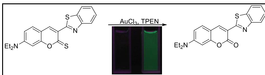
Figure 2.9. Detection of \text{Au}^{3+} ions via desulfation reaction (Source: Park et al., 2012)
