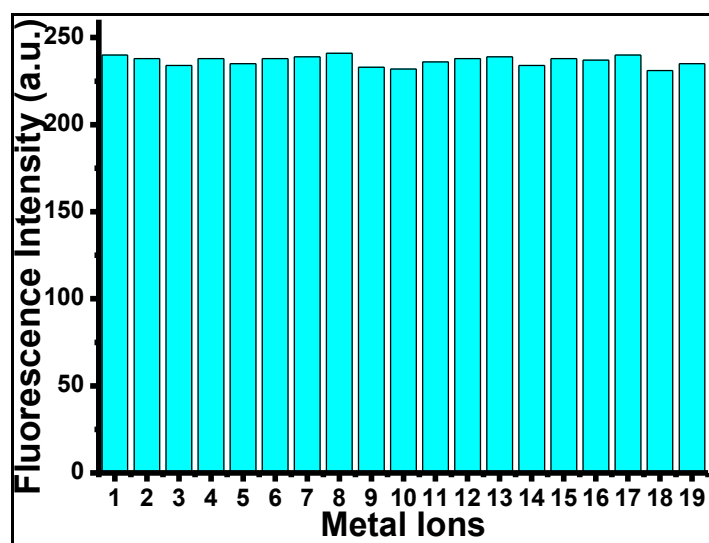
Figure 2.30. Fluorescence intensities of BOD-2 (5 \mu\text{M} ) in 1:1 \text{CH}_3\text{CN} /HEPES buffer at \text{pH} = 7.0 at \lambda_{\text{max}} : 505 nm in the presence \text{Au}^{3+} (1.0 equiv.) and 10.0 equiv. of the following metal ions: 1, none; 2, \text{Au}^+ ; 3, \text{Cu}^{2+} ; 4, \text{Zn}^{2+} ; 5, \text{Pb}^{2+} ; 6, \text{Ni}^{2+} ; 7, \text{Na}^+ ; 8, \text{Mg}^{2+} ; 9, \text{Li}^+ ; 10, \text{K}^+ , 11, \text{Pd}^{2+} ; 12, \text{Fe}^{2+} ; 13, \text{Co}^{2+} ; 14, \text{Cd}^{2+} ; 15, \text{Ca}^{2+} ; 16, \text{Ba}^{2+} 17, \text{Ag}^+ ; 18, \text{Cr}^{3+} ; 19, \text{Fe}^{3+}
