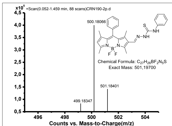
Figure B.4. Mass Spectrum of BOD-3 ((E)-5,5-difluoro-1,3,7,9-tetramethyl-10-phenyl-8-((2-(phenylcarbamothioyl)hydrazono)methyl)-5H-dipyrrolo[1,2-c:2',1'-f][1,3,2]diazaborinin-4-ium-5-uide)
