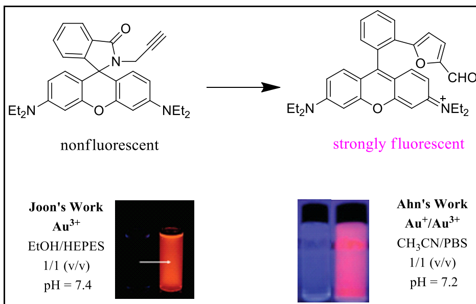
Figure 2.2. Rhodamine-propargylamide based fluorescent sensor for gold ions (Source: Jou et al., 2009; Egorova et al., 2010)
