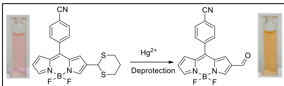
Figure 3.16. BODIPY based chemodosimeter working via deprotection mechanism (Source: Zhang et al., 2012)
