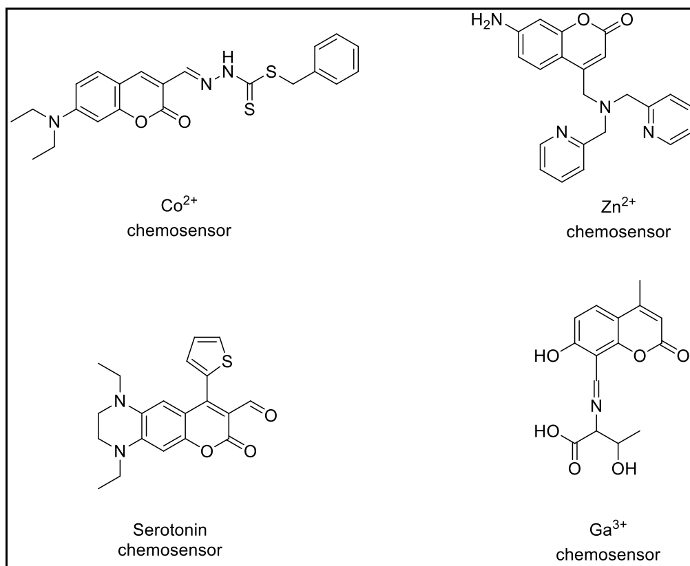
Figure 1.7. Coumarin based fluorescent sensors (Source: Liu et al., 2015; Aulsebrook et al., 2015; Hettie and Glass, 2016; Yan et al., 2016)
