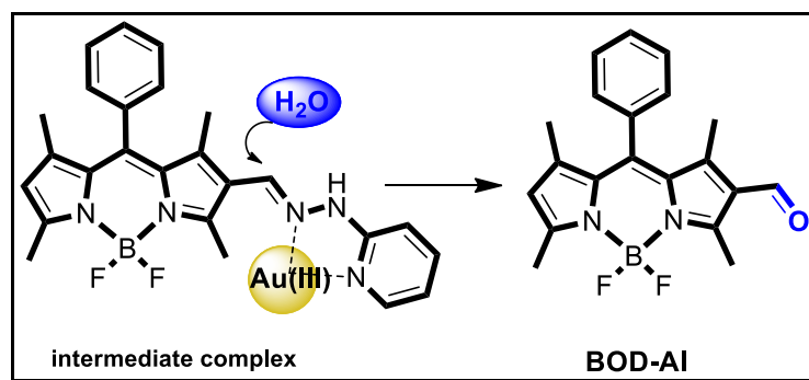
Figure 2.21. Gold mediated hydrolysis of BOD-1
