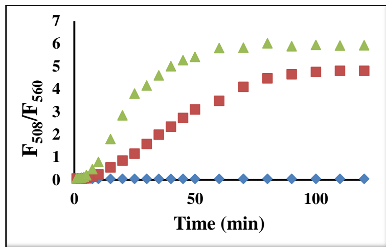
Figure 3.48. Reaction time profiles of BOD-4 (5 \mu\text{M} ) in the absence ( \blacklozenge ) or presence of \text{Hg}^{2+} [5 ( \blacksquare ), 10( \blacktriangle ) \mu\text{M} ]. The fluorescence intensities were continuously monitored at time intervals in 10 mM HEPES, pH 7.0/ \text{CH}_3\text{CN} (v/v, 6:4) ( \lambda_{\text{exc}}=460 nm at 25 ^\circ\text{C} ).
