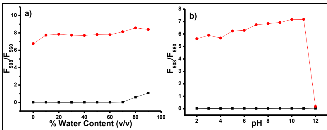
Figure 3.45. a) Effect of fraction of water (pH 7.0 HEPES/CH 3 CN) and b) Effect of pH (HEPES/CH 3 CN, (v/v, 6:4)) on the interaction of BOD-4 (10 \mu M) (black line) with Hg 2+ (20 \mu M, 2 equiv.) (red line) in 0.1M potassium phosphate buffer, ( \lambda_{\text{ex}} : 460 nm at 25 °C).
