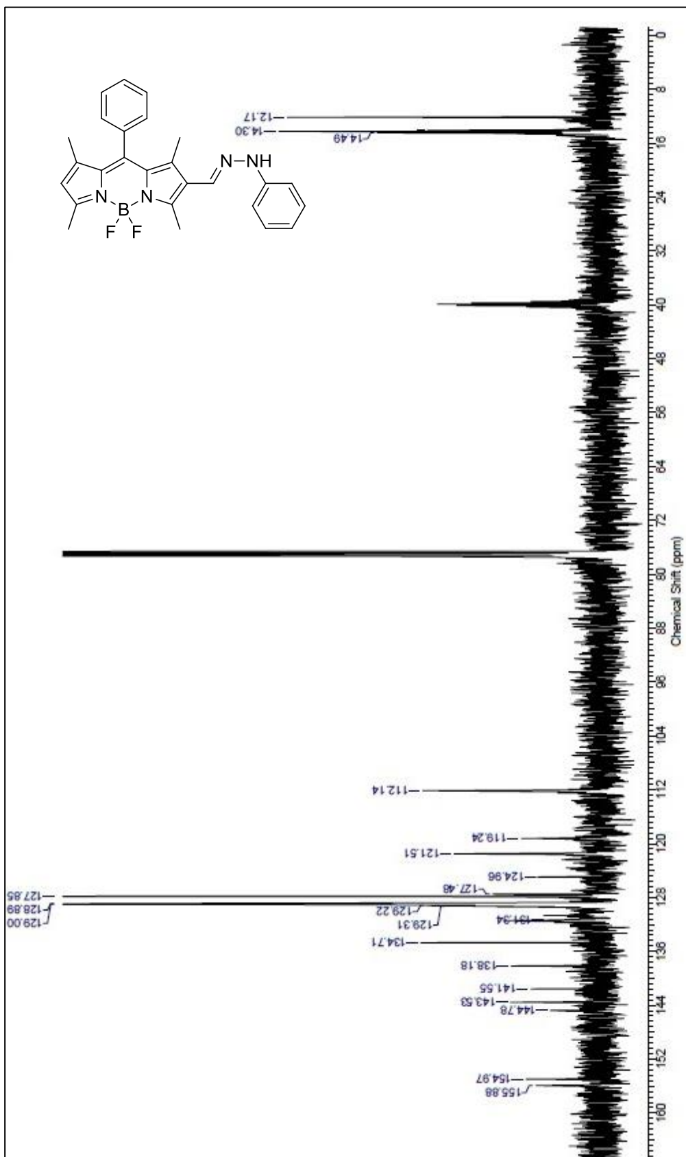
Figure A.8. 13 C NMR of (E)-5,5-difluoro-1,3,7,9-tetramethyl-10-phenyl-8-((2-phenylhydrazono)methyl)-5H-dipyrrolo[1,2-c:2,1'-f][1,3,2]diazaborin-4-ium-5-uide
