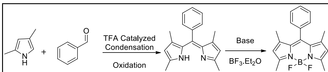
Figure 1.13. Acid catalyzed condensation of aromatic aldehydes with pyrroles (Source: Boens et al., 2012)
