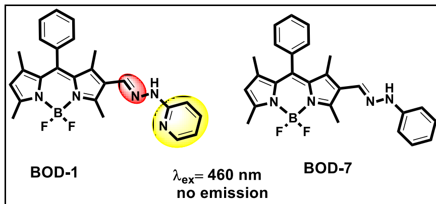
Figure 2.15. Structure of BOD-1 and control probe BOD-7
