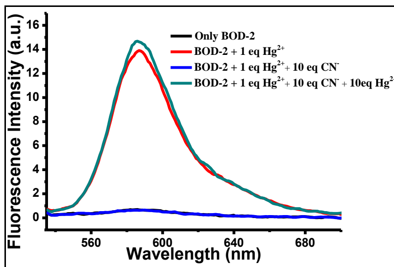
Figure 3.29. Fluorescence intensity changes of BOD-2 ( 5 \mu\text{M} ) in 1:1 \text{CH}_3\text{CN/HEPES} buffer at \text{pH} = 7.0 at \lambda_{\text{max}} : 585 after addition of 1 equiv. \text{Hg}^{2+} , 1 equiv. \text{Hg}^{2+} + 10 equiv. \text{CN}^- and 1 equiv. \text{Hg}^{2+} + 10 equiv. \text{CN}^- + 10 equiv. \text{Hg}^{2+} respectively.
