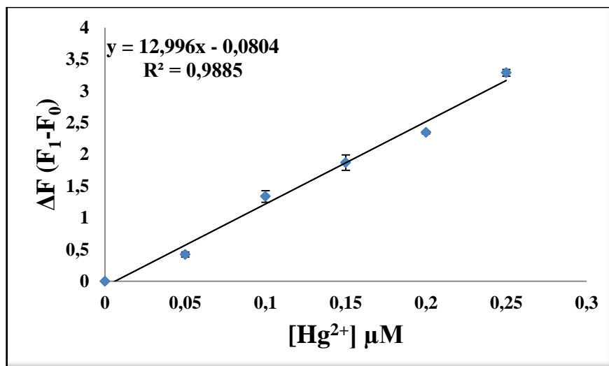
Figure 3.26. Fluorescence changes of probe 1 (5.0 μM) upon addition of Hg 2+ (0.05 to 0.3 μM, 0.01 to 0.05 equiv.)
