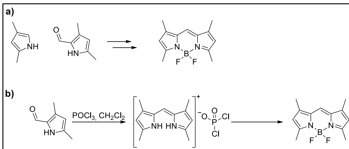
Figure 1.16. a) Conventional synthesis of tetramethyl-BODIPY and b) the new approach described (Source: Wu and Burgess, 2008)
