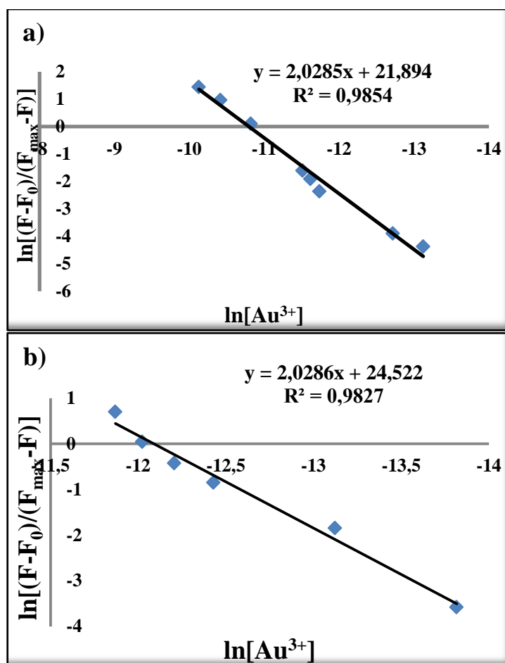
Figure 2.72. Binding ability of BOD-6 to \text{Au}^{3+} a) in EtOH in 0.1M potassium phosphate buffer, pH 7.0/EtOH (v/v, 1:1) b) in dichloroethane ( \lambda_{\text{exc}}=500 \text{ nm} , \lambda_{\text{em}}=577 \text{ nm} at 25 \text{ }^\circ\text{C} ).
