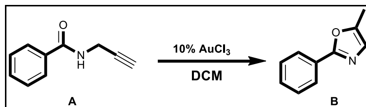
Figure 2.78. AuCl 3 catalyzed cyclization reaction of propargyl amide
