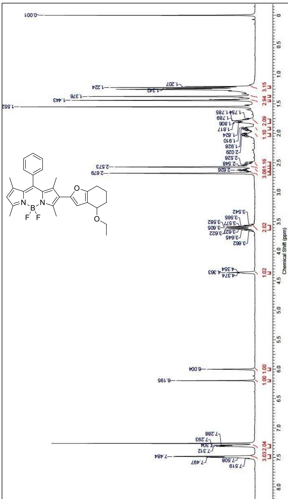
Figure A.23. 1 H NMR of (R)-8-(4-ethoxy-4,5,6,7-tetrahydrobenzofuran-2-yl)-5,5-difluoro-1,3,7,9-tetramethyl-10-phenyl-5H-dipyrrolo[1,2-c:2',1'-f][1,3,2]diazaborinin-4-ium-5-uide
