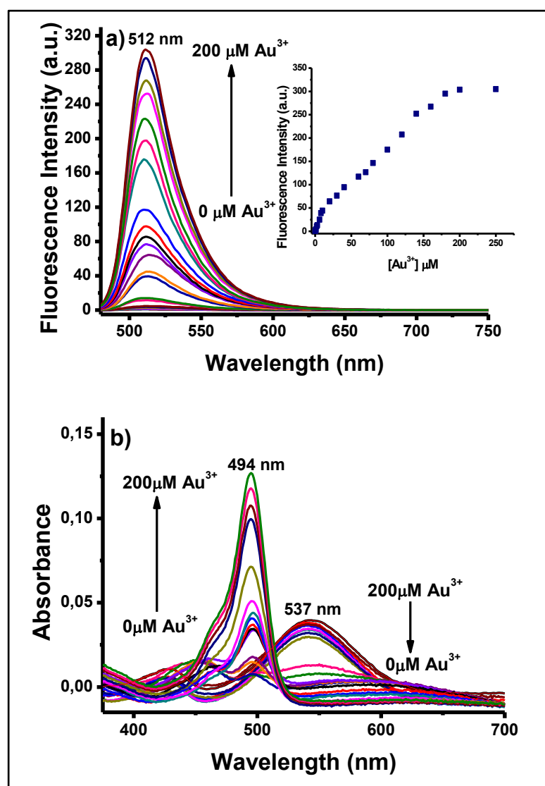
Figure 2.17. a) Fluorescence and b) Absorbance spectra of BOD-1 (10 \mu\text{M} ) in the presence of increasing amount of \text{Au}^{3+} (0-200 \mu\text{M} ) 0.1 M phosphate buffer/EtOH (pH 7.0, v/v, 1:1). Inset: Calibration curve. ( \lambda_{\text{ex}} : 460 nm at 25 ^{\circ}\text{C} ).
