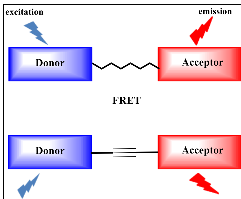
Figure 1.47. Schematic representation of FRET and TBET systems (Source: Das et al., 2013; Lee et al., 2015)
