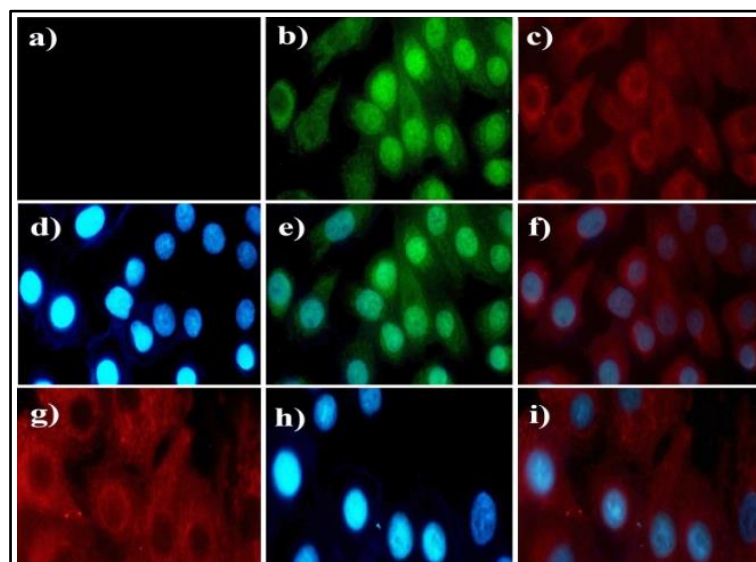
Figure 2.33. a) Fluorescence image of A549 cells treated with only BOD-2 ( 5\mu\text{M} ); b) Image of cells treated with \text{Au}^{3+} ( 5\mu\text{M} ) and probe ( 5\mu\text{M} ) ( \lambda_{\text{ex}}=470\text{ nm} ); c) Cells treated with \text{Au}^{3+} ( 5\mu\text{M} ) and probe ( 5\mu\text{M} ) ( \lambda_{\text{ex}}=525\text{ nm} ); d and h) Cells treated with DAPI for 15 min (control); d) Merged image of frame b and d; f) merged image of frame c and d; g) Cells treated with \text{Hg}^{2+} ( 5\mu\text{M} ) and probe ( 5\mu\text{M} ) ( \lambda_{\text{ex}}=525\text{ nm} ); i) merged image of frame g and h.
