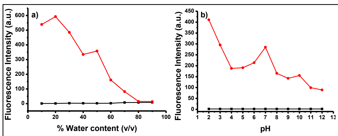
Figure 2.16. a) Effect of fraction of water (in 0.1M potassium phosphate buffer pH 7.0/EtOH) and b) Effect of pH (in 0.1M potassium phosphate buffer pH/EtOH (v/v, 1:1)) on the interaction of BOD-1 (10 \mu\text{M} ) (black line) with \text{Au}^{3+} (200 \mu\text{M} , 20 equiv.) (red line), ( \lambda_{\text{ex}} : 460 nm, \lambda_{\text{em}} = 512 nm at 25 ^{\circ}\text{C} ).
