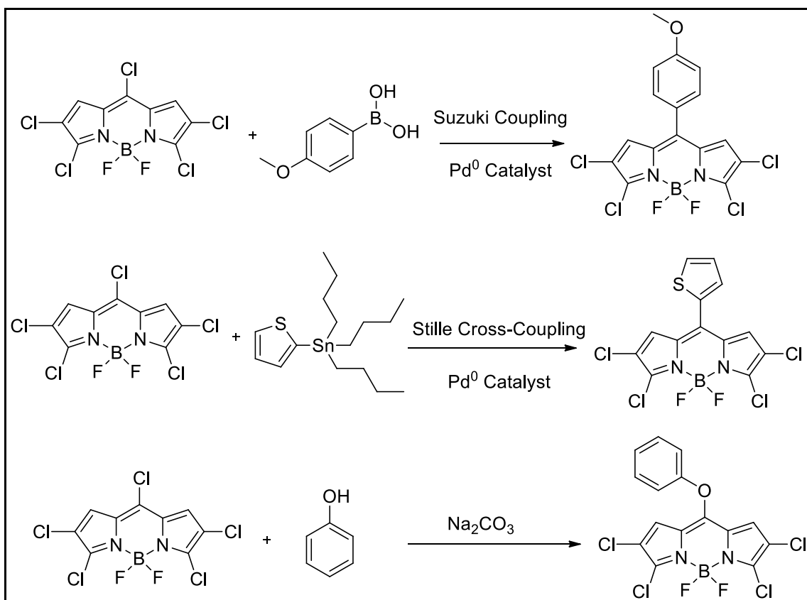
Figure 1.22. Examples of reactions of meso halogenated BODIPYs (Source: Zhao et al., 2015)
