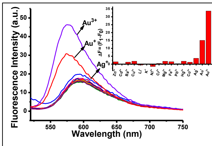
Figure 2.69. Fluorescence intensities of BOD-6 ( 10.0\mu\text{M} ), BOD-6 ( 10.0\mu\text{M} ) + \text{Au}^{3+} ( 60\mu\text{M} , 6 equiv.), BOD-6 ( 10.0\mu\text{M} ) + other ions ( 250\mu\text{M} , 25 equiv.) in 0.1\text{M} potassium phosphate buffer, pH 7.0/EtOH (v/v, 1:1) ( \lambda_{\text{ex}} :500 nm, at 25^\circ\text{C} ). Inset: Bar graph notation.
