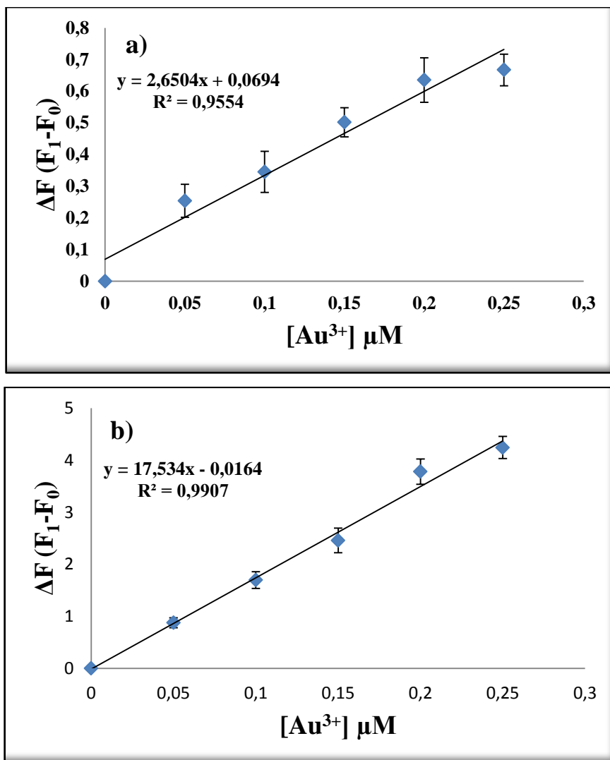
Figure 2.28. Detection limit of BOD-2 towards addition of Au^{3+} ions a) \lambda_{em}=506 nm and b) \lambda_{em}=585 nm
