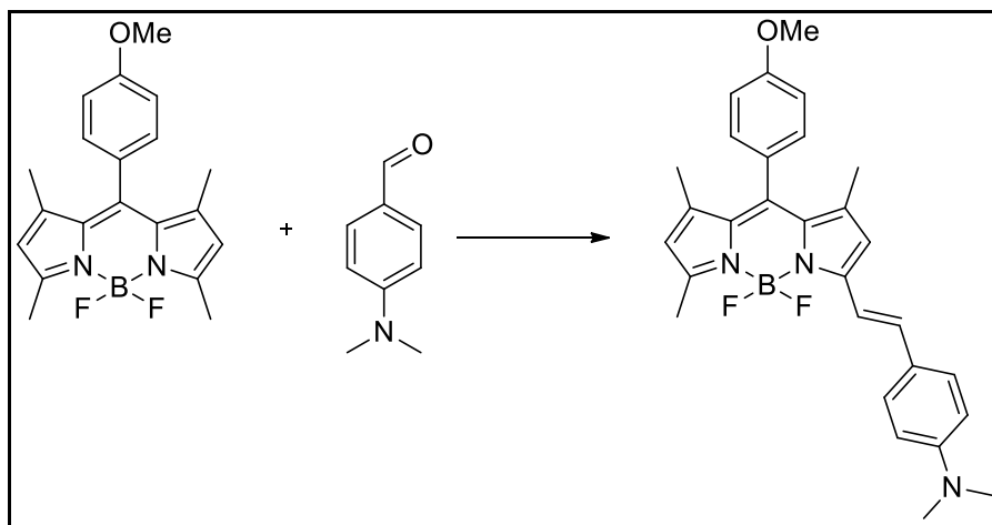
Figure 1.27. 3-monostyryl derivative of BODIPY (Source: Haugland and Kang, 1988)
