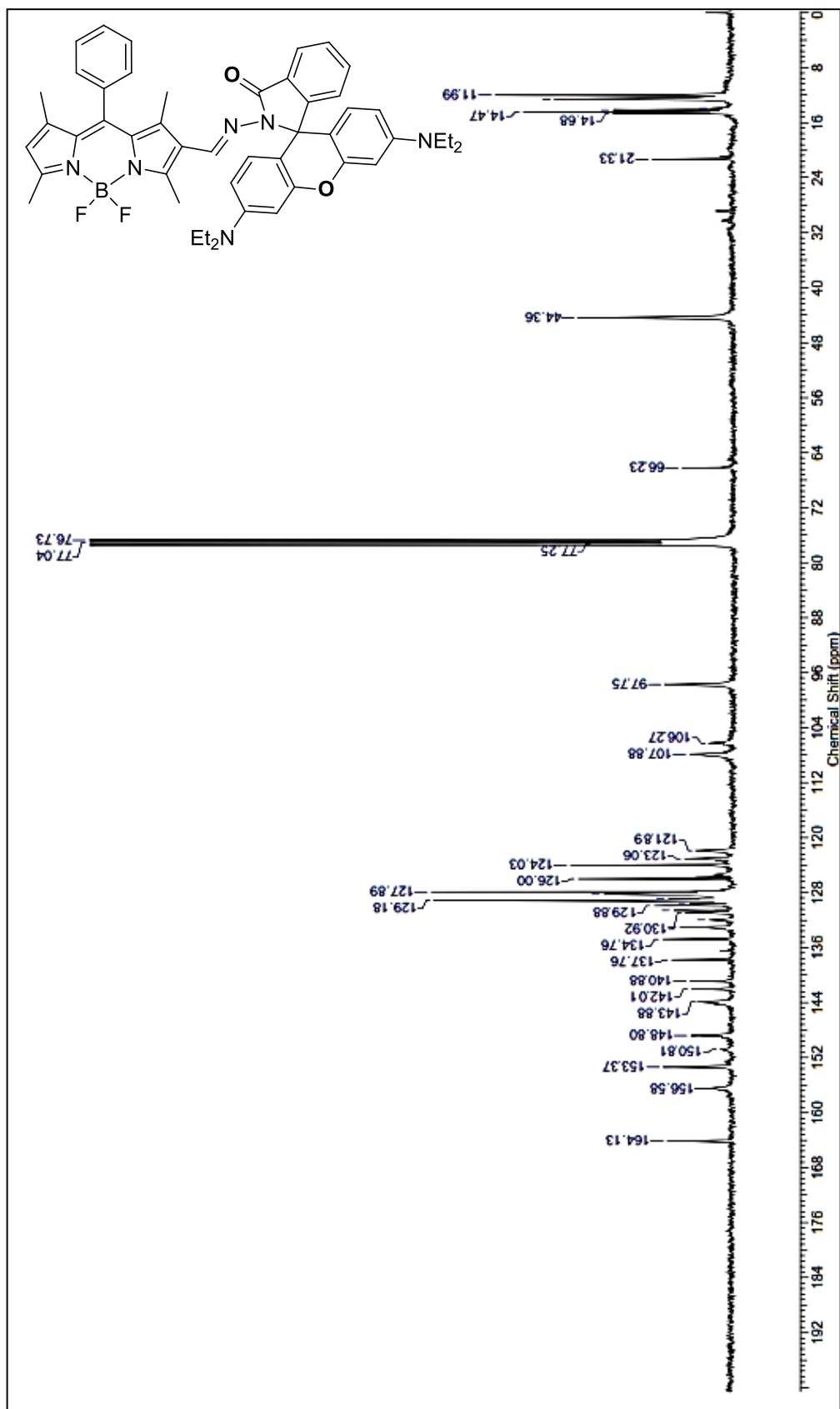
Figure A.12. ^{13}\text{C} NMR of (E)-8-(((3',6'-bis(diethylamino)-3-oxospiro[isoindoline-1,9'-xanthen]-2-yl)imino)methyl)-5,5-difluoro-1,3,7,9-tetramethyl-10-phenyl-5H-dipyrrolo[1,2-c:2',1'-f][1,3,2]diazaborin-4-ium-5-uide
