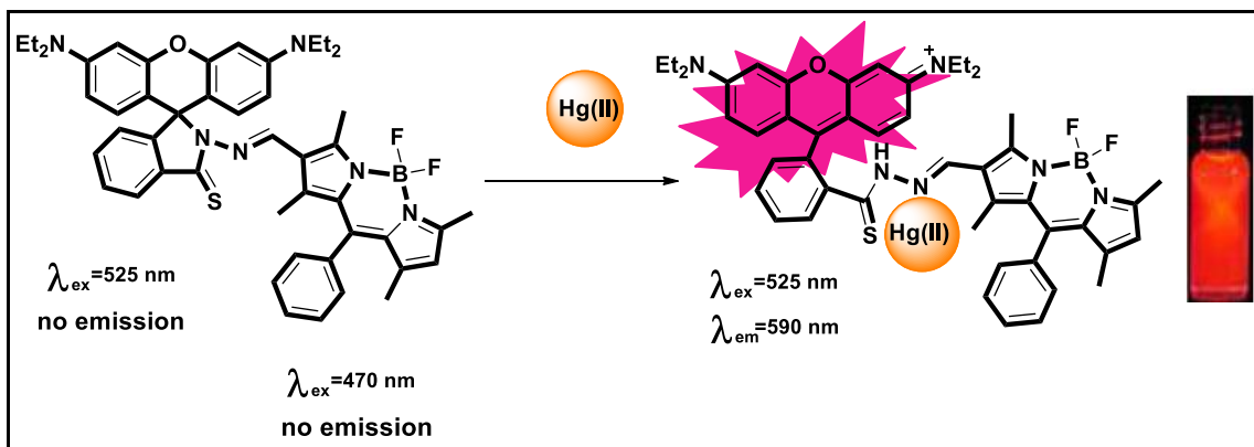
Figure 3.31. Proposed coordination of mercury to Rhodamine-BODIPY scaffold.
