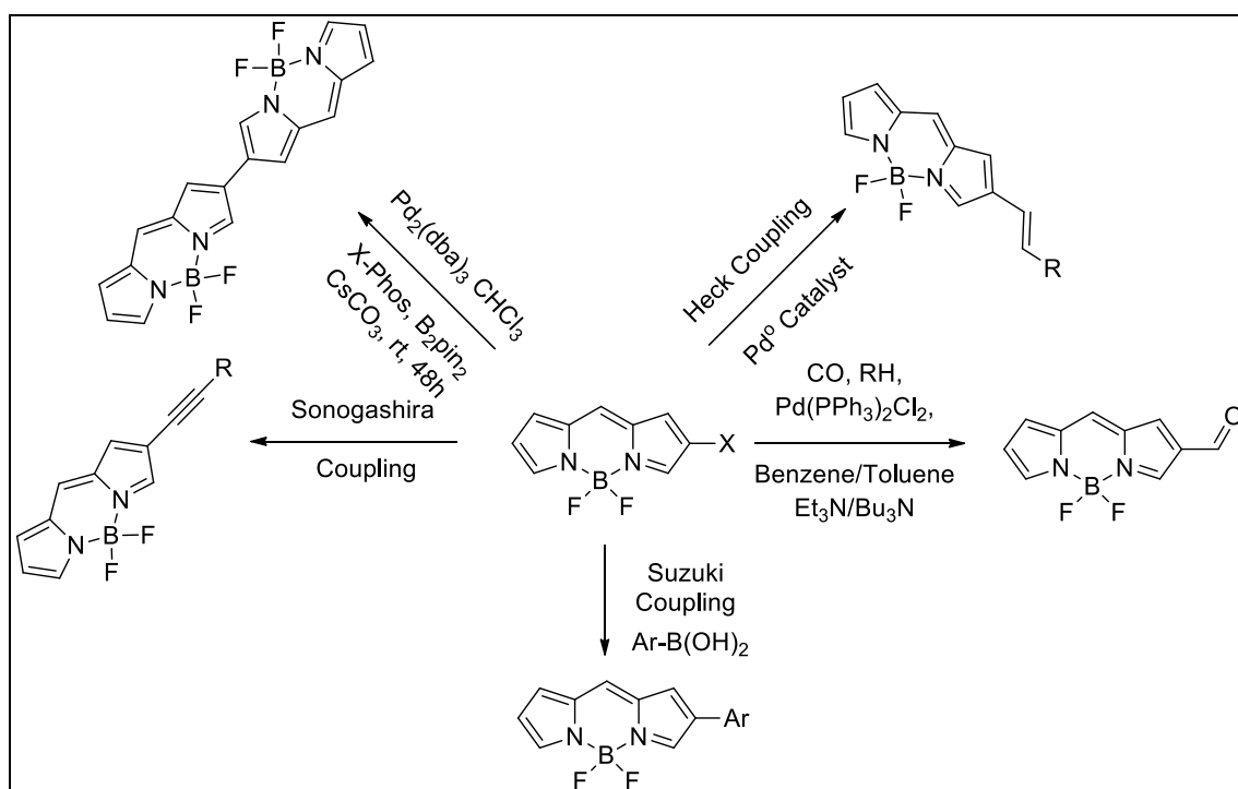
Figure 1.32. Reactions of BODIPY core halogenated from 2,6- positions (Source: Lakshmi et al., 2015)
