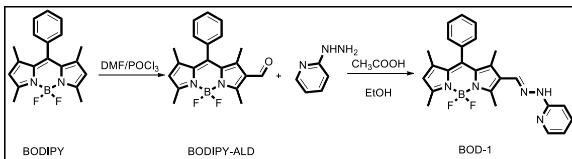
Figure 2.14. Synthetic route to BOD-1
