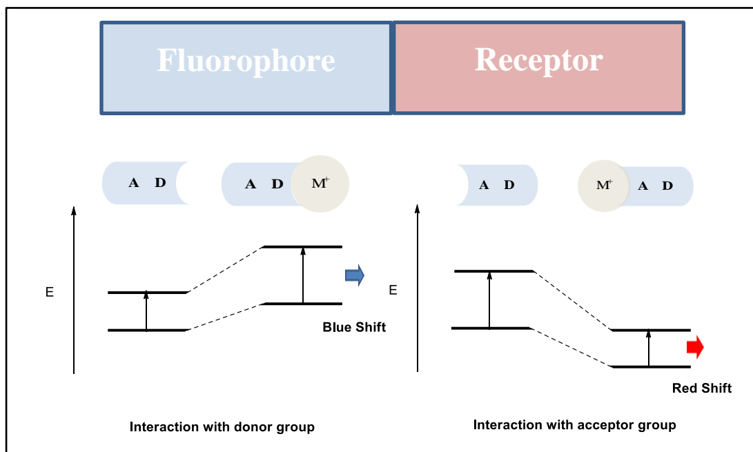
Figure 1.45. Intramolecular charge transfer mechanism (Source: Das et al., 2013; Lee et al., 2015)
