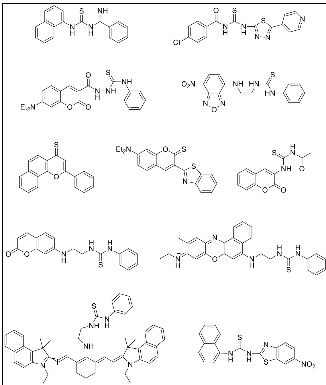
Figure 3.15. Fluorescent sensors for \text{Hg}^{2+} working via desulfuration reaction (Source: Yang et al., 2013)
