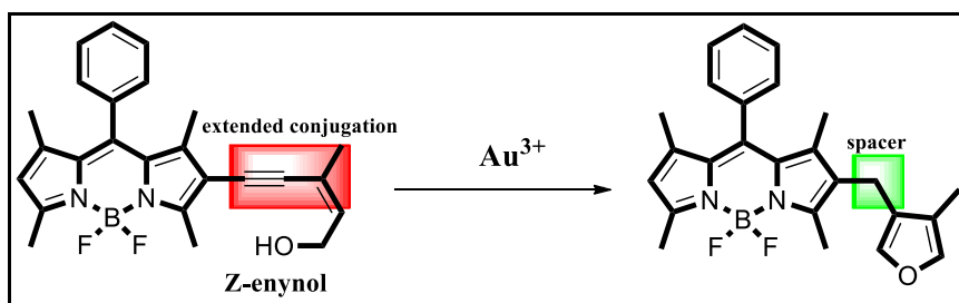
Figure 2.53. The rationale of ratiometric sensing
