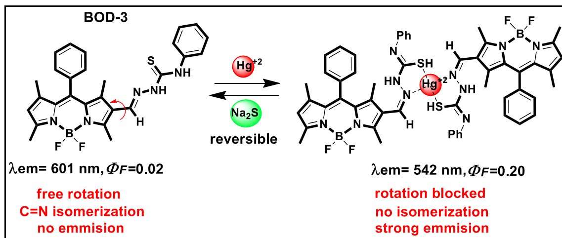
Figure 3.37. Proposed reversible binding of \text{Hg}^{2+} to BOD-3
