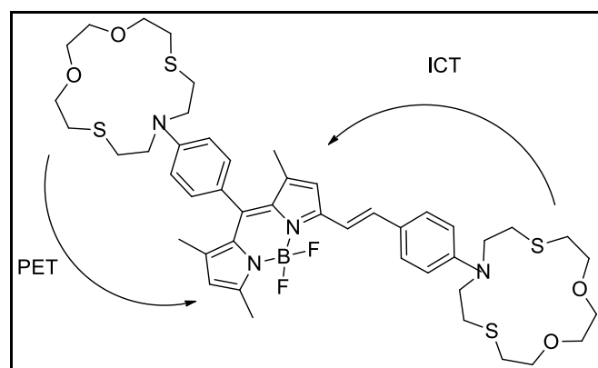
Figure 3.4. BODIPY based chemosensor for Hg 2+ (Source: Yuan et al., 2007)
