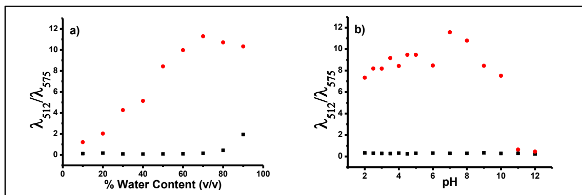
Figure 2.55. a) Effect of fraction of water (in 0.1M potassium phosphate buffer pH 7.0/EtOH) and b) Effect of pH (in 0.1M potassium phosphate buffer pH/EtOH (v/v, 7:3)) on the interaction of BOD-5 (10 \mu\text{M} ) (black line) with \text{Au}^{3+} (200 \mu\text{M} , 20 equiv.) (red line), ( \lambda_{\text{ex}} : 460 nm, emission wavelengths: \lambda_{512}/\lambda_{575} at 25 ^{\circ}\text{C} ).
