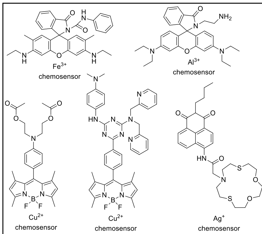
Figure 1.41. Examples of complexation based fluorescent sensors (Source: Joung and Joon, 2012; Das et al., 2013; Wu et al., 2015)
