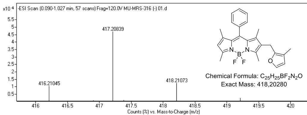
Figure B.11. Mass Spectrum of (7)-BODIPY-FUR 5,5-difluoro-1,3,7,9-tetramethyl-8-((3-methylfuran-2-yl)methyl)-10-phenyl-5H-dipyrrolo[1,2-c:2',1'-f][1,3,2]diazaborinin-4-ium-5-uide
