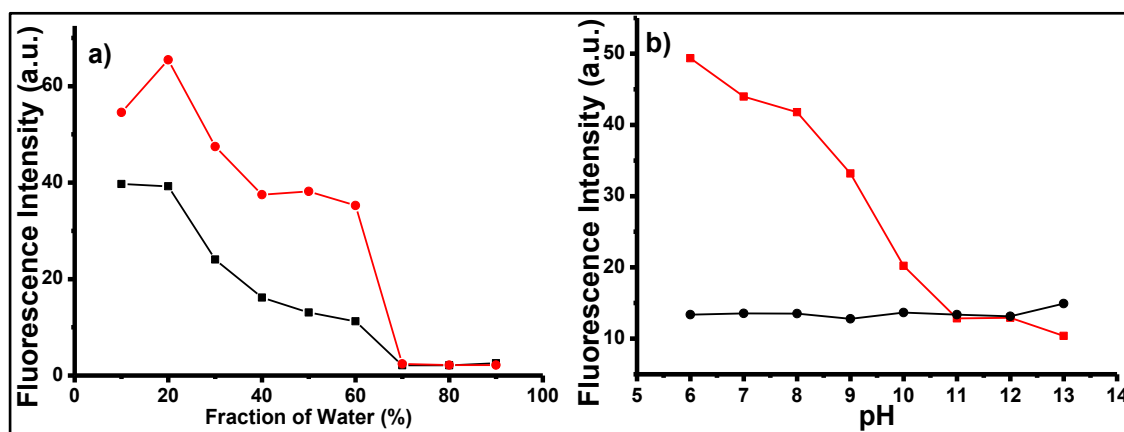
Figure 2.66. a) Effect of fraction of water (in 0.1M potassium phosphate buffer pH 7.0/EtOH) and b) Effect of pH (in 0.1M potassium phosphate buffer pH/EtOH (v/v, 1:1)) on the interaction of BOD-6 (10 \mu\text{M} ) (black line) with \text{Au}^{3+} (200 \mu\text{M} , 20 equiv.) (red line), ( \lambda_{\text{ex}} : 460 nm, \lambda_{\text{em}} = 577 at 25 °C).
