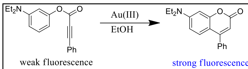
Figure 2.4. Reaction based fluorescent sensor for gold(III) ion (Source: Do et al., 2010)
