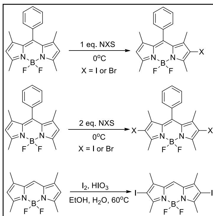
Figure 1.31. Halogenation of BODIPY compound from 2,6- position. (Source: Çakmak and Akkaya, 2009; Yogo et al., 2005)
