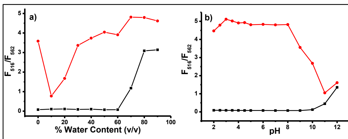
Figure 3.40. a) Effect of fraction of water (pH 7.0/EtOH ) and b) Effect of pH (pH/EtOH (v/v, 6:4)) on the interaction of BOD-4 (10 \mu\text{M} ) (black line) with \text{Hg}^{2+} (200 \mu\text{M} , 20 equiv.) (red line) in 0.1M potassium phosphate buffer, ( \lambda_{\text{ex}} : 460 nm at 25 ^{\circ}\text{C} ).
