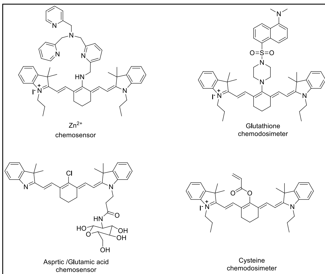
Figure 1.10. Cyanine based chemosensors and chemodosimeters (Source: Guo et al., 2012; Yin et al., 2015; Zhao et al., 2014)
