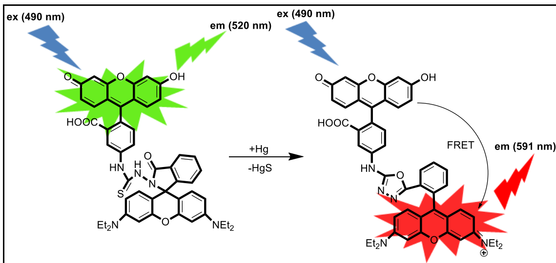
Figure 3.13. A FRET probe based on fluorescein-rhodamine scaffold (Source: Shang et al., 2008)
