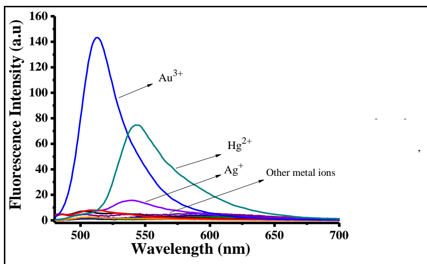
Figure 2.39. Fluorescence intensities of BOD-3 (10 \mu\text{M} ) in 0.1 M phosphate buffer/EtOH (pH = 7.0, v/v, 1:4) in the presence of 20.0 equiv. (200 \mu\text{M} ) of the cations of interest: BOD-3 only, \text{Au}^+ , \text{Ba}^{2+} , \text{Ca}^{2+} , \text{Cd}^{2+} , \text{Cr}^{3+} , \text{Cu}^{2+} , \text{Fe}^{3+} , \text{F}^- , \text{I}^- , \text{Li}^+ , \text{Mg}^{2+} , \text{Ni}^{2+} , \text{Pb}^{2+} , \text{Zn}^{2+} ( \lambda_{\text{ex}} = 460 nm, \lambda_{\text{em}} = 512 nm).
