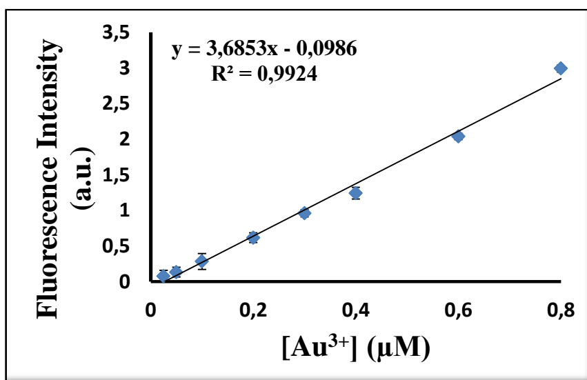
Figure 2.18. Fluorescence changes of BOD-1 (10.0 \mu\text{M} ) upon addition of \text{Au}^{3+} (0,025 to 0,8 \mu\text{M} , 0. 025 to 0.08 equiv.) in 0.1 M potassium phosphate buffer, pH 7.0/EtOH (v/v, 1:1) ( \lambda_{\text{ex}} : 460 nm, \lambda_{\text{em}} = 512 nm at 25 °C).
