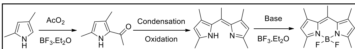
Figure 1.11. Serendipitous discovery of BODIPY (Source: Treibs and Kreuzer, 1968)
