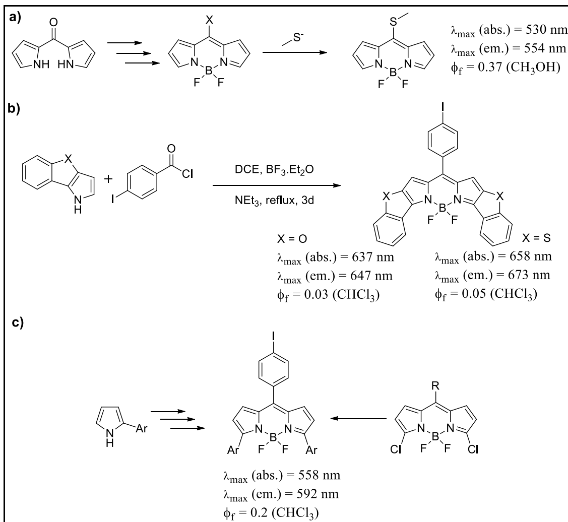
Figure 1.15. Synthetic pathways of BODIPY derivatives by using a) post-modification, b) premodification, and c) both methods. (Source: Ni and Wu, 2014; Boens et al., 2015)
