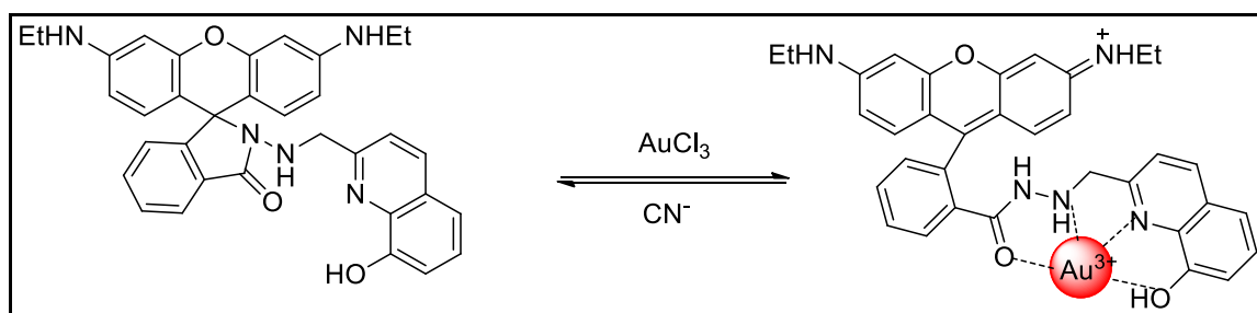
Figure 2.10. The first example of reversible \text{Au}^{3+} ions sensor (Source: Wang et al., 2011)
