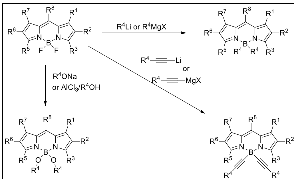
Figure 1.36. Reactions of BODIPY core from boron center (Source: Ulrich et al., 2008)
