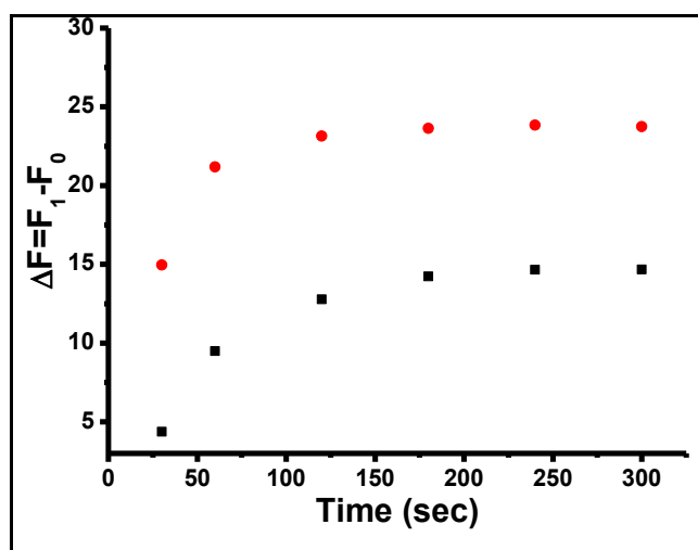
Figure 2.68. Reaction time profiles of BOD-6 (10.0 \mu M) in the presence of Au 3+ [30 (■) and 60 (●) \mu M.]. The fluorescence intensities at 577 nm were continuously monitored at time intervals in 0.1 M phosphate buffer/EtOH (pH 7.0, v/v, 1:1) ( \lambda_{\text{ex}} : 500 nm, \lambda_{\text{em}} = 577 nm at 25 °C).
