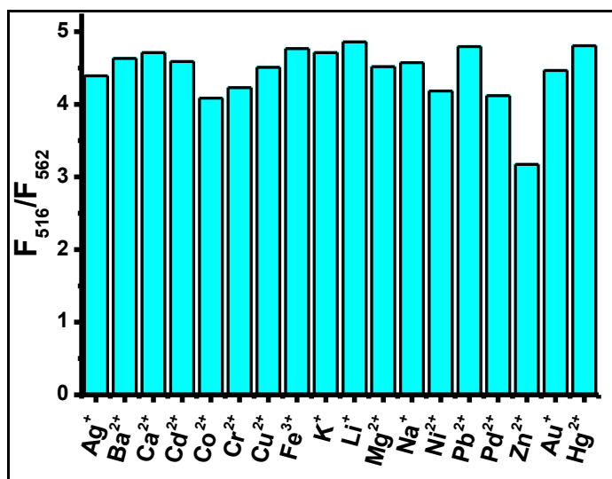
Figure 2.51. Fluorescence intensities of BOD-4 (5 \mu\text{M} ) in the presence of \text{Au}^{3+} (10 \mu\text{M} , 2 equiv.) and 10 equiv. of other metal ions in 0.1 M phosphate buffer/EtOH (pH 7.0, v/v, 6:4) ( \lambda_{\text{exc}}=460 nm at 25 ^{\circ}\text{C} )
