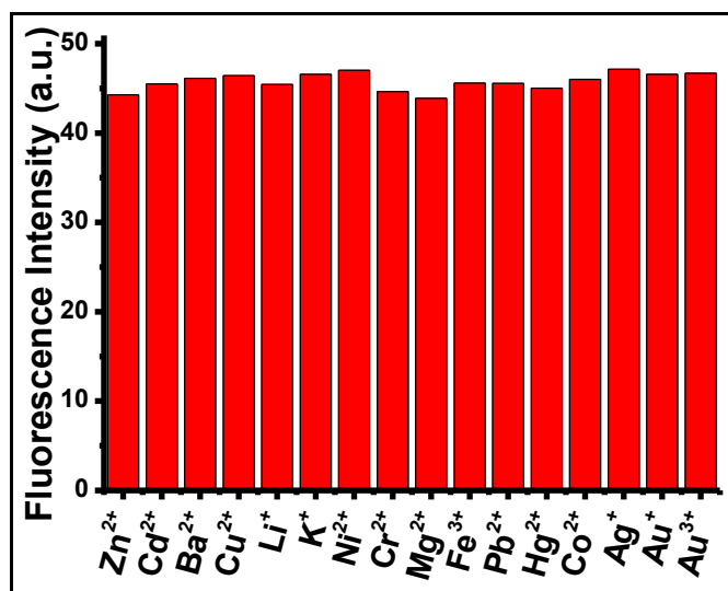
Figure 2.70. Fluorescence intensities of BOD-6 (10 \mu M) in the presence of Au 3+ (6 equiv.) and 10 equiv. of other metal ions in 0.1 M phosphate buffer/EtOH (pH 7.0, v/v, 1:1) ( \lambda_{\text{exc}} =500 nm, \lambda_{\text{em}} = 577 nm at 25 °C).
