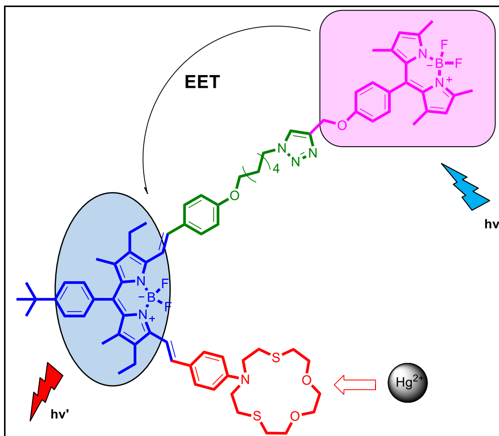
Figure 3.5. Selective \text{Hg}^{2+} sensing by coupling the internal charge transfer to excitation energy transfer (Source: Atilgan et al., 2010)
