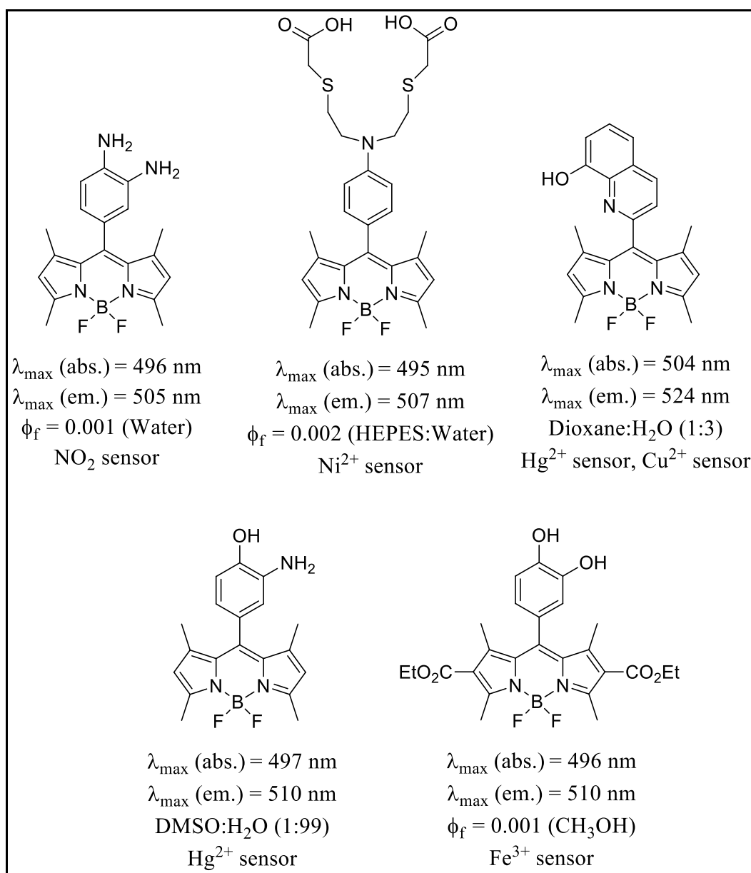
Figure 1.20. BODIPY based sensors synthesized from aldehyde derivative (Source: Boens et al., 2012)
