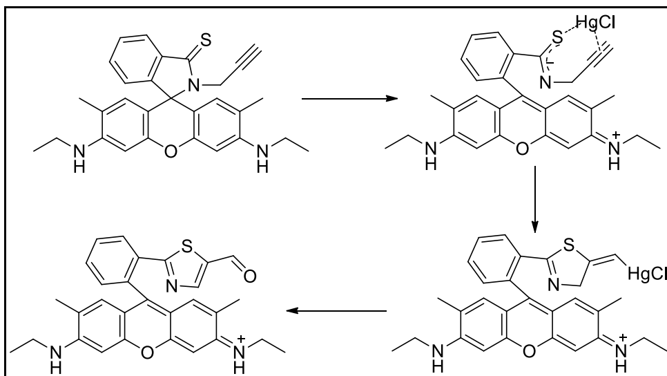
Figure 3.22. The proposed reaction mechanism of Rhodamine based probe with \text{Hg}^{2+} (Source: Lin et al., 2010)
