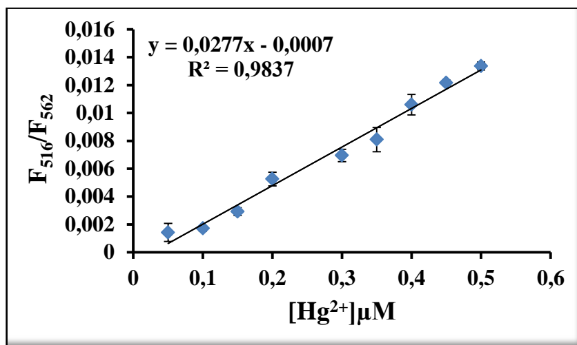
Figure 3.42. Fluorescence changes of BOD-4 (5.0 \mu\text{M} ) upon addition of \text{Hg}^{2+} (0.05 to 0.5 \mu\text{M} , 0.01 to 0.1 equiv.) in 0.1M potassium phosphate buffer, pH 7.0/EtOH (v/v, 6:4) ( \lambda_{\text{ex}} : 460 nm, at 25 °C).
