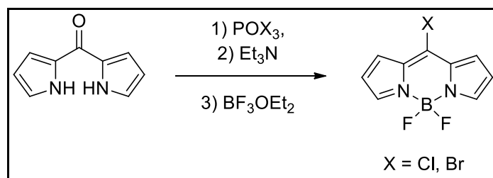
Figure 1.21. Synthesis of meso -halogenated BODIPY (Source: Leen et al., 2012)
