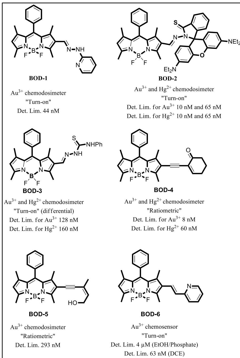
Figure 5.1. Summary of synthesized probe molecules
