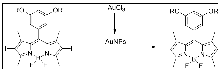
Figure 2.8. Detection of \text{Au}^{3+} ions via C-I bond cleavage (Source: Park et al., 2012)
