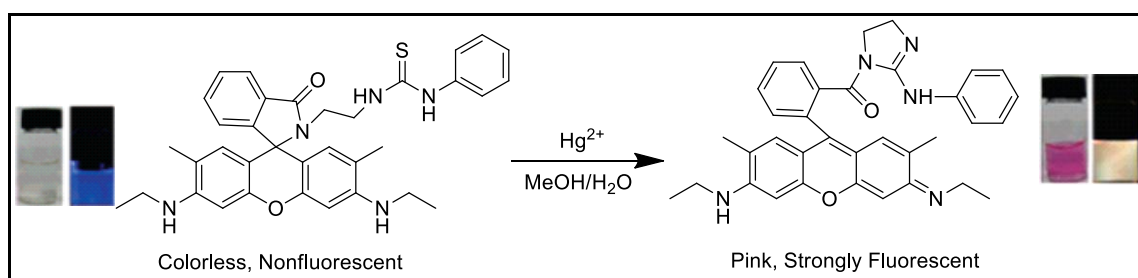
Figure 3.12. Response of the developed probe to the addition of \text{Hg}^{2+} ions (Source: Wu et al., 2007)
