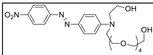
Figure 3.2. Chromogenic sensor for \text{Hg}^{2+} ions (Source: Sancenon et al., 2001)
