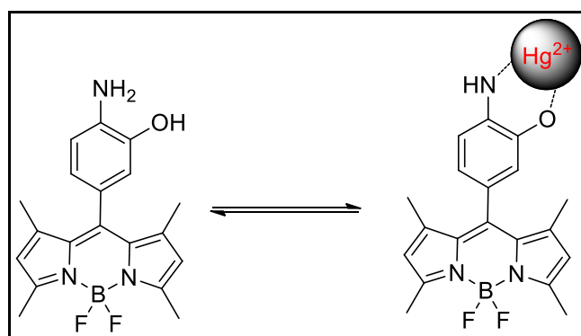
Figure 3.9. A reversible molecular sensor for \text{Hg}^{2+} (Source: Fan et al., 2012)
