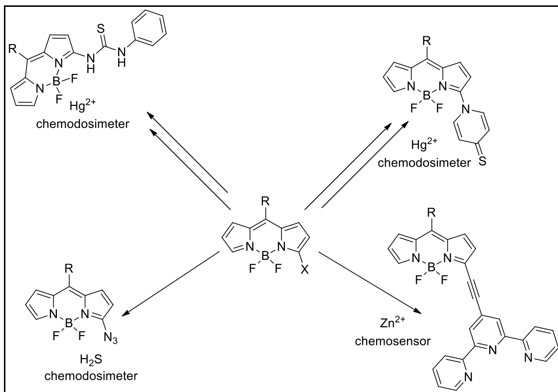
Figure 1.25. BODIPY based sensors functionalized from 3- position (Source: Lakshmi et al., 2015)
