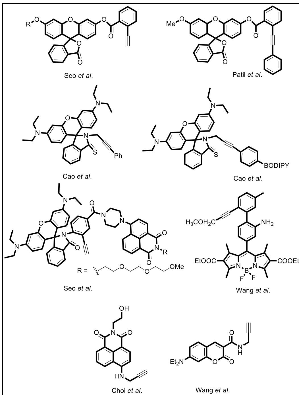
Figure 2.5. Gold ion sensor based on alkyne moiety. (Source: Singha et al. , 2015)
