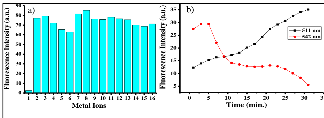
Figure 3.39 a) Fluorescence intensities of BOD-3 (10 \mu\text{M} ) in 0.1 M phosphate buffer/EtOH (pH = 7.0, v/v, 1:4) in the presence of 20.0 equiv. (200 \mu\text{M} ) of the cations interest : 1, BOD-3 only; 2, \text{Hg}^{2+} ; 3, \text{Au}^+ ; 4, \text{Ba}^{2+} ; 5, \text{Ca}^{2+} ; 6, \text{Cd}^{3+} ; 7, \text{Cr}^{2+} ; 8, \text{Cu}^{2+} ; 9, \text{Fe}^{2+} ; 10, \text{I}^- ; 11, \text{Mg}^{2+} ; 12, \text{Ni}^{2+} ; 13, \text{Pb}^{2+} ; 14, \text{Zn}^{2+} ; 15, \text{Ag}^+ ; 16, \text{F}^- . b) Selectivity profile of BOD-3 towards \text{Au}^{3+} and \text{Hg}^{2+} ions ( \lambda_{\text{ex}} = 460 \text{ nm} , \lambda_{\text{em}} = 542 \text{ nm} and 511 nm).
