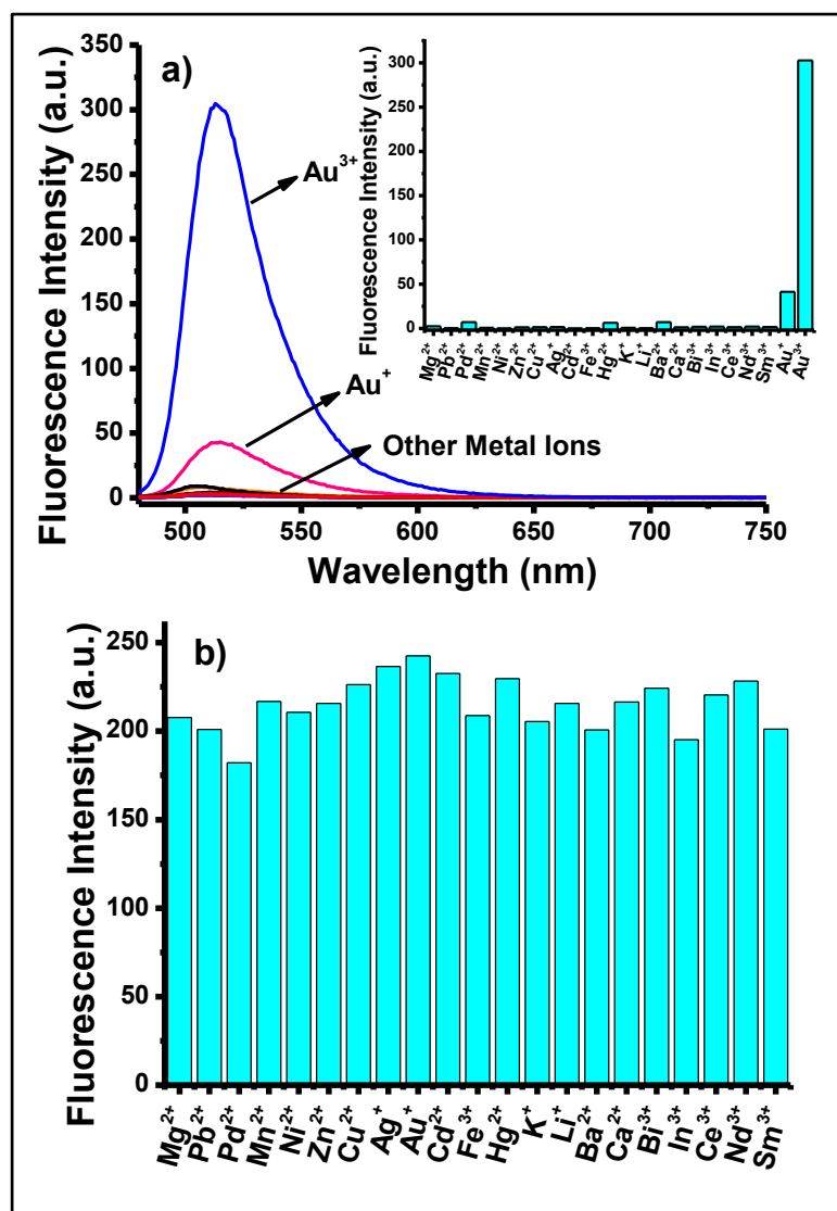
Figure 2.20. Fluorescence of a) selectivity b) competition experiments of BOD-1 (10 \mu\text{M} ) + \text{Au}^{3+} (200 \mu\text{M} , 20 equiv.), BOD-1 (10 \mu\text{M} ) + other metal ions (200 \mu\text{M} , 20 equiv.) in 0.1M potassium phosphate buffer, pH 7.0/EtOH (v/v, 1:1) ( \lambda_{\text{ex}} : 460 nm, at 25 ^{\circ}\text{C} ). Inset: Bar graph notation.
