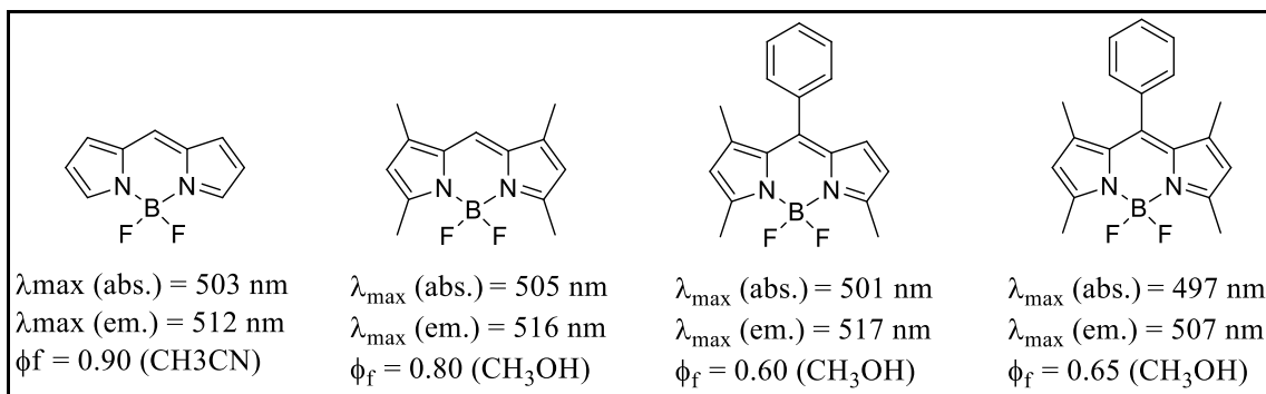
Figure 1.17. Influence of alkyl and meso aryl substituents on the spectroscopic properties (Source: Ni and Wu, 2014)
