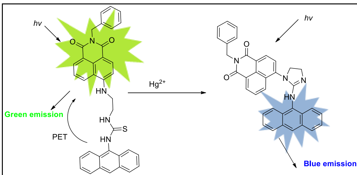
Figure 3.14. A FRET probe based on naphthalimide-anthracene scaffold. (Source: Srivastava et al., 2013)
