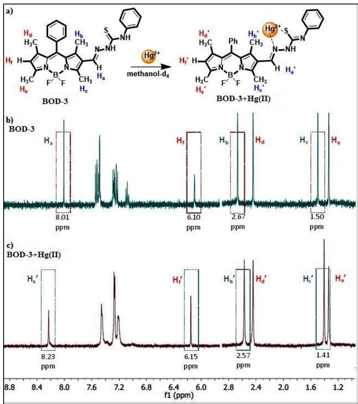
Figure 3.38. a) Proposed coordination mechanism of \text{Hg}^{2+} to BOD-3 . b) ^1\text{H-NMR} of BOD-3 in methanol- \text{d}_4 . c) ^1\text{H-NMR} of BOD-3 + \text{Hg}^{2+} (1 equiv.) in methanol- \text{d}_4 .
