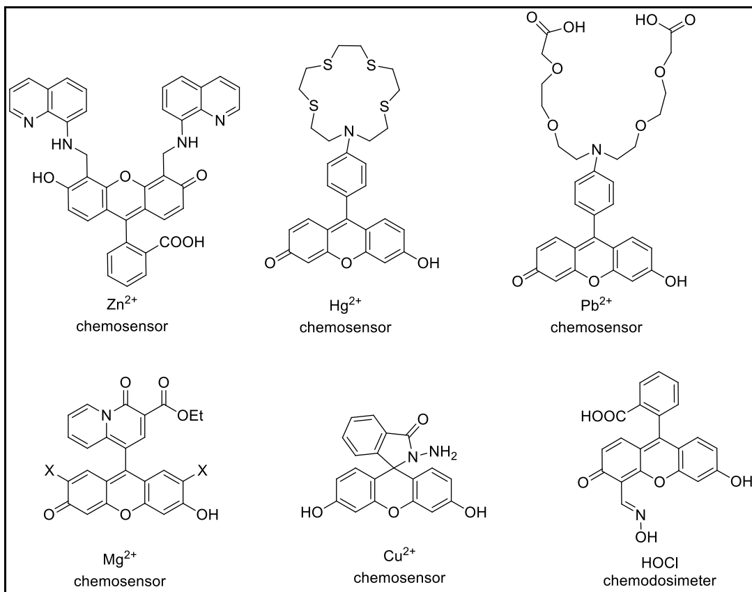
Figure 1.2. Fluorescein based sensors (Source: Li et al., 2013)
