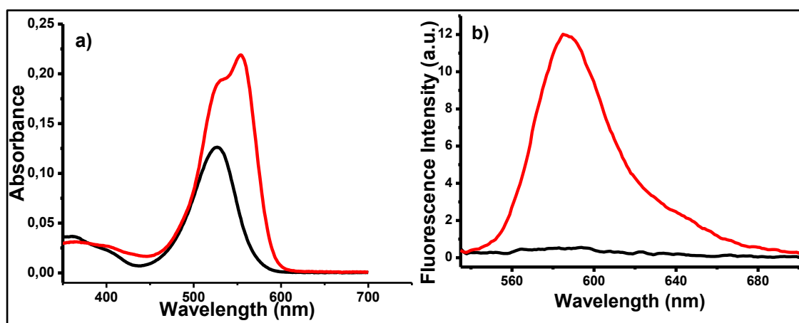
Figure 3.24. a) Absorption and b) Emission spectra of BOD-2 (5 \mu\text{M} ) and \text{Hg}^{2+} (1.0 equiv.) in 1:1 \text{CH}_3\text{CN}/\text{HEPES} buffer at pH = 7.0; ( \lambda_{\text{ex}} : 525 nm, at 25 °C).
