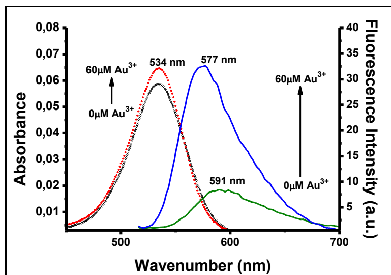
Figure 2.67. Absorbance spectra of BOD-6 (10 \mu M) in the absence (black dot-line) and presence (red dot-line) of 6 equiv. (60 \mu M) of Au 3+ and fluorescence spectra of BOD-6 (10 \mu M) in the absence (green line) and presence (blue line) of 6 equiv. (60 \mu M) of Au 3+ in 0.1 M phosphate buffer/EtOH (pH 7.0, v/v, 1:1).
