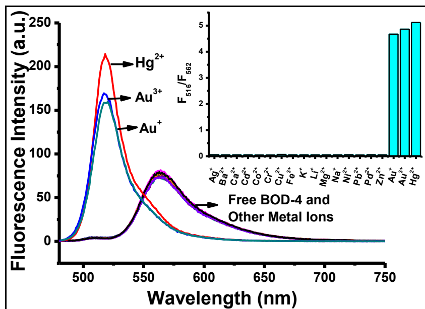
Figure 2.50. Fluorescence intensities of BOD-4 (5 \mu\text{M} ), BOD-4 (5 \mu\text{M} ) + \text{Au}^{3+} (25 \mu\text{M} , 5 equiv.), BOD-4 (5 \mu\text{M} ) + other metal ions (50 \mu\text{M} , 10 equiv.) in 0.1M potassium phosphate buffer, pH 7.0/EtOH (v/v, 6:4) ( \lambda_{\text{ex}} : 460 nm, at 25 ^{\circ}\text{C} ). Inset: Bar graph notation.
