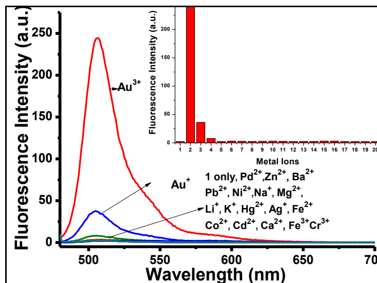
Figure 2.29. Fluorescence intensities of BOD-2 (5 \mu\text{M} ) in 1:1 \text{CH}_3\text{CN} /HEPES buffer at \text{pH} = 7.0 at \lambda_{\text{max}} : 505 nm in the presence of 10.0 equivalent of the cations interest.
