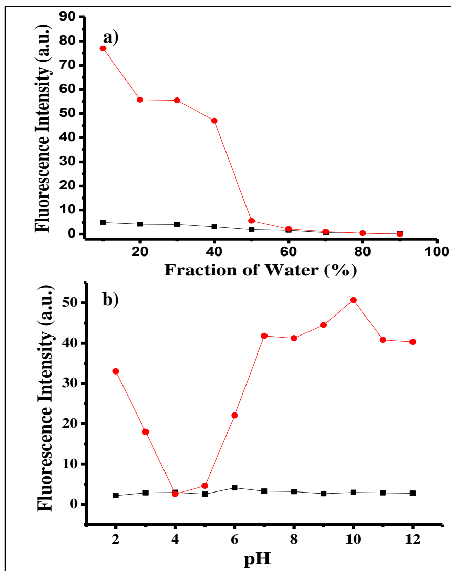
Figure 3.33. a) Effect of fraction of water (pH 7.0/EtOH ) and b) Effect of pH (pH/EtOH (v/v, 1:4)) on the interaction of BOD-3 (10 \mu\text{M} ) (black line) with \text{Hg}^{2+} (200 \mu\text{M} , 20 equiv.) (red line) in 0.1M potassium phosphate buffer, ( \lambda_{\text{ex}} : 460 nm, \lambda_{\text{em}} = 542 nm at 25 ^{\circ}\text{C} ).
