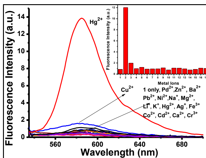
Figure 3.27. Fluorescence intensities of BOD-2 (5 μM) in 1:1 CH 3 CN/HEPES buffer at pH = 7.0 at λ max : 585 nm in the presence of 10.0 equivalents of the cations of interest and Hg 2+ (1.0 equiv.).
