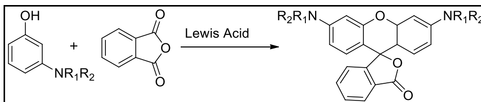
Figure 1.3. Synthetic scheme for Rhodamine core (Source: Noelting and Dziewoński, 1905)
