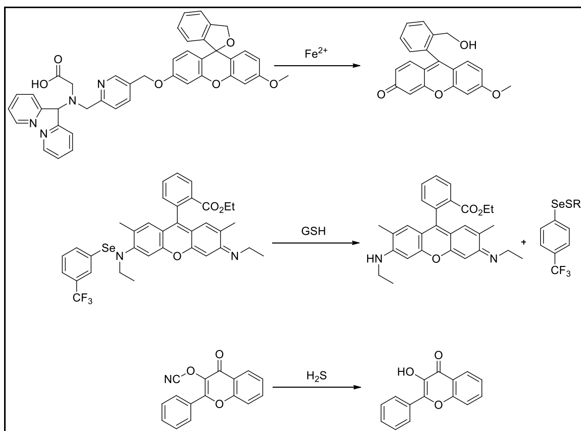
Figure 1.40. Fluorescent molecular sensors work via hydrolysis mechanism (Source: Aron et al., 2015; Manjare et al., 2014; Karakuş et al., 2016)
