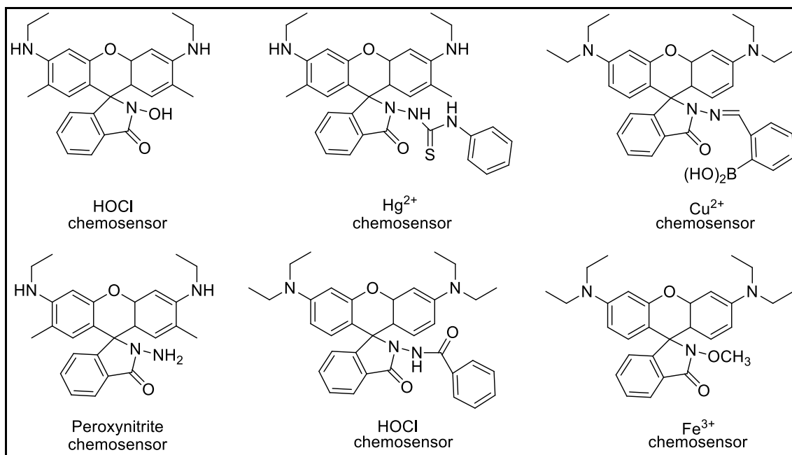
Figure 1.4. Rhodamine based chemosensors (Source: Beija et al., 2009)
