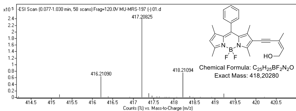
Figure B.7. Mass Spectrum of BOD-5 ((Z)-5,5-difluoro-8-(5-hydroxy-3-methylpent-3-en-1-yn-1-yl)-1,3,7,9-tetramethyl-10-phenyl-5H-dipyrrolo[1,2-c:2',1'-f][1,3,2]diazaborinin-4-ium-5-uide)
