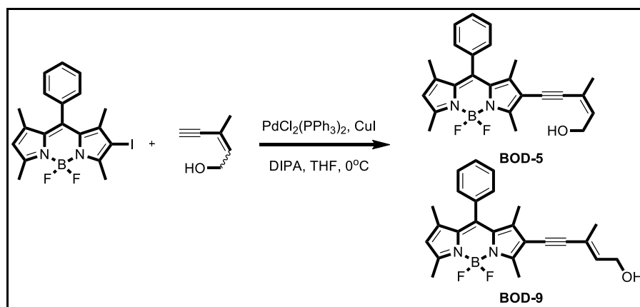
Figure 2.54. Synthesis route of BOD-5 and BOD-9
