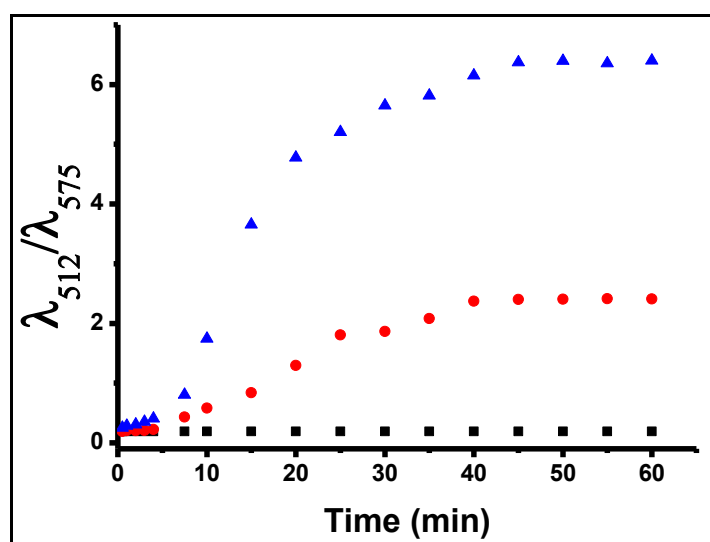
Figure 2.58. Reaction time profiles of BOD-5 (10 μM) in the absence (■) or presence of Au 3+ [10 (●), 30(▲) μM.]. The fluorescence intensities at 512 nm and 575 nm were continuously monitored at time intervals in 0.1 M phosphate buffer/EtOH (pH 7.0, v/v, 7:3) ( \lambda_{\text{ex}} : 460 nm, emission wavelengths: \lambda_{512}/\lambda_{575} at 25 °C).
