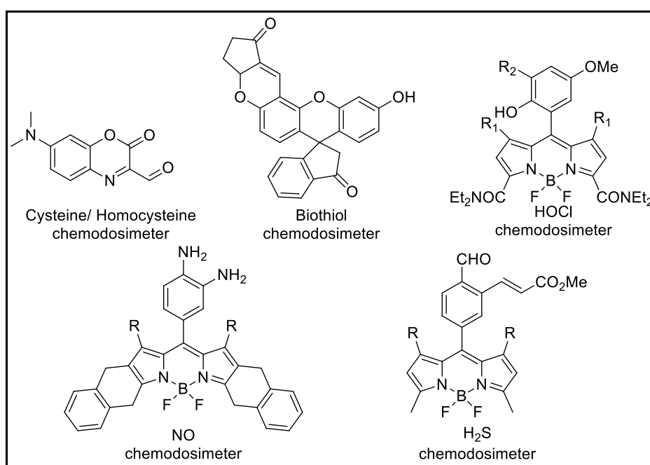
Figure 1.39. Fluorescent molecular sensors working via reaction based approach (Source: Zhou and Joon, 2012; Kowada et al., 2015)
