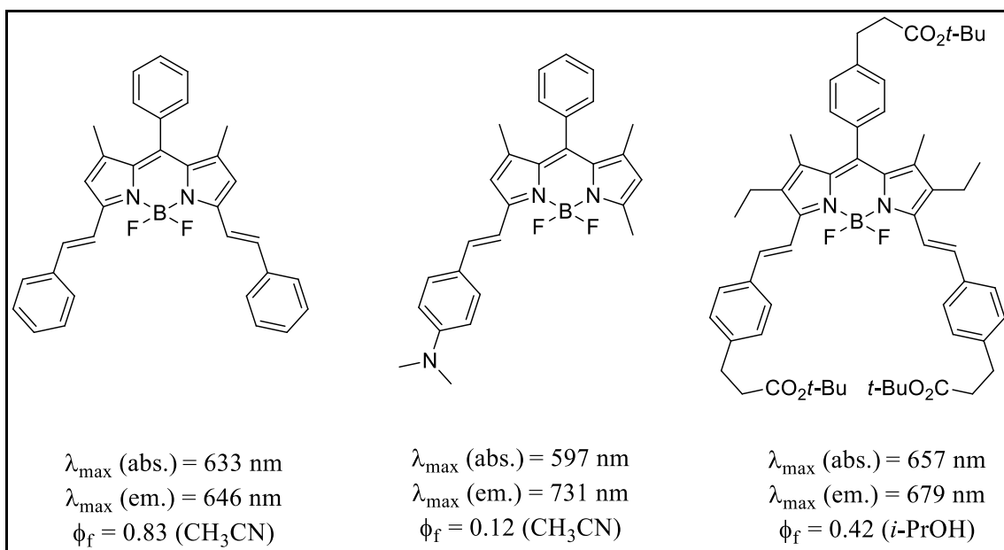
Figure 1.28. BODIPY structures synthesized via Knoevenagel condensation. (Source: Ni and Wu, 2014)
