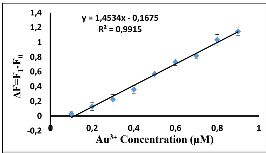
Figure 2.37. Fluorescence changes of BOD-3 (10 \mu\text{M} ) in 0.1 M phosphate buffer/EtOH (pH = 7.0, v/v, 1:4) upon the addition of \text{Au}^{3+} (0.01 to 0.1 equiv.) (0.1-1 \mu\text{M} ) (25°C, \lambda_{\text{ex}}=460 nm).
