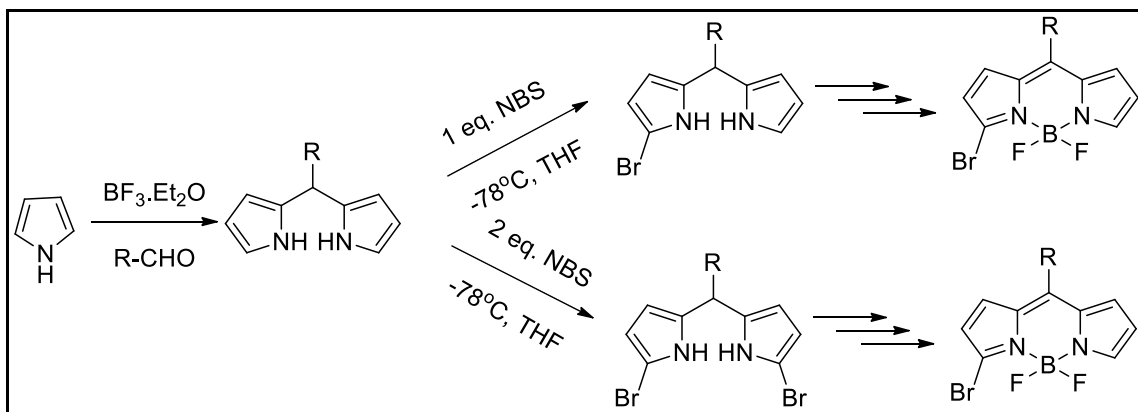
Figure 1.23. Synthesis of 3- and 3,5-bis- halogenated BODIPYs (Source: Lakshmi et al., 2015)
