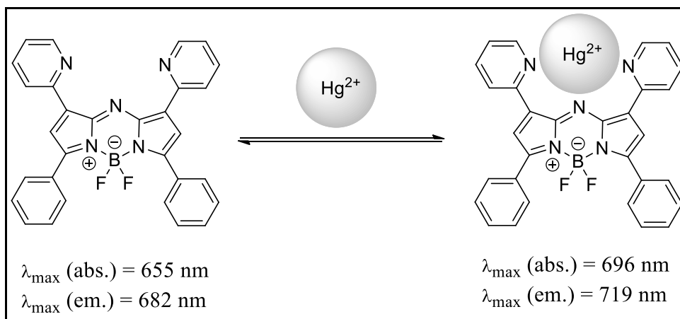
Figure 3.8. \text{Hg}^{2+} -induced response of modified boratriazaindacene (Source: Coskun et al., 2007)
