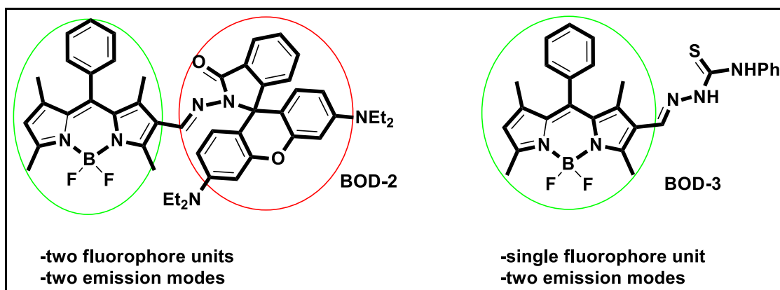
Figure 3.32. Chemical structure of BOD-2 and BOD-3
