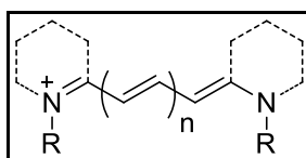
Figure 1.9. General structure of cyanine dyes (Source: Narayanan and Patonay, 1995)
