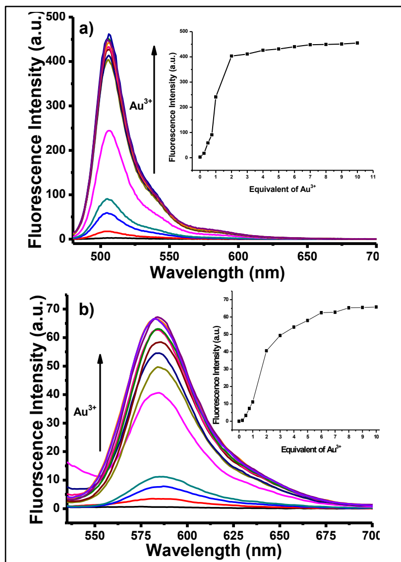
Figure 2.27. Fluorescence spectra of BOD-2 (5 μM) in 1:1 CH 3 CN/HEPES buffer at pH = 7.0 in the presence of Au 3+ (mole equivalents = 0.25 - 10.0 ) a) λ exc = 470 nm, b) λ exc = 525 nm.
