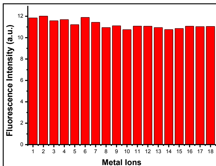
Figure 3.28. Fluorescence intensities of BOD-2 (5 \mu\text{M} ) in 1:1 \text{CH}_3\text{CN}/\text{HEPES} buffer at \text{pH} = 7.0 at \lambda_{\text{max}} : 585 nm in the presence \text{Hg}^{2+} (1.0 equiv.) and 10.0 equiv the following metal ions: 1, none; 2, \text{Cu}^{2+} ; 3, \text{Ag}^+ ; 4, \text{Zn}^{2+} ; 5, \text{Pb}^{2+} ; 6, \text{Ni}^{2+} ; 7, \text{Na}^+ ; 8, \text{Mg}^{2+} ; 9, \text{Li}^+ ; 10, \text{K}^+ ; 11, \text{Pd}^{2+} ; 12, \text{Fe}^{2+} ; 13, \text{Co}^{2+} ; 14, \text{Cd}^{2+} ; 15, \text{Ca}^{2+} ; 16, \text{Ba}^{2+} 17, \text{Cr}^{3+} ; 18, \text{Fe}^{3+}
