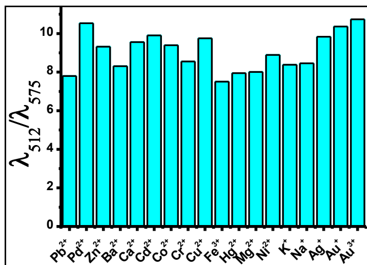
Figure 2.60. Fluorescence intensities of BOD-5 (10 \mu\text{M} ) in the presence of \text{Au}^{3+} (200 \mu\text{M} , 20 equiv.) and 20 equiv. of other metal ions in 0.1 M phosphate buffer pH 7.0/EtOH (v/v, 7:3) ( \lambda_{\text{ex}} : 460 nm, emission wavelengths: \lambda_{512}/\lambda_{575} at 25 ^{\circ}\text{C} ).
