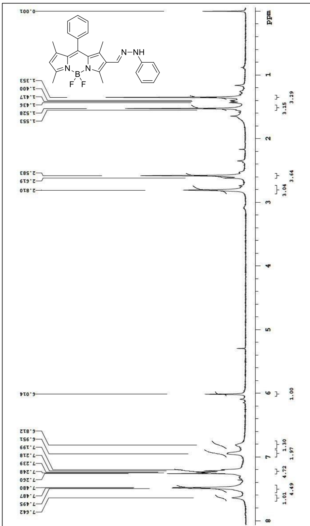
Figure A.7. ^1\text{H} NMR of (E)-5,5-difluoro-1,3,7,9-tetramethyl-10-phenyl-8-((2-phenylhydrazono)methyl)-5H-dipyrrolo[1,2-c:2,1'-f][1,3,2]diazaborinin-4-ium-5-uide
