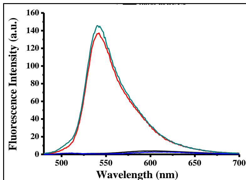
Figure 3.36. Fluorescence intensity changes of BOD-3 (black line) (10 \mu\text{M} ) in EtOH at pH = 7.0 at \lambda_{\text{max}} = 542 \text{ nm} after addition of 10 equiv. \text{Hg}^{2+} (red line), 10 equiv. \text{Hg}^{2+} + 10 equiv. \text{Na}_2\text{S} (blue line), 10 equiv. \text{Hg}^{2+} + 10 equiv. \text{Na}_2\text{S} + 10 equiv. \text{Hg}^{2+} (green line). ( \lambda_{\text{ex}} = 460 \text{ nm} )
