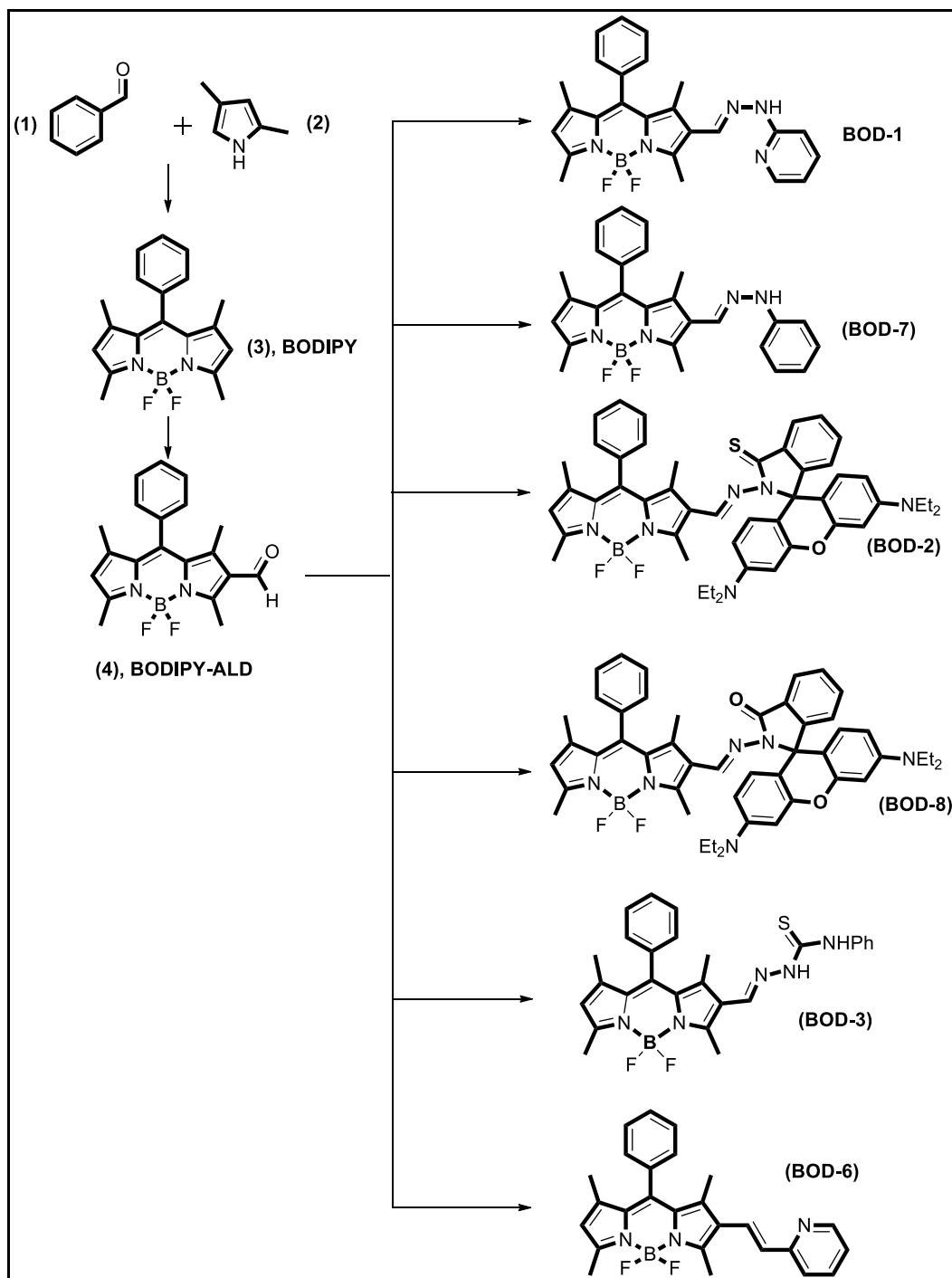
Figure 4.1. Synthetic routes of probe molecules from (4), BODIPY-ALD
