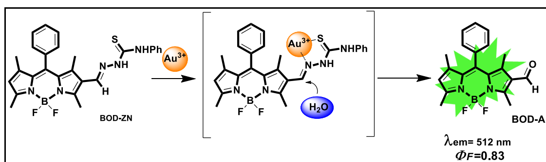
Figure 2.41. Hydrolysis mechanism of BOD-3 in the presence of \text{Au}^{3+} ions.
