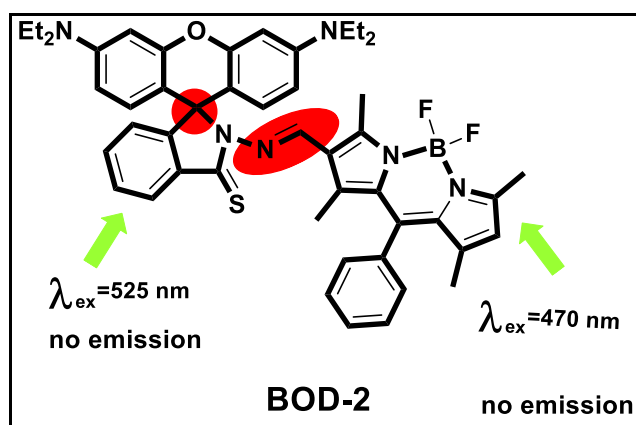
Figure 2.25. Structure of BOD-2
