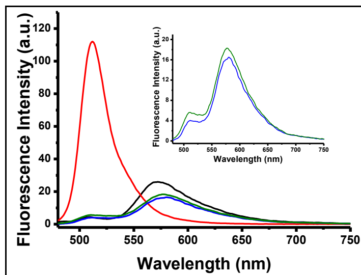
Figure 2.62. Fluorescence responses of BOD-5 (10 \mu\text{M} ) and BOD-9 (10 \mu\text{M} ) in reaction conditions (0.1 M phosphate buffer/EtOH (pH 7.0, v/v, 7:3) ( \lambda_{\text{exc}}=460 nm at 25 ^{\circ}\text{C} ). [( BOD-5 ): black line, ( BOD-5 + \text{Au}^{3+} (100 \mu\text{M} )): red line, ( BOD-9 ): blue line and ( BOD-9 + \text{Au}^{3+} (100 \mu\text{M} )): green line]
