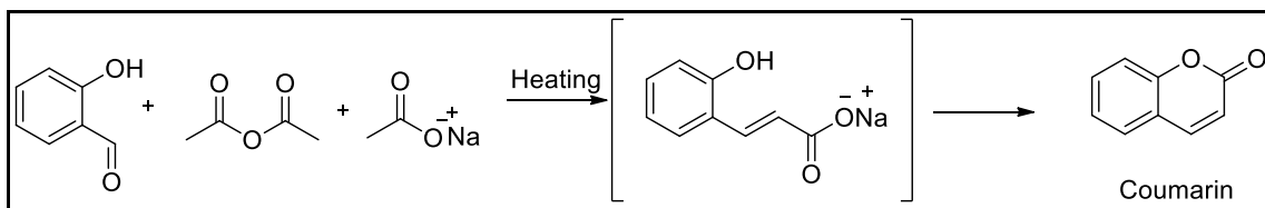
Figure 1.6. Synthesis of Coumarin structure by using Perkin reaction (Source: Perkin, 1868)
