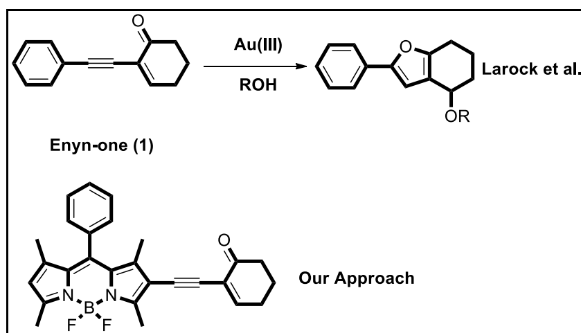
Figure 2.43. Work of both our and the Larock group.
