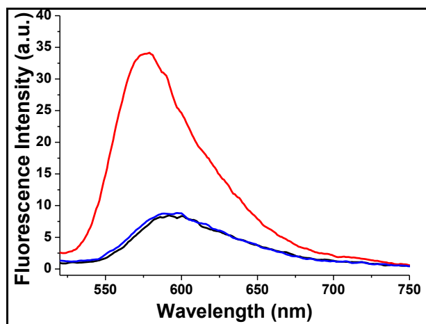
Figure 2.75. Fluorescence intensities of BOD-6 (10 \mu\text{M} ) (black), BOD-6 (10 \mu\text{M} ) + \text{Au}^{3+} (red), BOD-6 (10.0 \mu\text{M} ) + \text{Au}^{3+} + excess amount of \text{CN}^- (blue), in 0.1M potassium phosphate buffer, pH 7.0/EtOH (v/v, 1:1) ( \lambda_{\text{ex}} : 500 nm, at 25 ^\circ\text{C} ).
