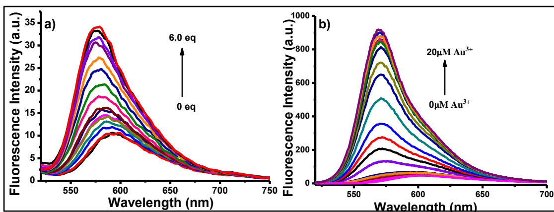
Figure 2.74. Fluorescence spectra of BOD-6 (10 \mu M) in the presence of increasing concentrations of Au 3+ a) (0-60 \mu M, 0-6 equiv.) in 0.1 M phosphate buffer/EtOH (pH 7.0, v/v, 1:1) ( \lambda_{exc} =500 nm at 25 ^{\circ} C) and b) (0-20 \mu M, 0-2 equiv.) in DCE.
