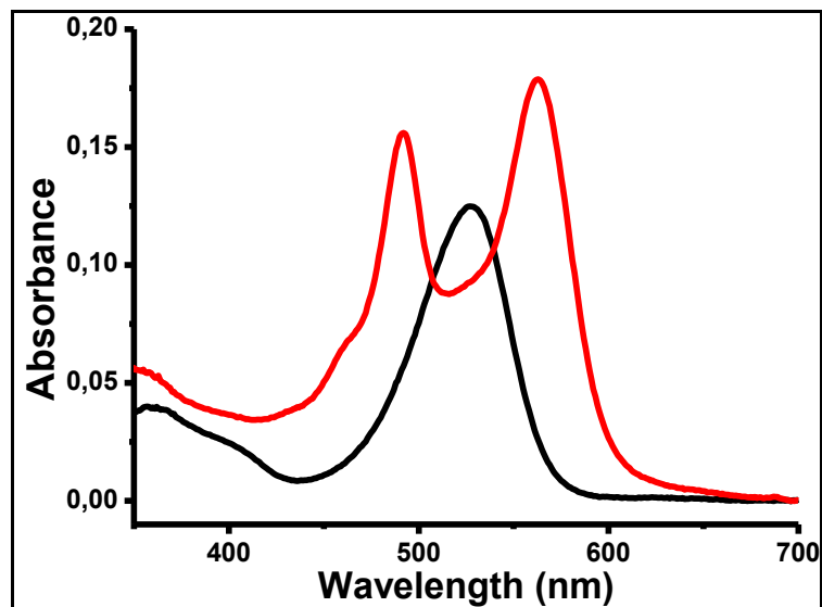
Figure 2.26. Absorption spectra of BOD-2 (5 μM) and \text{Au}^{3+} (1 equiv.) in 1:1 \text{CH}_3\text{CN}/\text{HEPES} buffer at pH = 7.0; ( \lambda_{\text{ex}} : 470 nm, at 25 °C).
