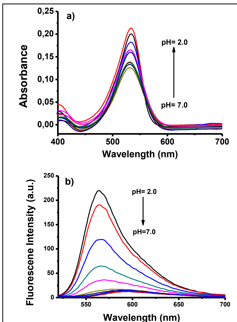
Figure 2.80. a) Absorbance and b) Fluorescence spectra of BOD-6 (10 \mu\text{M} ) in 0.1 M phosphate buffer/EtOH (v/v, 1:1) at various pH values (2.0-7.0) ( \lambda_{\text{exc}}=500 nm, 25 ^{\circ}\text{C} ).
