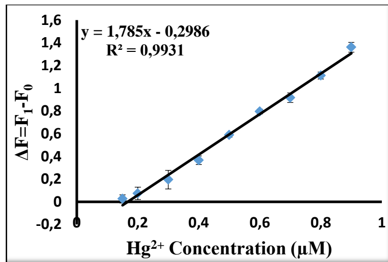
Figure 3.35. Fluorescence changes of BOD-3 (10 \mu\text{M} ) in 0.1 M phosphate buffer/EtOH (pH = 7.0, v/v, 1:4) upon addition of \text{Hg}^{2+} (0.01 to 0.1 equiv.) (0.1-1 \mu\text{M} ) ( \lambda_{\text{ex}} = 460 \text{ nm} , \lambda_{\text{em}} = 542 \text{ nm} )
