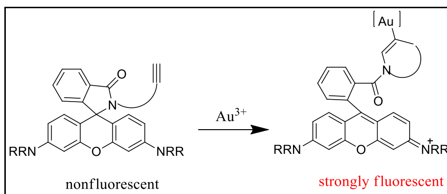
Figure 2.1. First example of gold ion sensors (Source: Yang et al, 2009)
