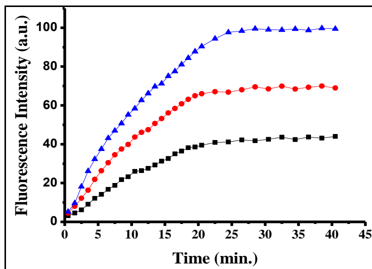
Figure 2.38 Time-dependent fluorescence change of BOD-3 (10 \mu\text{M} ) in the presence of 1.0 (■), 3.0 (●) and 5.0 (▲) equiv. (10, 30 and 50 \mu\text{M} ) of \text{AuCl}_3 measured in 0.1 M phosphate buffer/EtOH (pH = 7.0, v/v, 1:4) ( \lambda_{\text{ex}} = 460 nm, \lambda_{\text{em}} = 512 nm).
