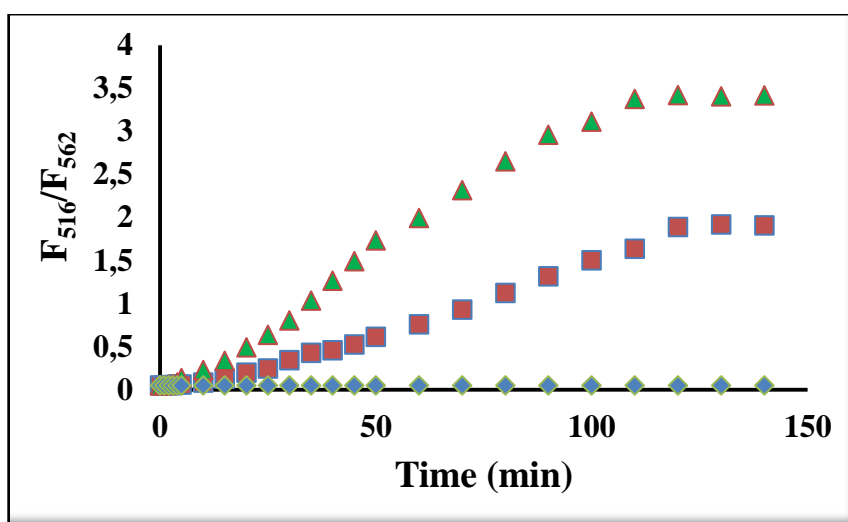
Figure 3.43. Reaction time profiles of BOD-4 (5 \mu\text{M} ) in the absence ( \blacklozenge ) or presence of \text{Hg}^{2+} [5( \blacksquare ), 10( \blacktriangle ) \mu\text{M} ]. The fluorescence intensities were continuously monitored at time intervals in 0.1 M phosphate buffer/EtOH (pH 7.0, v/v, 6:4) ( \lambda_{\text{exc}} =460 nm at 25 °C).
