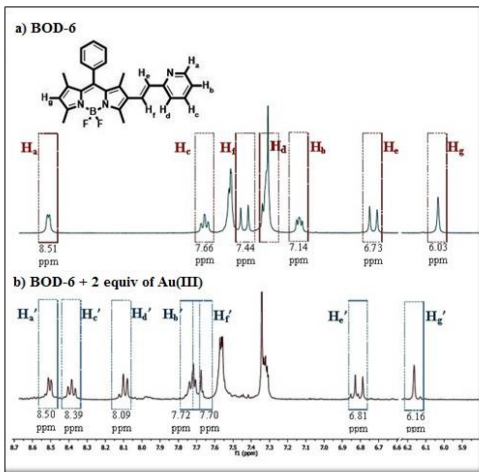
Figure 2.77. a) Partial 1 H NMR spectra of BOD-6 and b) BOD-6 + AuCl 3 (2 equiv.) in CDCl 3 .
