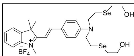
Figure 3.3. Hemicyanine based chemosensor for \text{Hg}^{2+} (Source: Li et al., 2011)
