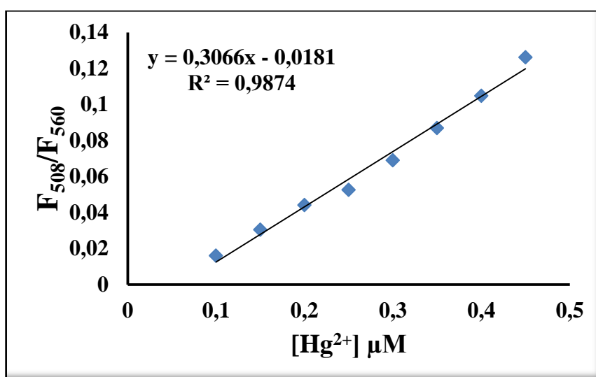
Figure 3.47. Fluorescence changes of BOD-4 (5.0 \mu\text{M} ) upon addition of \text{Hg}^{2+} (0,1 to 0,5 \mu\text{M} , 0.02 to 0.1 equiv.) in 10mM HEPES, pH 7.0/ \text{CH}_3\text{CN} (v/v, 6:4) ( \lambda_{\text{ex}} : 460 nm, at 25 °C).
