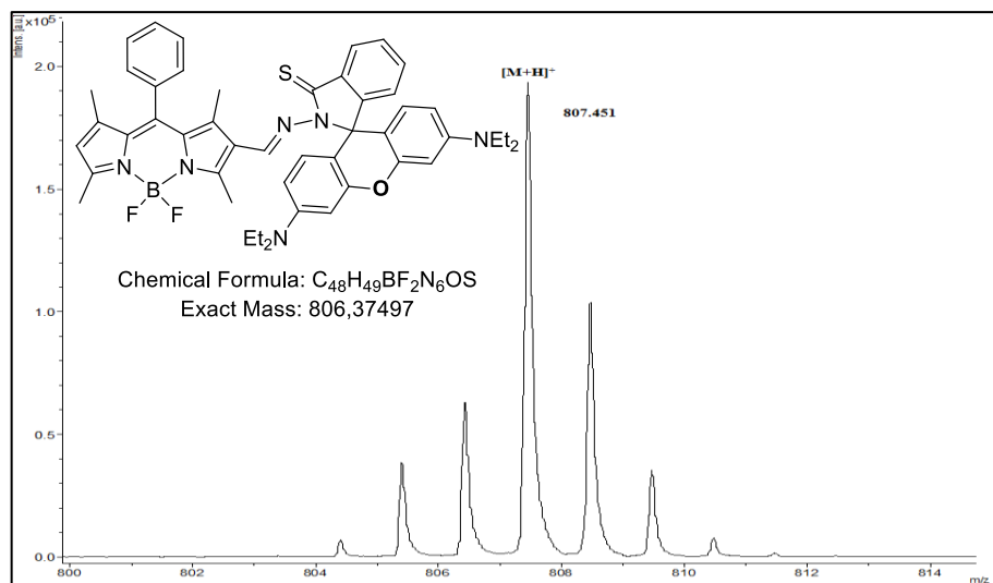
Figure B.3. MALDI-TOF Spectra of BOD-2 ((E)-8-(((3',6'-bis(diethylamino)-3-thioxospiro[isindoline-1,9'-xanthen]-2-yl)imino)methyl)-5,5-difluoro-1,3,7,9-tetramethyl-10-phenyl-5H-dipyrrolo[1,2-c:2',1'-f][1,3,2]diazaborinin-4-ium-5-uide)
