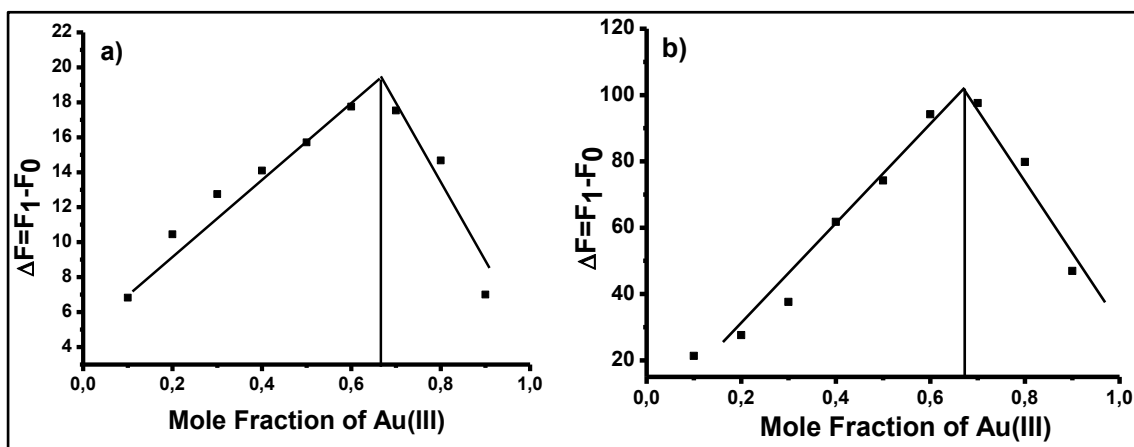
Figure 2.73. The Job's plot analysis between BOD-6 and \text{Au}^{3+} (a) in 0.1 M phosphate buffer/EtOH (pH 7.0, v/v, 1:1) (b) in ethanol. The total concentration of BOD-6 and \text{Au}^{3+} was kept constant at 20 \mu\text{M} ( \lambda_{\text{exc}}=500 \text{ nm} , \lambda_{\text{em}}=577 \text{ nm} at 25 \text{ }^\circ\text{C} ).
