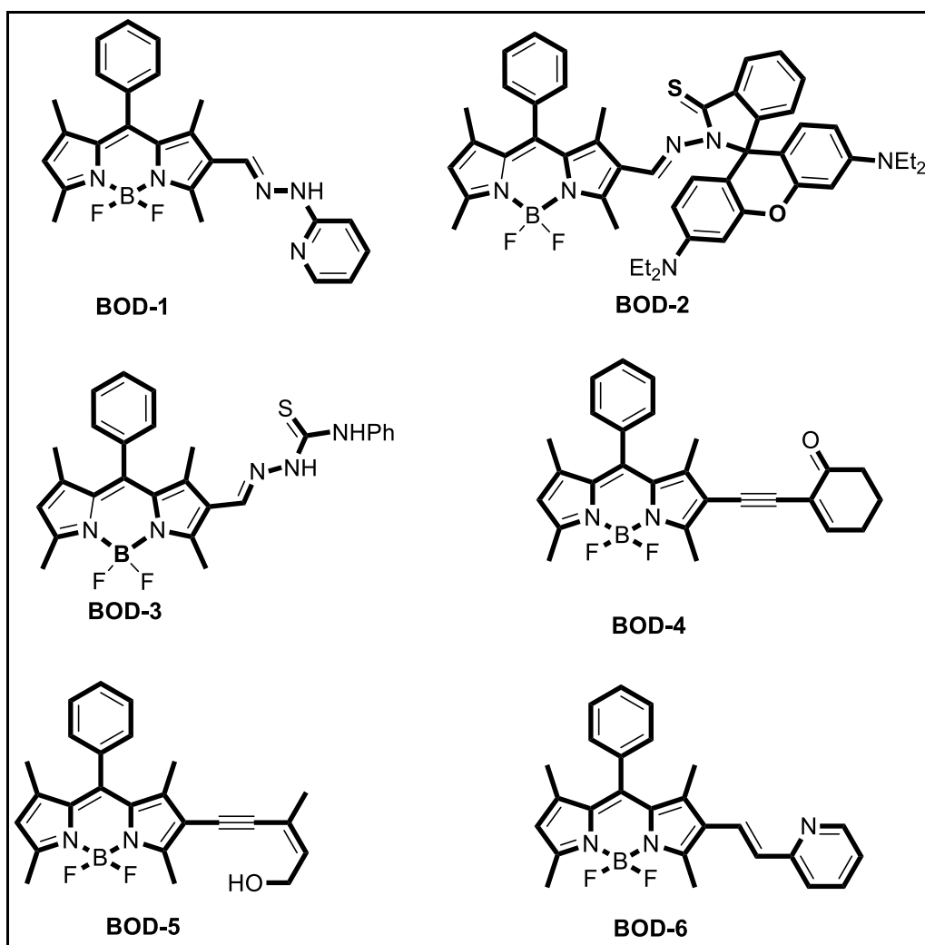
Figure 2.13. BODIPY based gold and mercury ions selective sensors.
