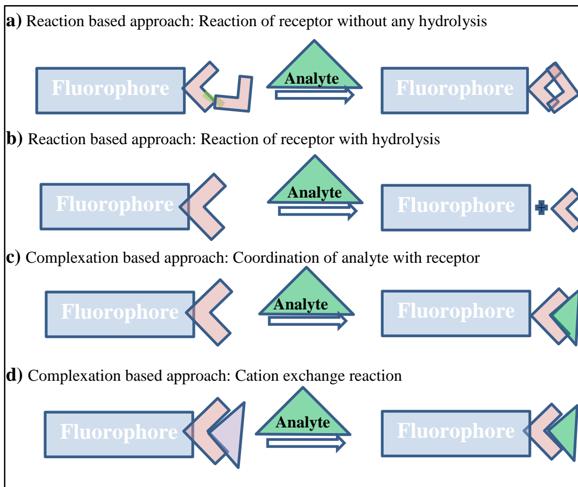
Figure 1.38. Sensing approaches to construct molecular sensors (Source: Patil et al., 2012; Cheng et al., 2015)
