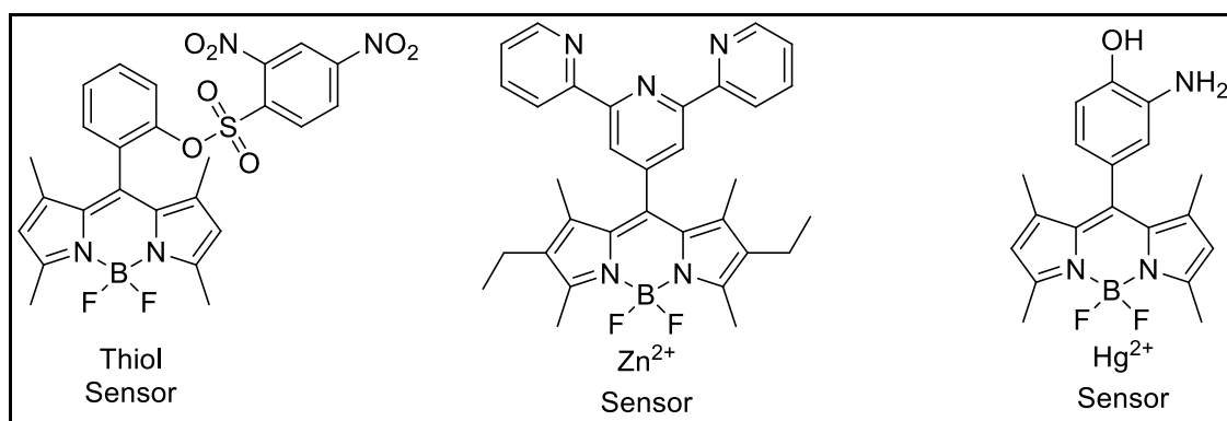
Figure 1.43. Examples of PET based sensors (Source: Boens et al., 2012)
