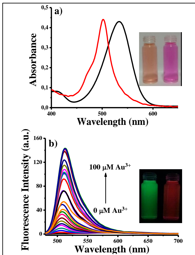
Figure 2.36. a) Absorbance spectra of BOD-3 (10 \mu\text{M} ) in the absence (black line) and presence (red line) of 10 equiv. (100 \mu\text{M} ) of \text{Au}^{3+} ; b) Fluorescence titration spectra of BOD-3 (10 \mu\text{M} ) + \text{Au}^{3+} (0.1 to 100 \mu\text{M} , 0.01 to 10 equiv.) in 0.1 M phosphate buffer / EtOH (pH 7.0, v/v, 1:4) (25°C, \lambda_{\text{ex}}=460 nm).
