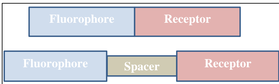
Figure 1.37. Structural design of a fluorescent sensor. (Source: Das et al., 2013)
