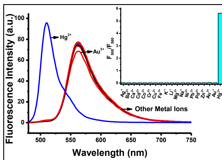
Figure 3.49. Fluorescence intensities of BOD-4 (5 \mu\text{M} ), BOD-4 (5 \mu\text{M} ) + \text{Hg}^{2+} (10 \mu\text{M} , 2 equiv.), BOD-4 (5 \mu\text{M} ) + other metal ions (50 \mu\text{M} , 10 equiv.) in 10 mM HEPES, pH 7.0/ \text{CH}_3\text{CN} (v/v, 6:4) ( \lambda_{\text{exc}} : 460 nm, at 25 ^\circ\text{C} ). Inset: Bar graph notation.
