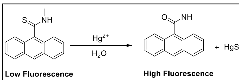
Figure 3.1. Response of the developed probe with the addition of \text{Hg}^{2+} (Source: Chae and Czarnik, 1992)
