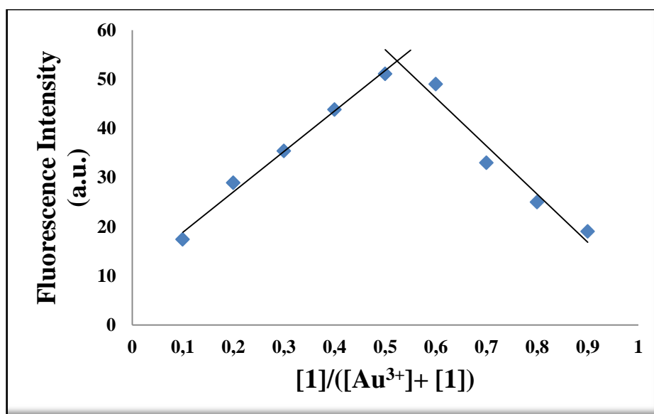
Figure 2.32. Job's plot for the rhodamine derivative and \text{Au}^{3+} in 1:1 \text{CH}_3\text{CN}/\text{HEPES} solution at \lambda_{\text{ex}} : 525 nm
