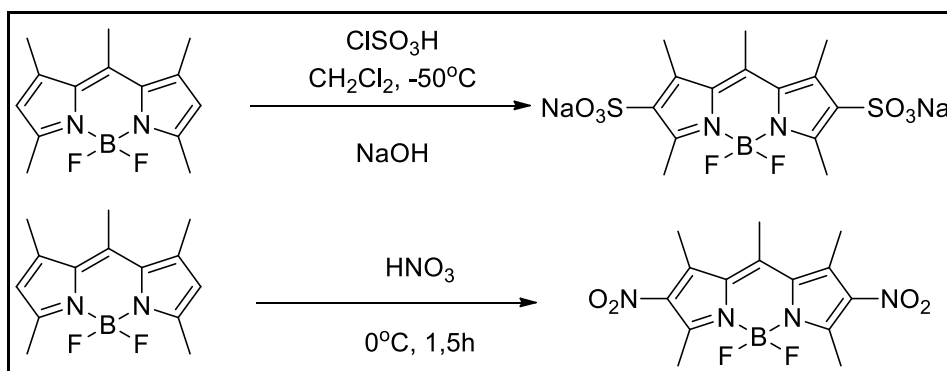
Figure 1.35. Sulfonation and nitration reactions of BODIPY from 2,6- positions (Source: Wories et al., 1985; Esnal et al., 2013)
