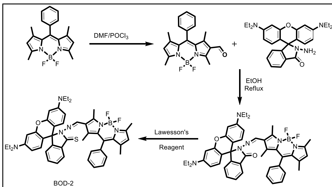
Figure 2.24. Synthetic route to BOD-2
