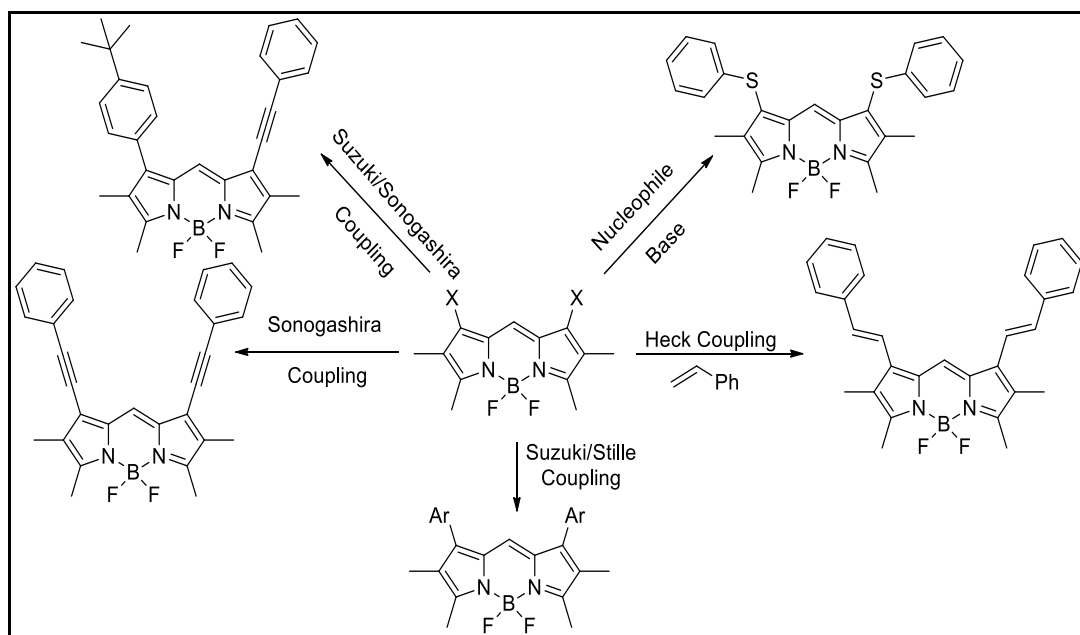
Figure 1.30. Reactions of BODIPY core halogenated from 1,7- positions (Source: Lakshmi et al., 2015)
