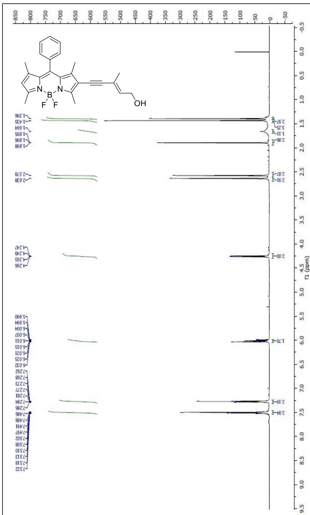
Figure A.21. 1 H NMR of (E)-5,5-difluoro-8-(5-hydroxy-3-methylpent-3-en-1-yn-1-yl)-1,3,7,9-tetramethyl-10-phenyl-5H-dipyrrolo[1,2-c:2',1'-f][1,3,2]diazaborinin-4-ium-5-uide
