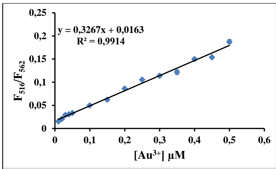
Figure 2.48. Fluorescence changes of BOD-4 (5.0 μM) upon addition of Au 3+ (0,005 to 0,5 μM, 0. 001 to 0.1 equiv.) in 0.1M potassium phosphate buffer, pH 7.0/EtOH (v/v, 6:4) (λ ex : 460 nm, at 25 °C).
