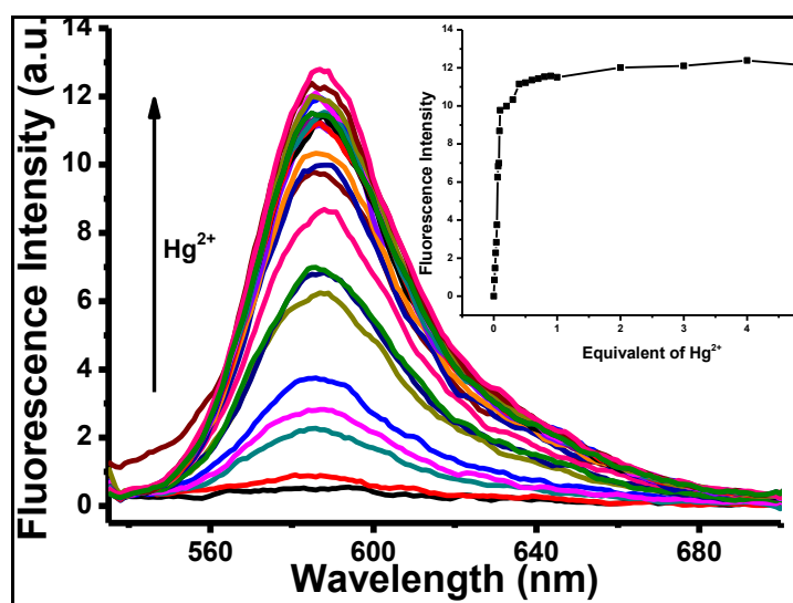
Figure 3.25. Fluorescence spectra of BOD-2 (5 \mu\text{M} ) in 1:1 \text{CH}_3\text{CN} /HEPES buffer at pH = 7.0 in the presence of \text{Hg}^{2+} (mole equivalents = 0.01 - 5.0). Inset: Calibration Curve.
