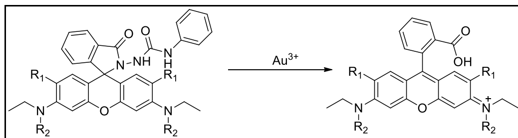
Figure 2.7. Fluorescent molecular sensor works via hydrolysis of acylsemicarbazide (Source: Yuan et al., 2011)
