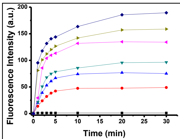
Figure 2.19. Reaction time profiles of BOD-1 (10 \mu\text{M} ) in the absence ( \blacksquare ) or presence of \text{Au}^{3+} [10 ( \bullet ), 30( \blacktriangle ), 50( \blacktriangledown ), 100 ( \blacktriangleleft ), 150( \blacktriangleright ), 200( \blacklozenge ) \mu\text{M} ]. The fluorescence intensities at 512 nm were continuously monitored at time intervals in 0.1 M phosphate buffer/EtOH (pH 7.0, v/v, 1:1) ( \lambda_{\text{exc}}=460 nm, \lambda_{\text{em}}=512 nm at 25 ^{\circ}\text{C} ).
