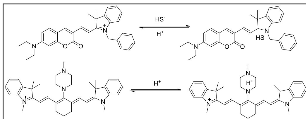
Figure 1.46. Examples of ICT based sensors (Source: Lee et al., 2015)
