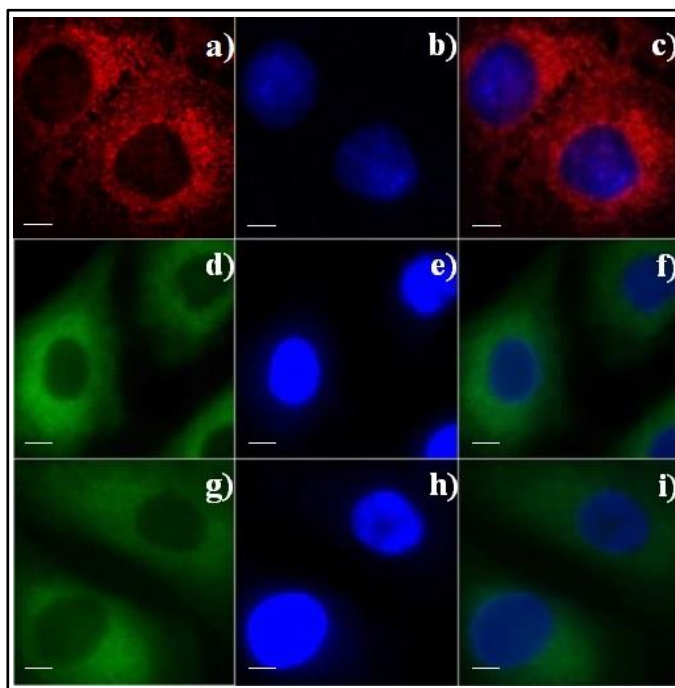
Figure 2.52. Fluorescence images of Human Lung Adenocarcinoma cells (A549). a) Fluorescence image of A549 cells treated with only BOD-4 (10 \mu\text{M} ); b, e, h) Fluorescence image of cells treated with DAPI (control); d, g) Fluorescence image of cells treated with BOD-4 (10 \mu\text{M} ) and \text{Au}^{3+} (10 \mu\text{M} ), \text{Hg}^{2+} (10 \mu\text{M} ); c, f, i) merged images of frames a-b, d-e and g-h ( \lambda_{\text{ex}} = 460 \text{ nm} ). Scale bar represents 10 \mu\text{m} .
