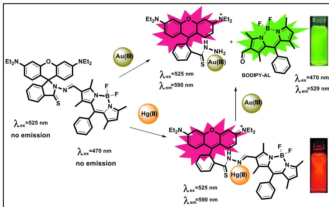
Figure 2.31. Response of BOD-2 towards the addition of \text{Au}^{3+} and \text{Hg}^{2+}
