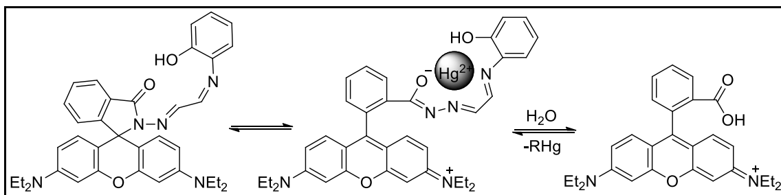
Figure 3.6. \text{Hg}^{2+} mediated hydrolysis of Rhodamine derivative (Source: Du et al., 2010)
