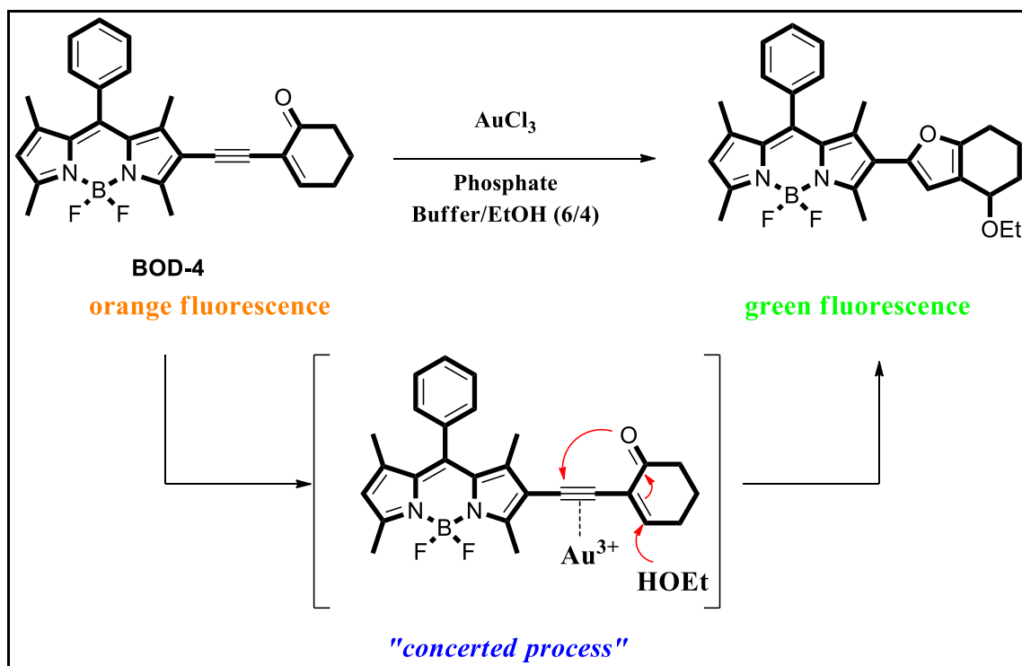
Figure 2.47. Proposed reaction mechanism for the detection of gold ions
