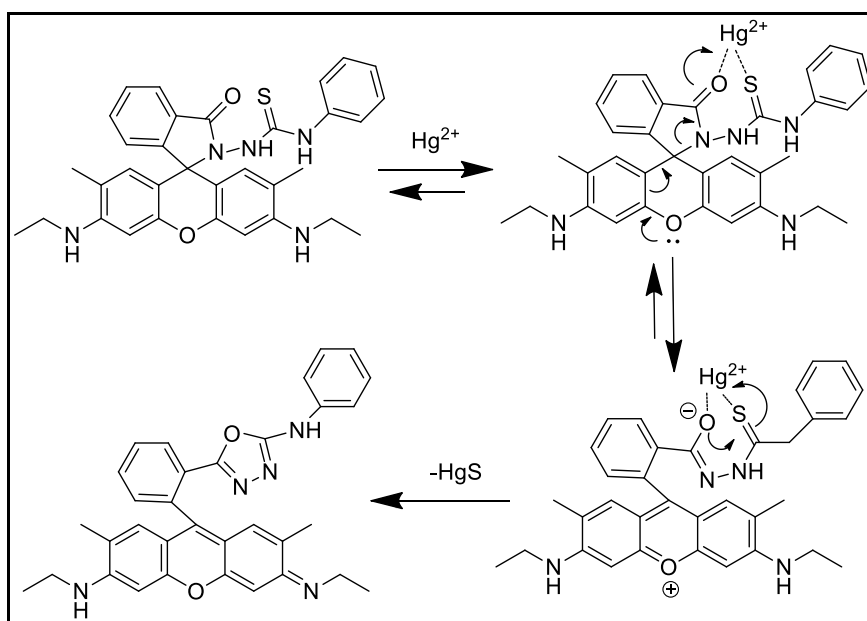
Figure 3.11. \text{Hg}^{2+} -induced ring opening and cyclization of the designed rhodamine derivative (Source: Yang et al., 2005)
