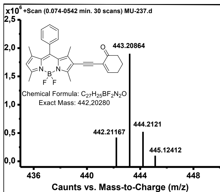
Figure B.6. Mass Spectrum of BOD-4 (5,5-difluoro-1,3,7,9-tetramethyl-8-((6-oxocyclohex-1-en-1-yl)ethynyl)-10-phenyl-5H-dipyrrolo[1,2-c:2',1'-f][1,3,2]diazaborinin-4-ium-5-uide)
