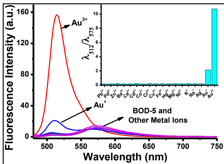
Figure 2.59. Fluorescence intensities of BOD-5 (10 \mu\text{M} ), BOD-5 (10 \mu\text{M} ) + \text{Au}^{3+} (100 \mu\text{M} , 10 equiv.), BOD-5 (10 \mu\text{M} ) + other metal ions (200 \mu\text{M} , 20 equiv.) in 0.1M potassium phosphate buffer, pH 7.0/EtOH (v/v, 7:3) ( \lambda_{\text{ex}} : 460 nm, at 25 ^{\circ}\text{C} ). Inset: Bar graph notation.
