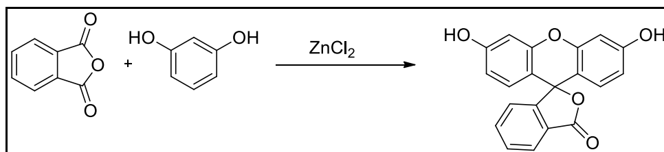
Figure 1.1. Synthesis of fluorescein fluorophore (Source: Orndorff and Hemmer, 1927)
