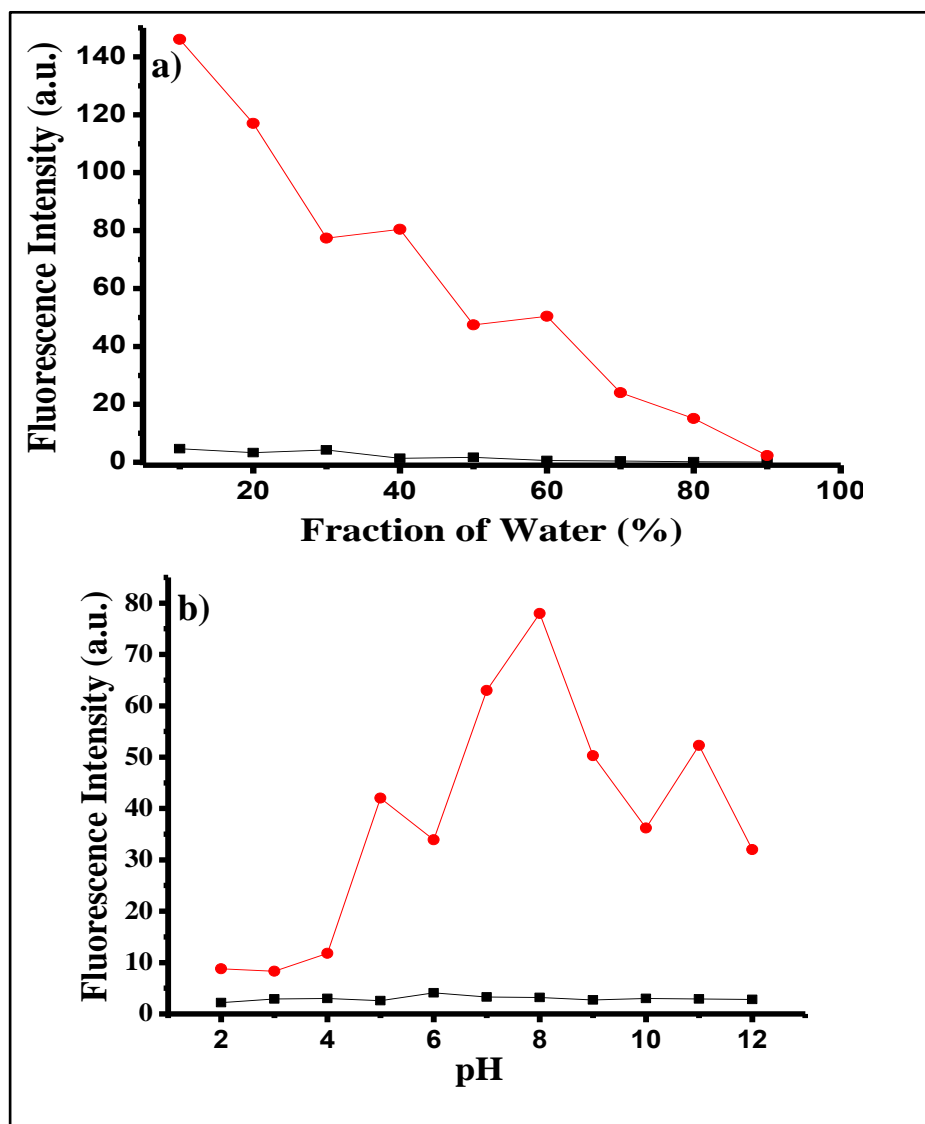
Figure 2.35. a) Effect of fraction of water (pH 7.0/EtOH ) and b) Effect of pH (pH/EtOH (v/v, 1:4)) on the interaction of BOD-3 (10 \mu M) (black line) with Au 3+ (200 \mu M, 20 equiv.) (red line) in 0.1M potassium phosphate buffer, ( \lambda_{\text{ex}} : 460 nm, \lambda_{\text{em}} = 512 nm at 25 °C).
