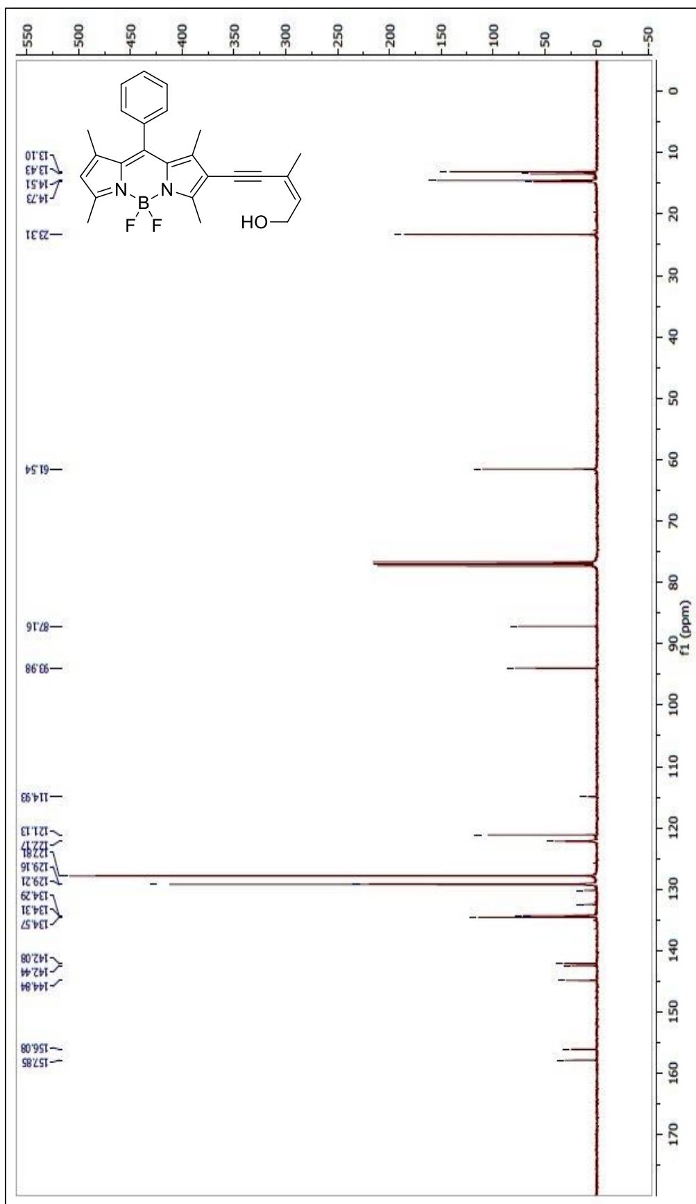
Figure A.20. ^{13}\text{C} NMR of (Z)-5,5-difluoro-8-(5-hydroxy-3-methylpent-3-en-1-yn-1-yl)-1,3,7,9-tetramethyl-10-phenyl-5H-dipyrrolo[1,2-c:2',1'-f][1,3,2]diazaborinin-4-ium-5-uide
