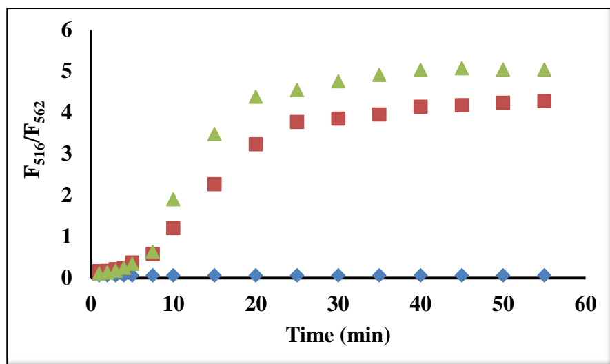
Figure 2.49. Reaction time profiles of BOD-4 (5 μM) in the absence (♦) or presence of Au 3+ [5 (■), 10(▲) μM]. The fluorescence intensities were continuously monitored at time intervals in 0.1 M phosphate buffer/EtOH (pH 7.0, v/v, 6:4) (λ exc =460 nm at 25 °C).
