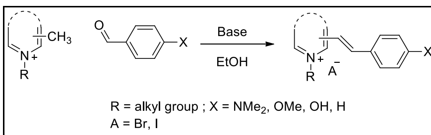
Figure 1.8. Synthetic scheme of cyanine dyes (Source: Mishra et al., 2000)
