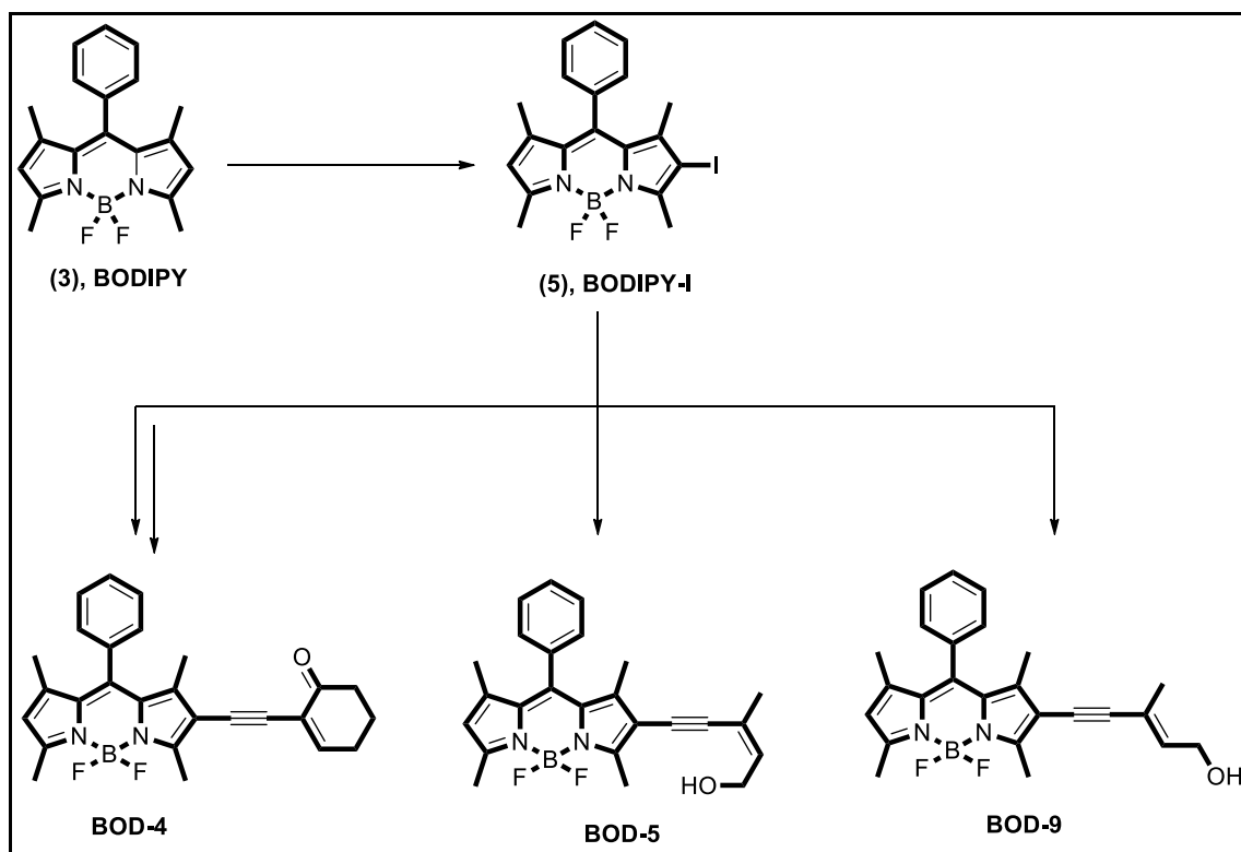
Figure 4.2. Synthetic routes of probe molecules from (5), BODIPY-I
