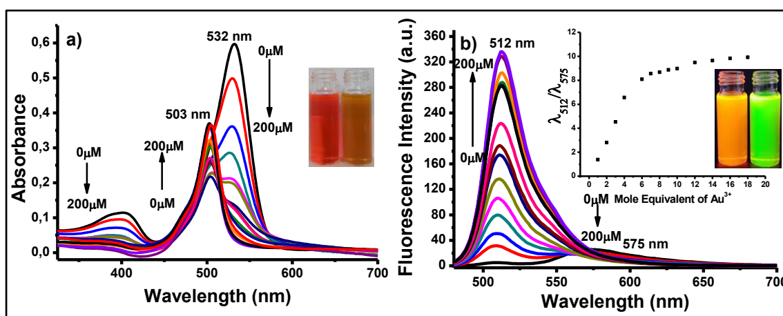
Figure 2.56. a) Absorbance and b) Fluorescence titration spectra of BOD-5 (10 μM) + Au 3+ (1 to 200 μM), 0.1 to 20 equiv.) in 0.1 M phosphate buffer / EtOH (pH 7.0, v/v, 7:3). Inset: Calibration curve.
