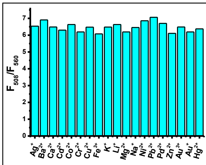
Figure 3.50. Fluorescence intensities of BOD-4 (5 \mu\text{M} ) in the presence of \text{Hg}^{2+} (10 \mu\text{M} , 2 equiv.) and 10 equiv. of other metal ions in 10 mM HEPES, pH 7.0/ \text{CH}_3\text{CN} (v/v, 6:4) ( \lambda_{\text{exc}}=460 nm at 25 ^\circ\text{C} )
