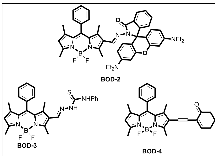
Figure 3.23. BODIPY based sensors detects both gold and mercury ions selectively.
