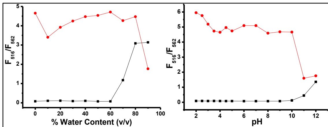
Figure 2.45. a) Effect of fraction of water (in 0.1M potassium phosphate buffer pH 7.0/EtOH) and b) Effect of pH (in 0.1M potassium phosphate buffer pH/EtOH (v/v, 6:4)) on the interaction of BOD-4 (5 \mu M) (black line) with Au 3+ (10 \mu M, 2 equiv.) (red line), ( \lambda_{ex} : 460 nm, \lambda_{em} = 516 nm at 25 °C).
