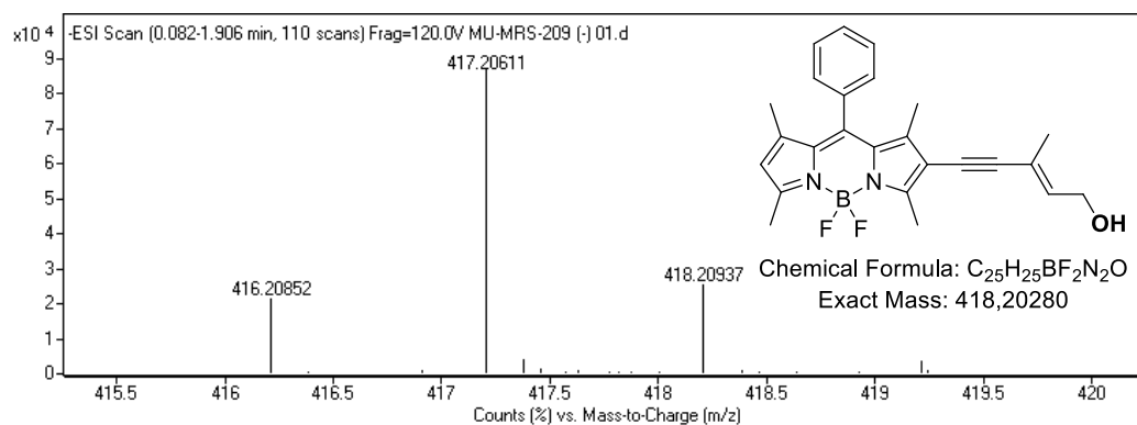
Figure B.8. Mass Spectrum of BOD-9 ((E)-5,5-difluoro-8-(5-hydroxy-3-methylpent-3-en-1-yn-1-yl)-1,3,7,9-tetramethyl-10-phenyl-5H-dipyrrolo[1,2-c:2',1'-f][1,3,2]diazaborinin-4-ium-5-uide)
