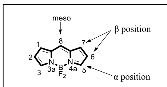
Figure 1.12. IUPAC numbering system of a boron dipyrrole compound (Source: Wood and Thompson, 2007)
