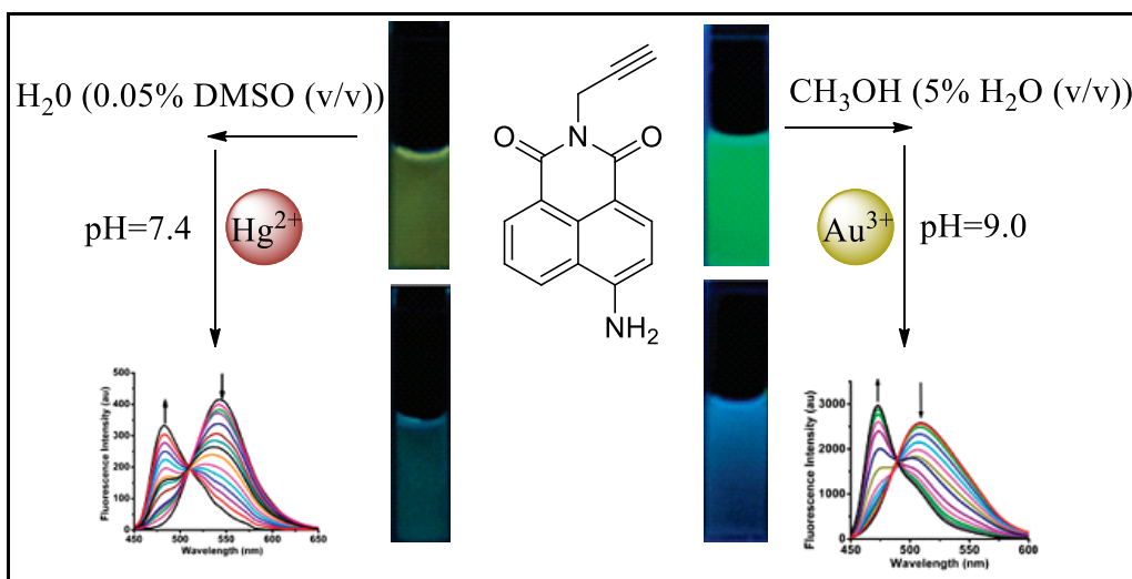
Figure 2.3. A ratiometric probe for gold and mercury ions (Source: Dong et al., 2010)
