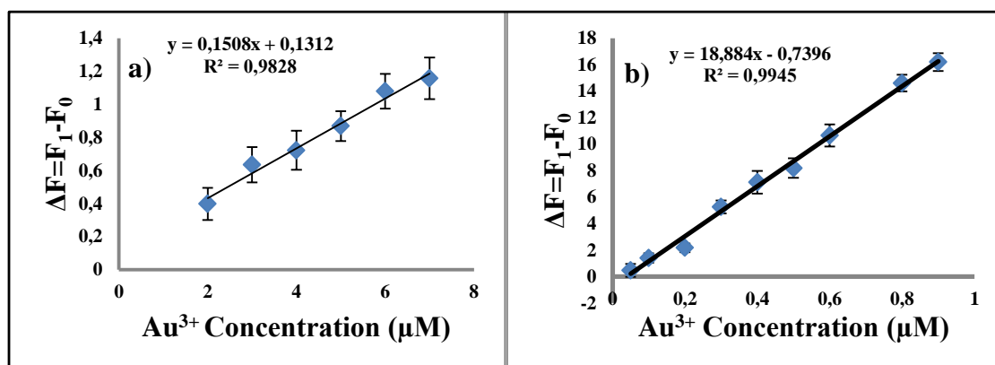
Figure 2.71. Fluorescence changes of BOD-6 (10 \mu M) upon addition of Au 3+ a) (2 to 7 \mu M, 0. 2 to 0.7 equiv.) in 0.1M potassium phosphate buffer, pH 7.0/EtOH (v/v, 1:1) b) (0.05 to 1.0 \mu M, 0.005 to 0.1 equiv.) in dichloroethane ( \lambda_{\text{ex}} : 500 nm, \lambda_{\text{em}} = 577 nm at 25 °C).
