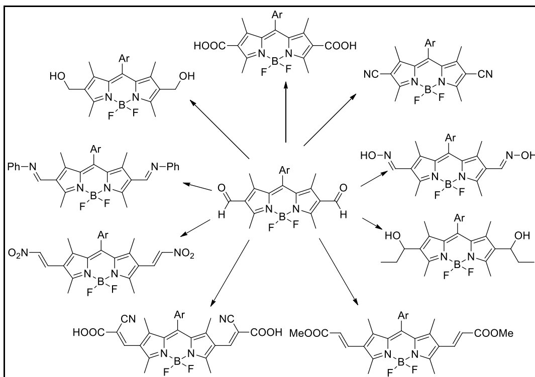
Figure 1.34. Derivatization possibilities of 2,6- formylated BODPYs (Source: Zu et al., 2013)
