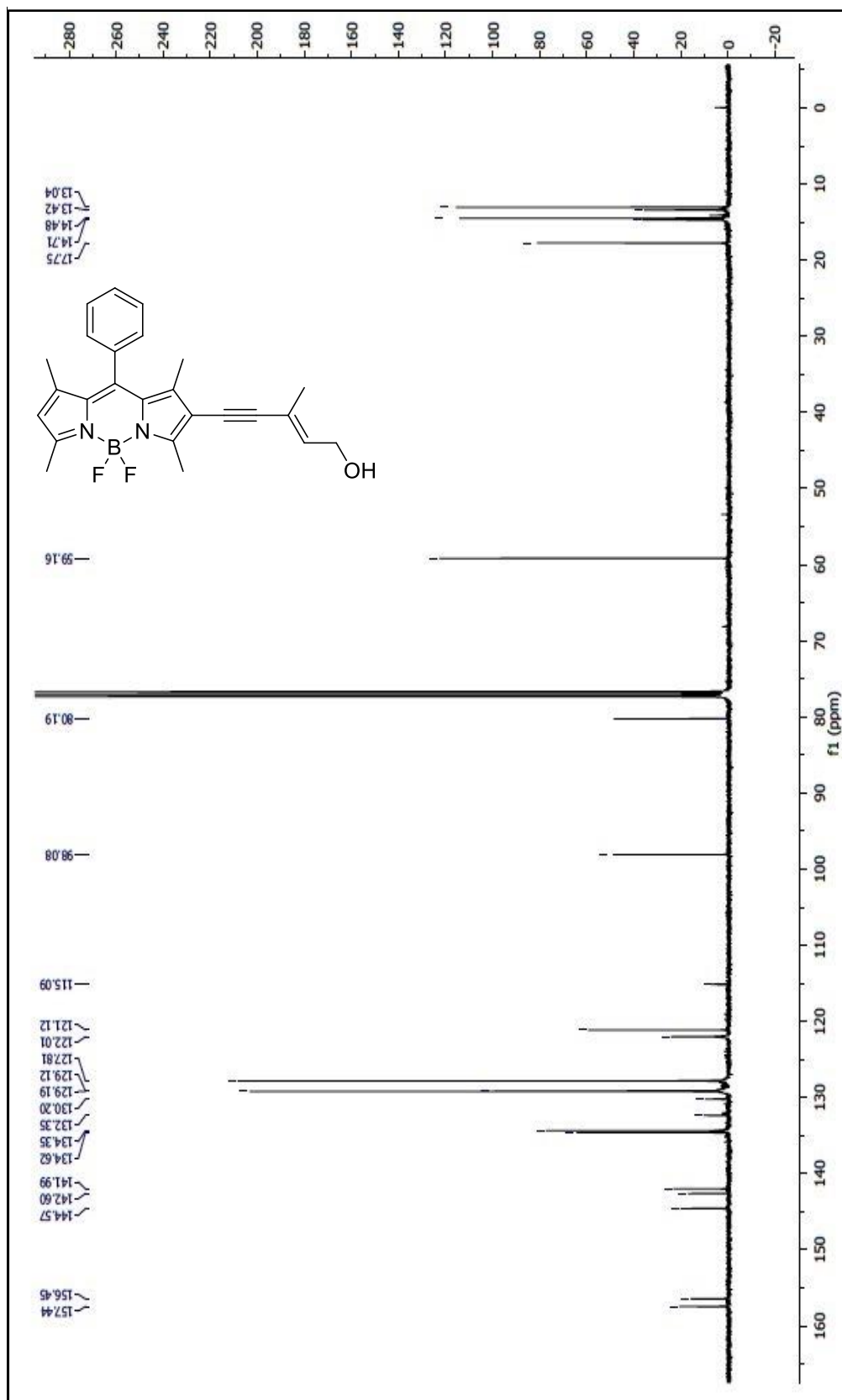
Figure A.22. ^{13}\text{C} NMR of (E)-5,5-difluoro-8-(5-hydroxy-3-methylpent-1-en-1-yn-1-yl)-1,3,7,9-tetramethyl-10-phenyl-5H-dipyrrolo[1,2-c:2',1'-f][1,3,2]diazaborinin-4-ium-5-uide
