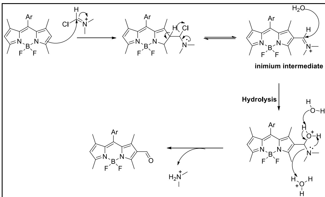
Figure 1.33. Reaction mechanism of Vilsmeier Haack's Formylation (Source: Jiao et al., 2009)
