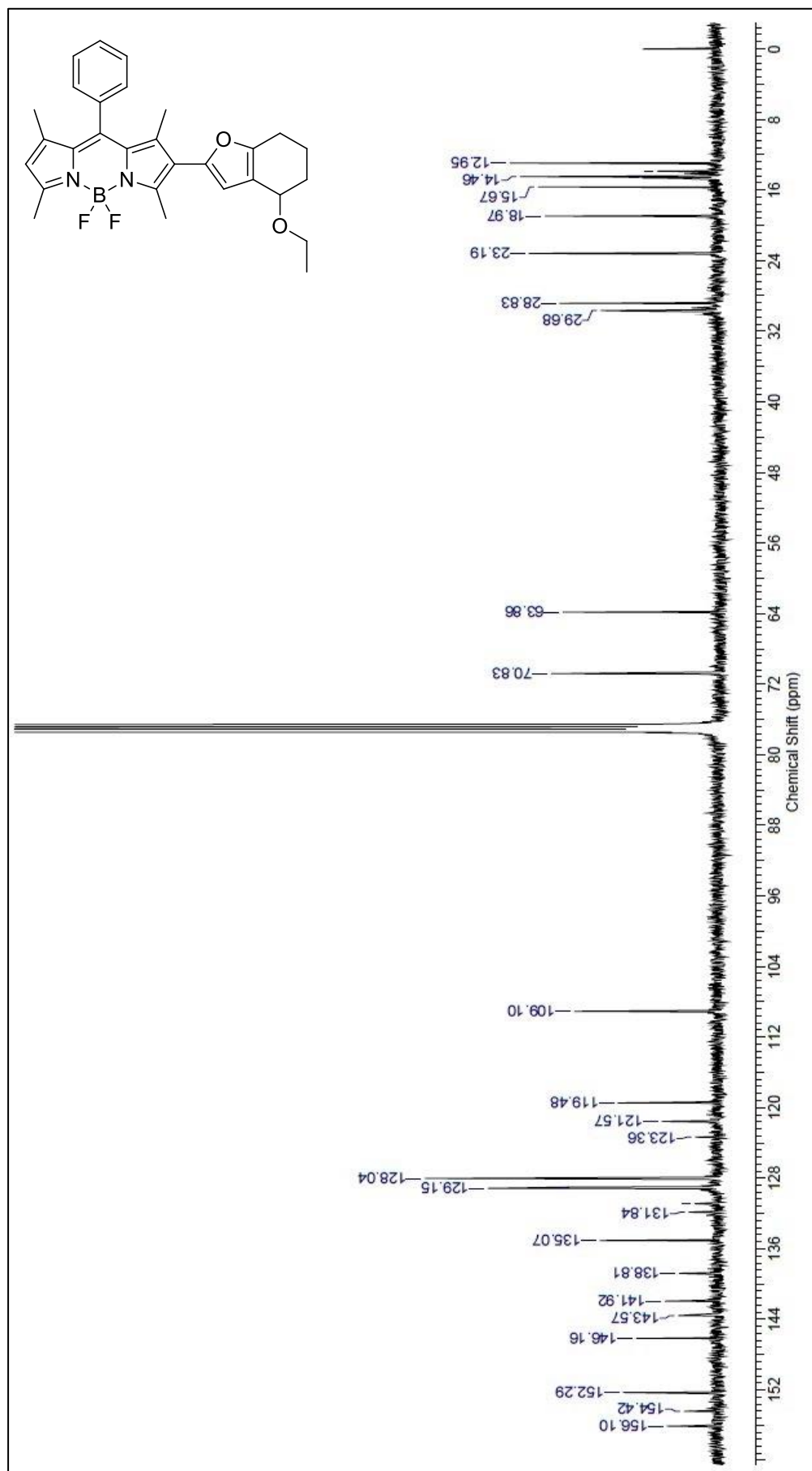
Figure A.24. 13 C NMR of (R)-8-(4-ethoxy-4,5,6,7-tetrahydrobenzofuran-2-yl)-5,5-difluoro-1,3,7,9-tetramethyl-10-phenyl-5H-dipyrolo[1,2-c:2',1'-f][1,3,2]diazaborinin-4-ium-5-uide
