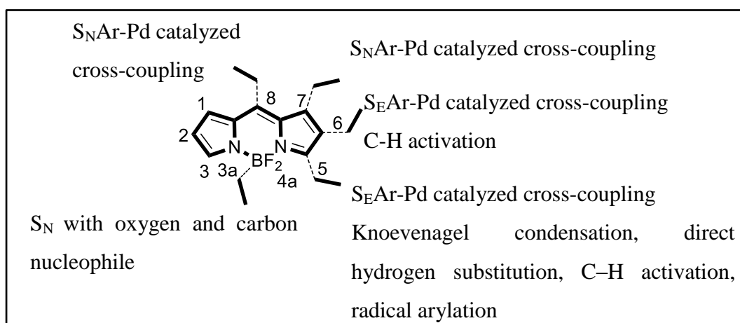
Figure 1.18. Possible post-functionalization sites of BODIPY structure (Source: Boens et al., 2015)
