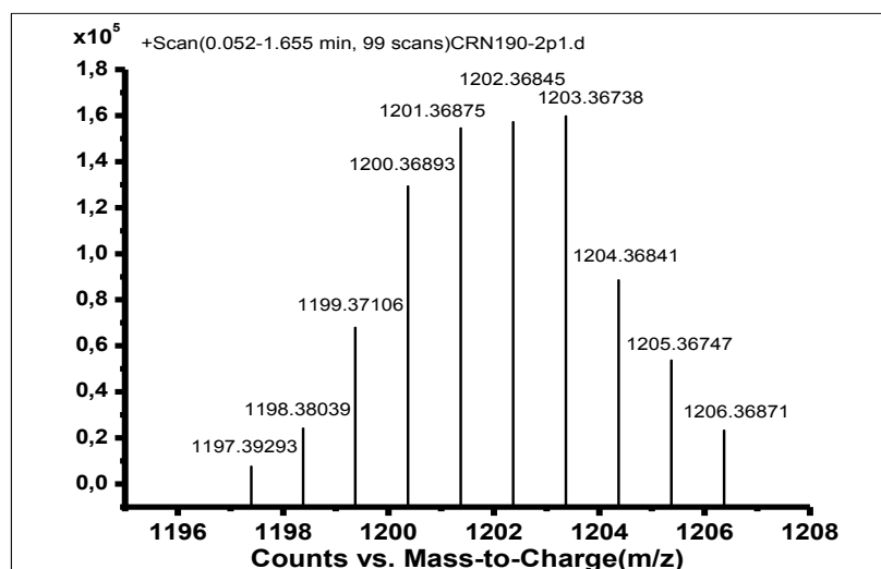
Figure B.5. Mass Spectrum of the Obtained \text{Hg}^{2+} -BOD-3 Complex
