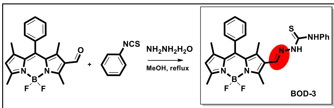
Figure 2.34. Synthesis route of BOD-3 .
