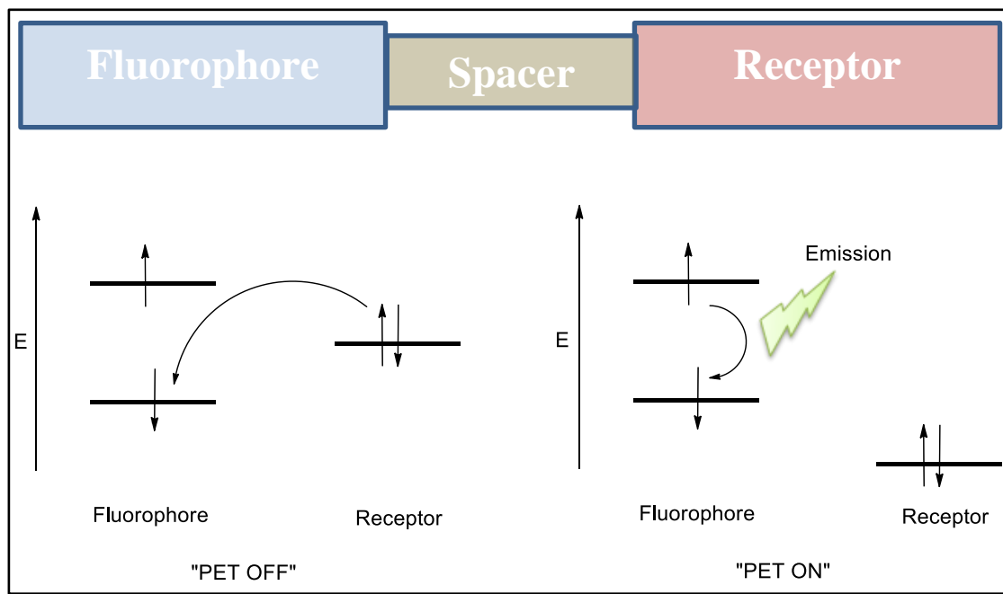
Figure 1.44. Photo-induced electron transfer mechanism (Source: Das et al., 2013)
