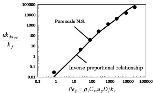
Fig. 3 Comparison of the inverse proportional relationship with DNS
