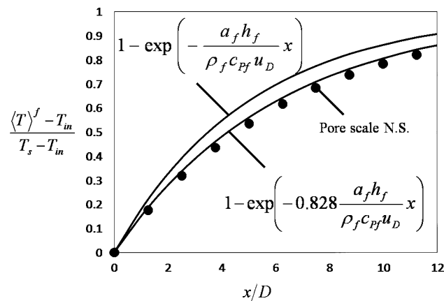
Fig. 7 Development of the fluid temperature
