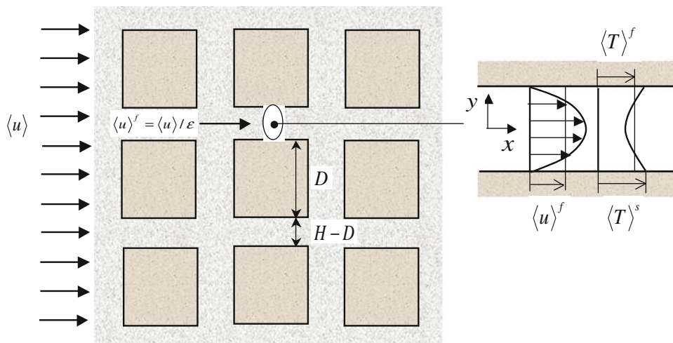
Fig. 2 Model consisting of square tubes for evaluation of the shape factor
