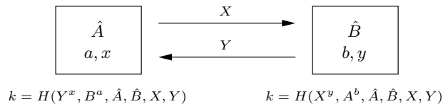
Figure 3: Protocol 3: The variant of Protocol 1 analyzed in [9].
