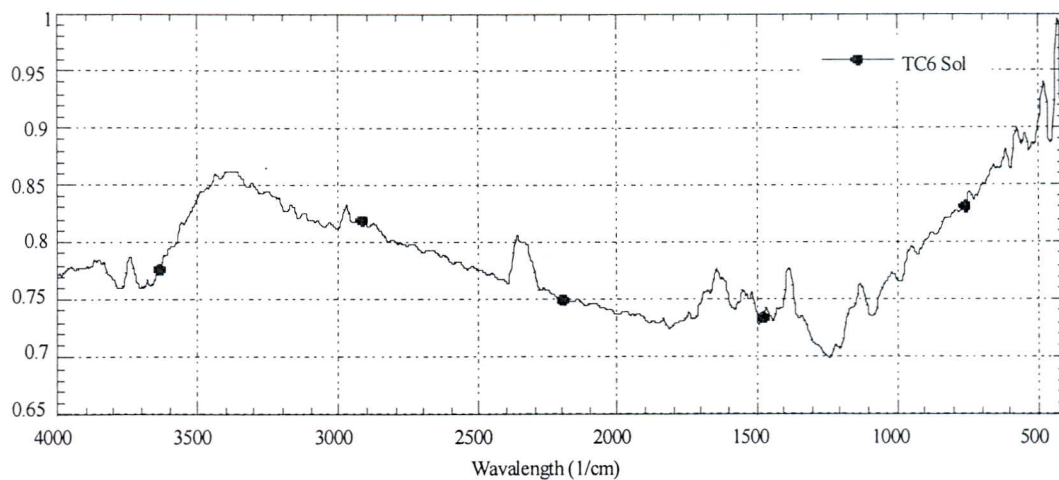
Figure 8.15. FTIR spectrum of TC6 sol.
