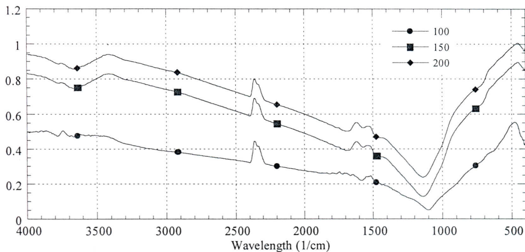
Figure 8.25. FTIR Spectra of TC5 heat treated at 100, 150, 200°C.
