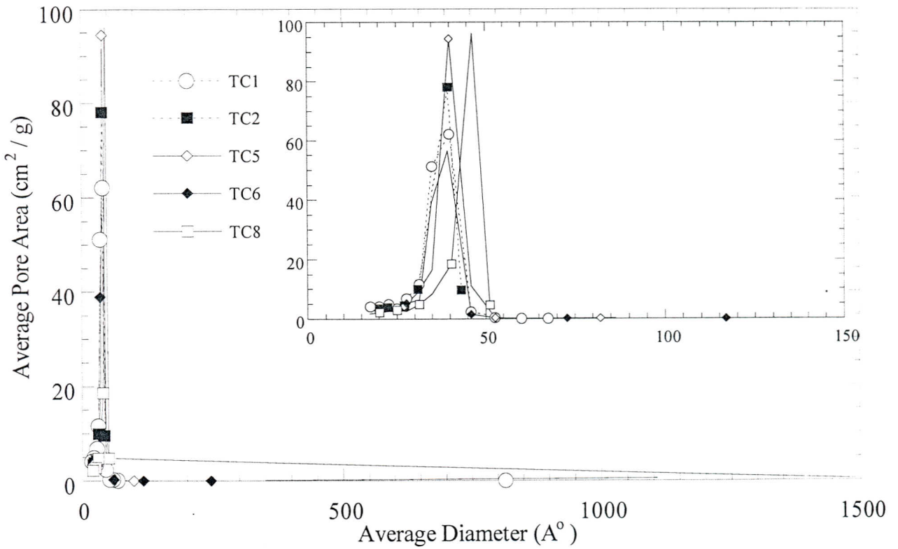
Figure 8.4. The pore area distribution of TC1, TC2, TC5, TC6, and TC8 gels.
