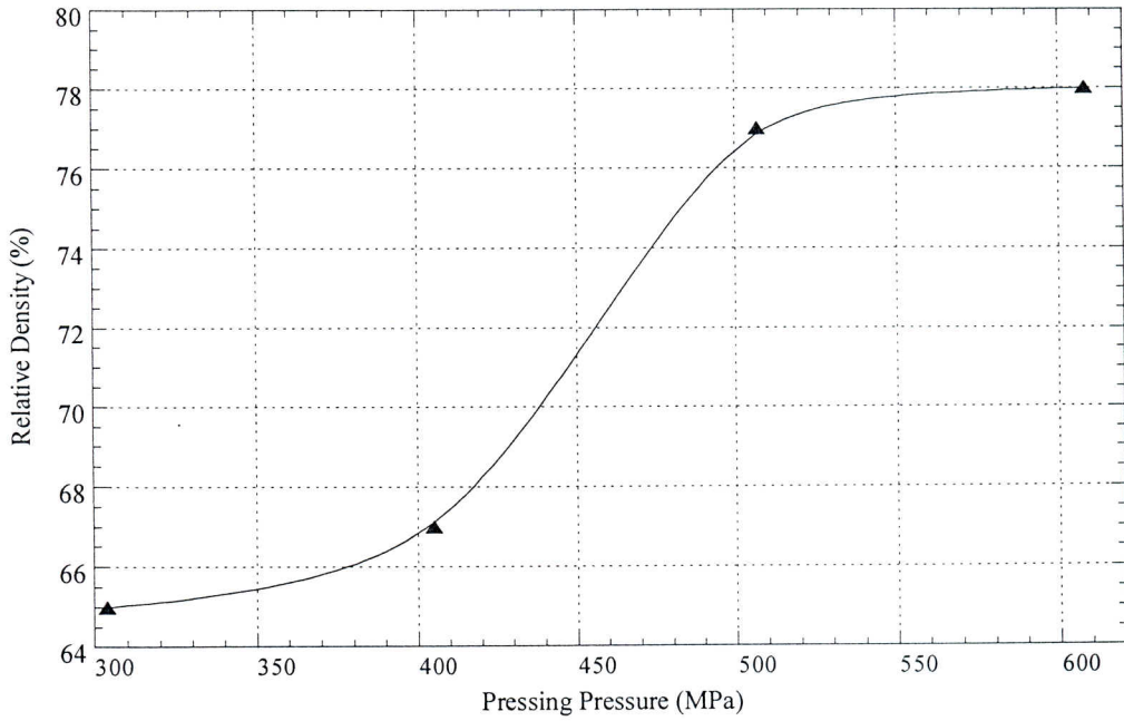
Figure 8.6. The Relative Density versus Pressure Graph of Route 4 (The Sintering Temperature of the Compacts was 700 °C).
