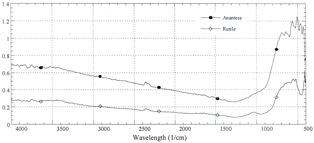
Figure 8.23. FTIR Spectra of commercial anatase and rutile.
