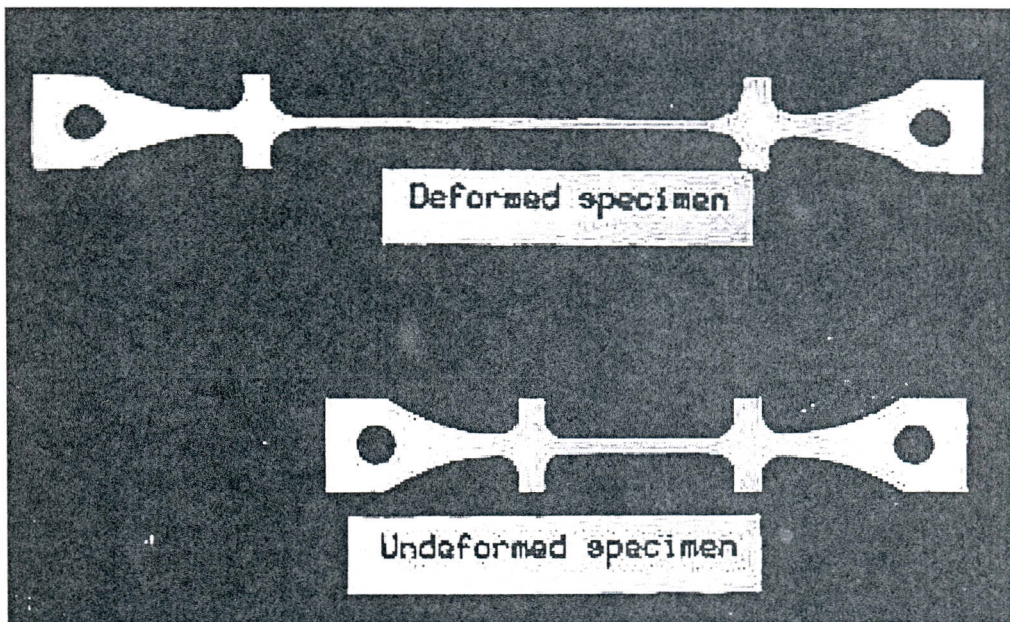
Figure 2.4. Superplastically elongated specimen of Y-TZP at 1450^\circ C .
