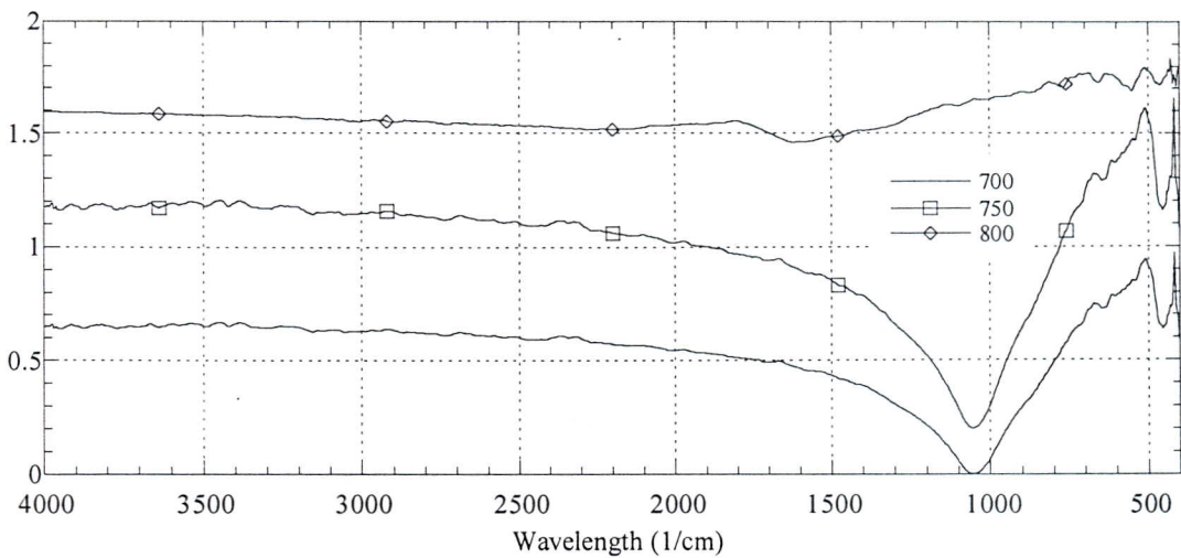
Figure 8.29. FTIR Spectrums of TC5 heat treated at 700, 750, and 800 °C.
