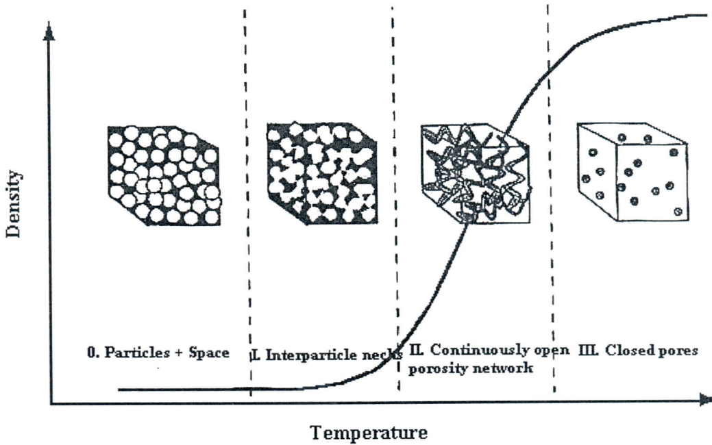
Figure 6.1. Schematic diagram illustrating the three stages of sintering [36].
