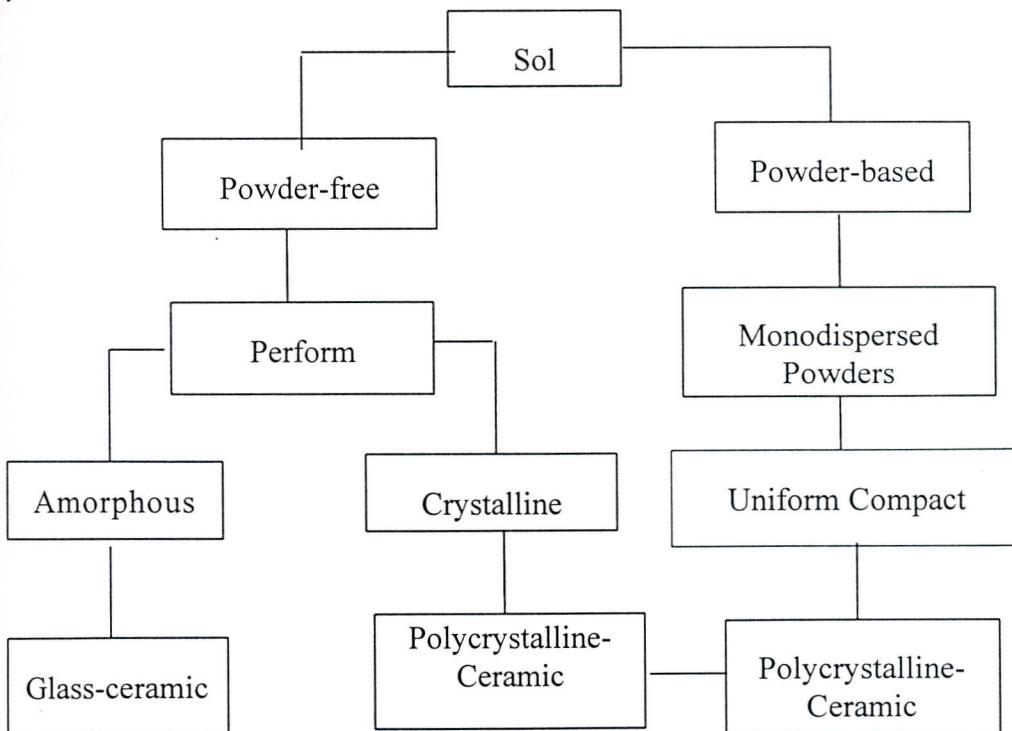
Figure 4.1. Preparation of glass, glass-ceramics, and ceramics by the sol-gel method.
