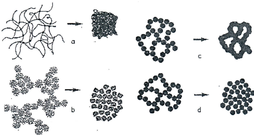
Figure 4.3. Schematic representation of gel desiccation for (a) acid-catalyzed, (b) base-catalyzed gels, (c) colloidal gel aged under conditions of high silica solubility, (d) colloidal gel composed of weakly bonded particles [12].
