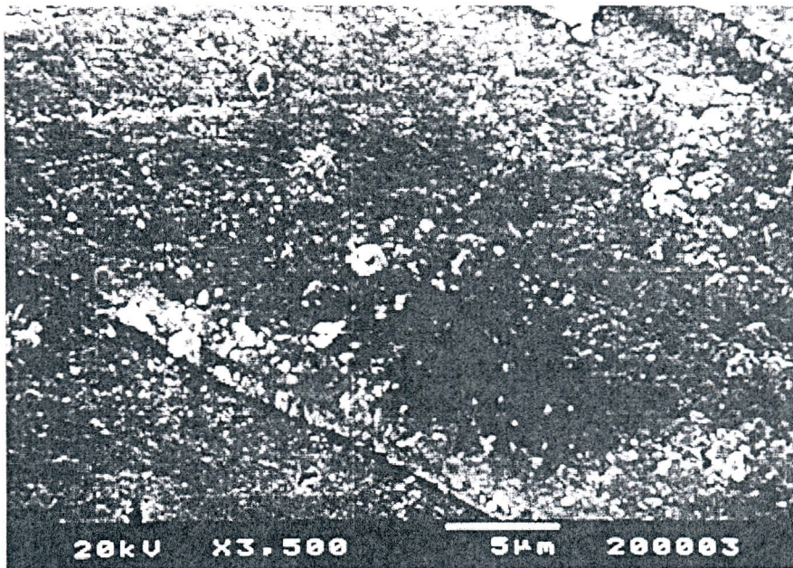
Figure 8.13. The SEM micrograph of TC6 sintered at 700°C at a magification of 3500x.
