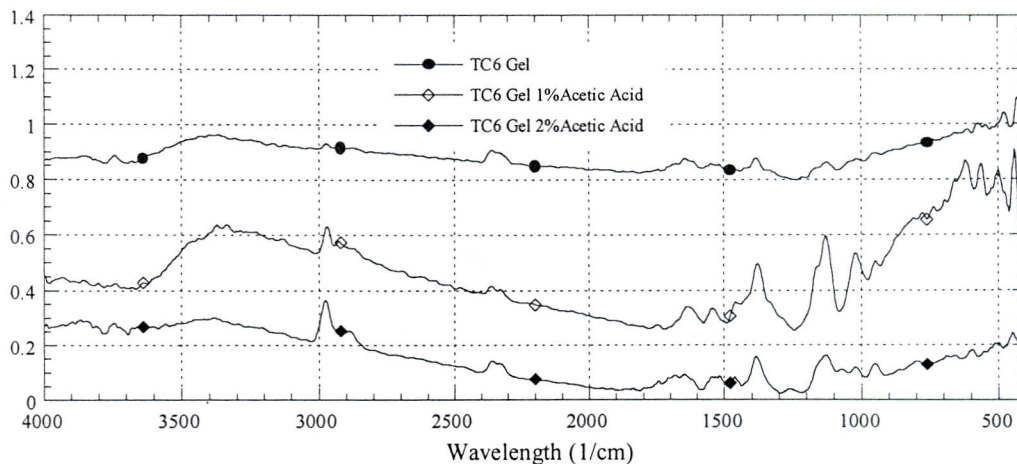
Figure 8.21. FTIR Spectra of TC6 gel and TC6 gels with acetic acid at different ratios.
