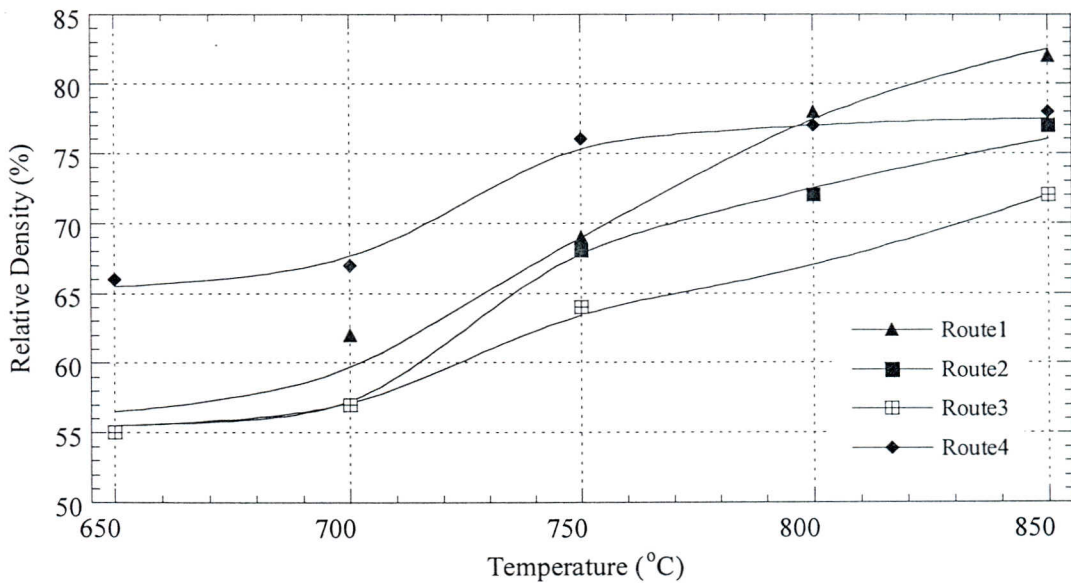
Figure 8.7. The densification behaviour of the pellets produced from Route 2, Route3, Route4, and Route 5.
