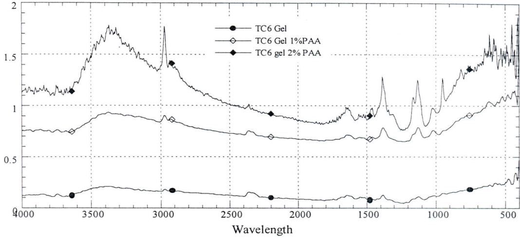
Figure 8.22. FTIR Spectra of TC6 gel and TC6 gels with polyacrylic acid at different ratios.
