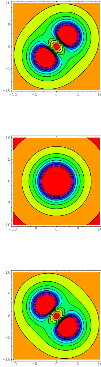
Figure 5.1. N = 2 Vortex Dynamics
