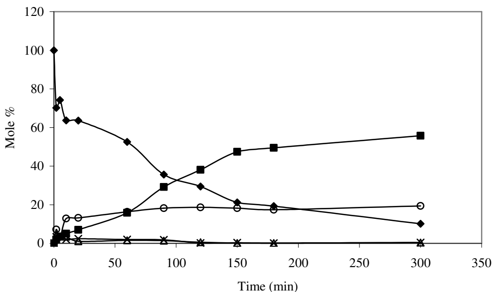
Figure 5.32. Change of acetal formation with respect to reaction time over Ni/MCM-41 catalyst. (◆) Citral; (■) Citronellal; (×) Acetal 1; (Δ) Acetal 2; (○) Acetal 3.
