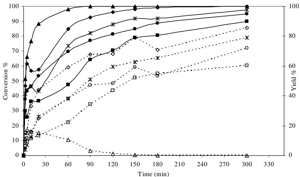
Figure 5.42. Conversion and Yield vs. Time for zeolite supported Ni catalysts: (◆) Ni-NaY Conversion; (▲) Ni/Na-Beta Conversion; (●) Ni/Mordenite Conversion; (■) Ni/MCM-41 Conversion; (✕) Ni/Clinontitolite Conversion; (◇) Ni-NaY Yield; (△) Ni/Beta Yield; (○) Ni/Mordenite Yield; (□) Ni/MCM-41 Yield; (✕) Ni/Clinoptilolite Yield.
