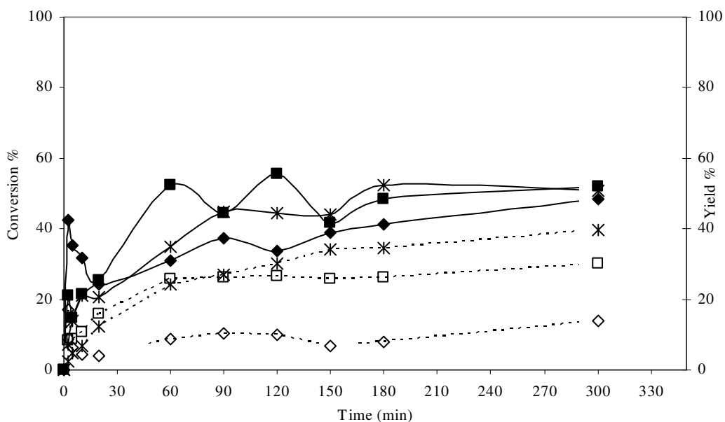
Figure 5.43. Conversion and Yield vs. Time for zeolite supported Pt catalysts: (◆) Pt/NaY Conversion; (■) Pt/MCM-41 Conversion; (✕) Pt/Clinontitolite Conversion; (◇) Pt/NaY Yield; (□) Pt/MCM-41 Yield; (✕) Pt/Clinoptilolite Yield.
