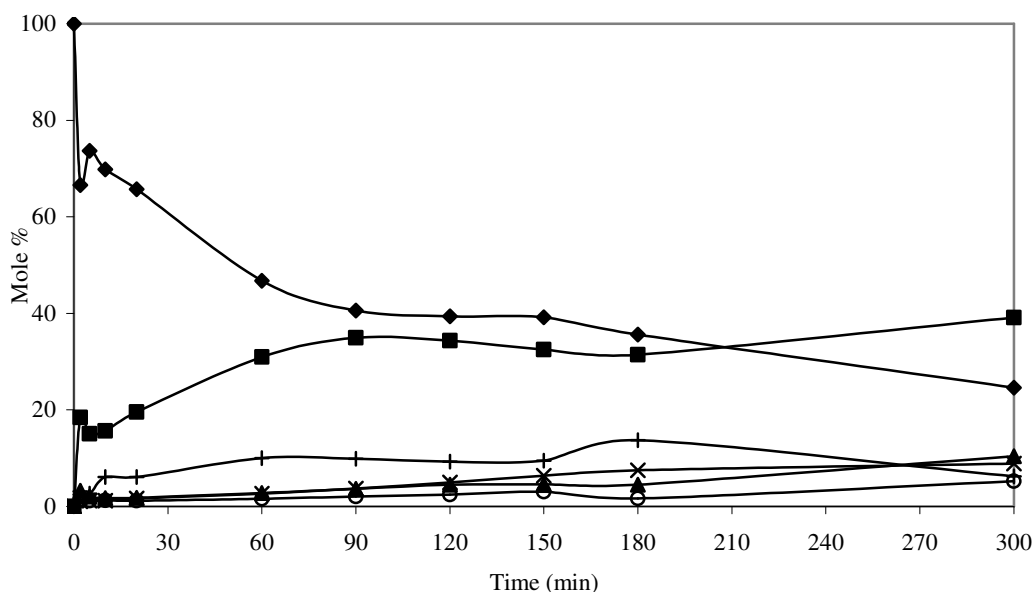
Figure 5.40. Product distribution of citral hydrogenation over Pt-Sn/Clinoptilolite(0.02) catalyst: (◆) Citral; (■) Citronellal; (▲) Citronellol; (×) Nerol; (+) Acetals; (○) Geraniol.
