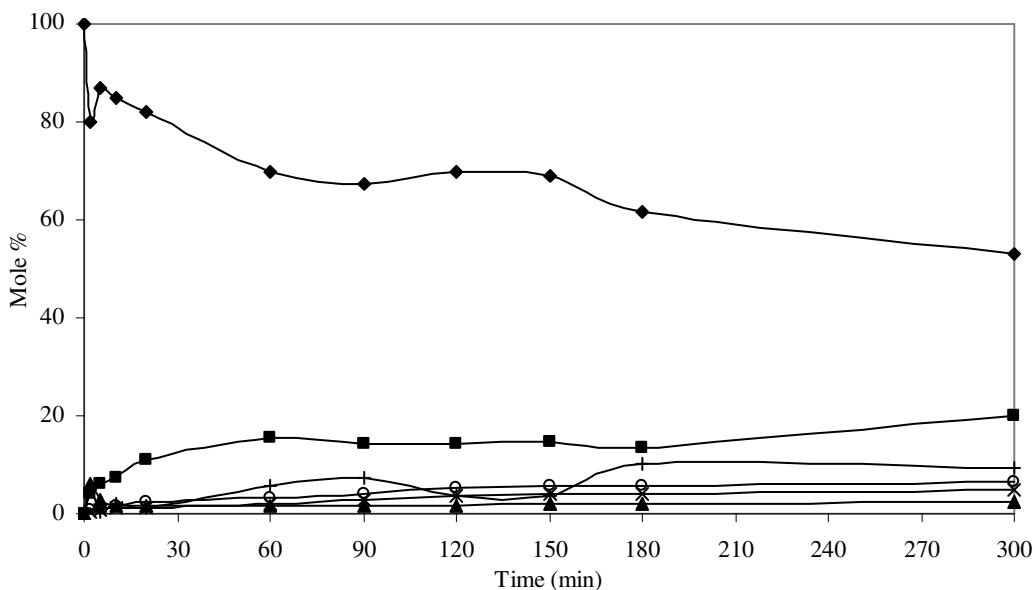
Figure 5.35. Product distribution of citral hydrogenation over monometallic Pt/Na-Y catalyst: (◆) Citral; (■) Citronellal; (▲) Citronellol; (×) Nerol; (+) Acetal; (○) Geraniol.
