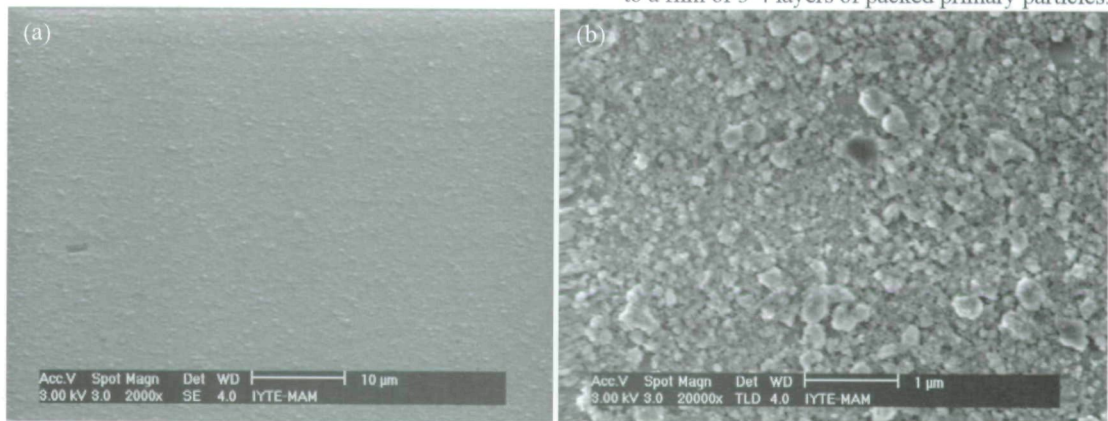
Figure 10. The m-HAp films (with 15% solid content suspension) on glass/sericin substrate at various magnifications (a) 2 000x (b) 20 000x.
