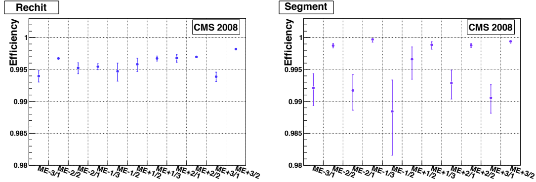
Figure 12. Summaries of rechit and segment efficiencies, analogous to figure 11.
