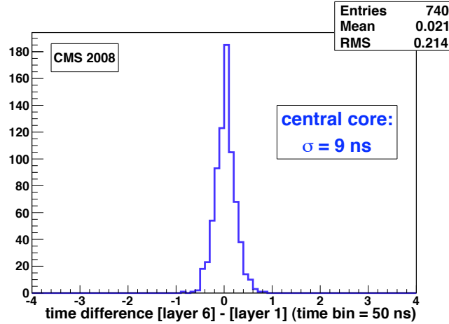
Figure 19. The difference in rechit times for layers 6 and 1 in chamber ME+3/2/9. Units are 50 ns time bins. A fit of the central core to a Gaussian function gives a width of 9 ns.
