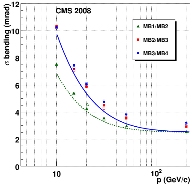
Figure 24. Widths of Gaussian fits to the distributions of the bending angle differences between consecutive stations as a function of the muon momentum. Full points: \mu^+ ; open points: \mu^- . The dashed (full line) curves show the expectation from multiple scattering between MB1-MB2(MB2-MB3 and MB3-MB4) stations, with 2.5 mrad added in quadrature, corresponding to the asymptotic value extracted at high momenta.
