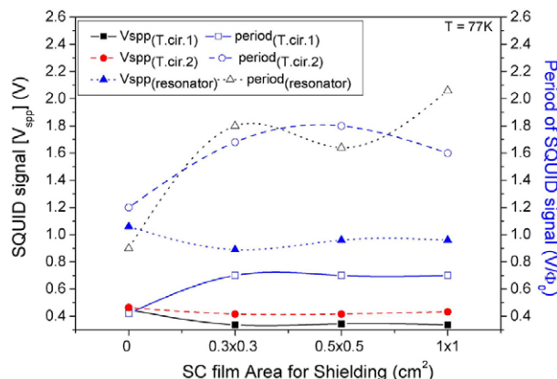
Figure 4. Effect of the applied shield area ( a ). Tank circuits 1 and 2 are conventional LC tank circuits but the loop diameter of the inductor for tank circuit 1 is \sim 0.5 mm and for 2 it is \sim 1 mm. The resonator circuit of the conventional superconducting circular washer type.
