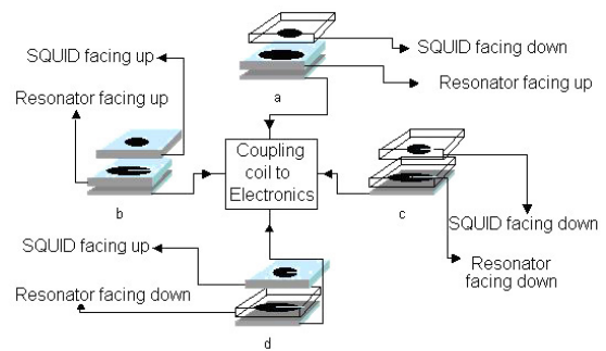
Figure 2. Basic possible configurations for the resonator to rf SQUID coupling.
