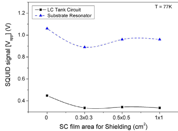
Figure 1. Comparison between the tank circuit and resonator for the rf SQUID signal level under different shielding conditions. A shielding SC film has been applied in the flip chip configuration.
