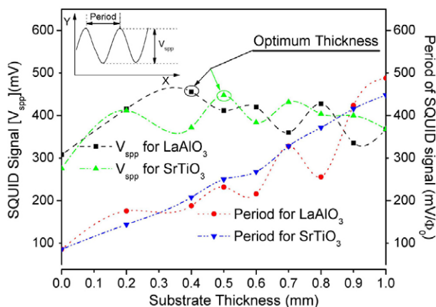
Figure 3. Effect of substrate ( \text{LaAlO}_3 and \text{SrTiO}_3 ) thickness between rf SQUID and LC tank circuit. The inset explains the terms period and V_{\text{spp}} , from the x - y graph where the x -axis represents the input applied modulation flux and the y -axis represents the output of the rf SQUID electronics.
