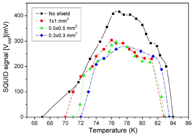
Figure 5. Effect of the temperature on the V_{spp} of the shielded rf SQUID.
