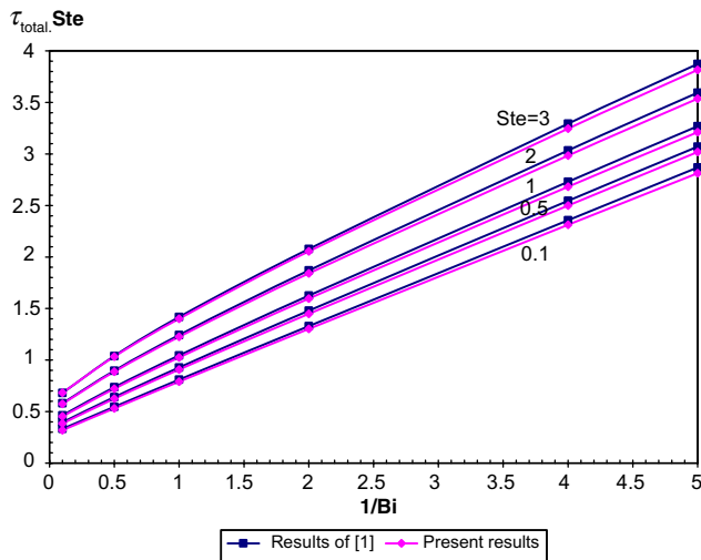
Fig. 4. Comparison of the total solidification time of a cylinder with Ref. [1].
