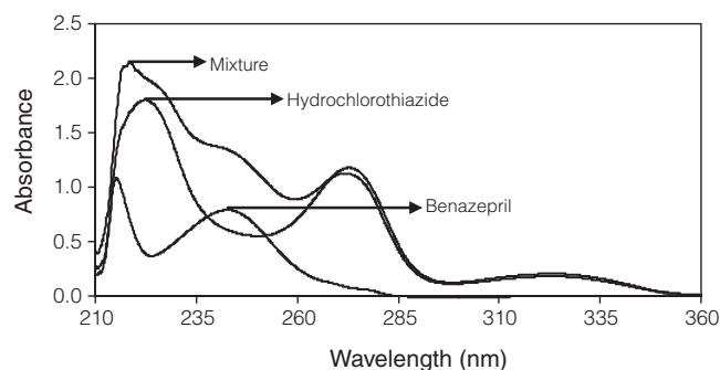
Figure 1. UV spectra of benazepril (36 \mu\text{g}/\text{mL} ) and hydrochlorothiazide (22 \mu\text{g}/\text{mL} ) along with a binary mixture of the two components between 220 and 360 nm wavelength range.
