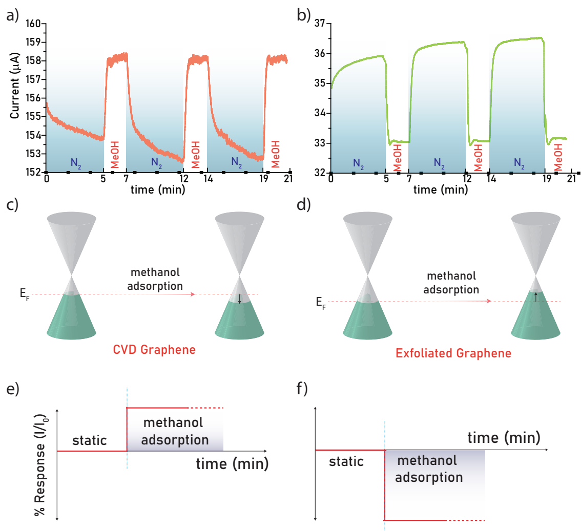
Figure 4.4. Effect of exposure to methanol gas on the normalized current of a) CVD graphene and b) exfoliated graphene chemiresistors. Doping level change of c) CVD and d) exfoliated graphene upon exposure to methanol. d) Change of electrical response read on e) CVD and f) exfoliated graphene sensor device due to methanol adsorption.
