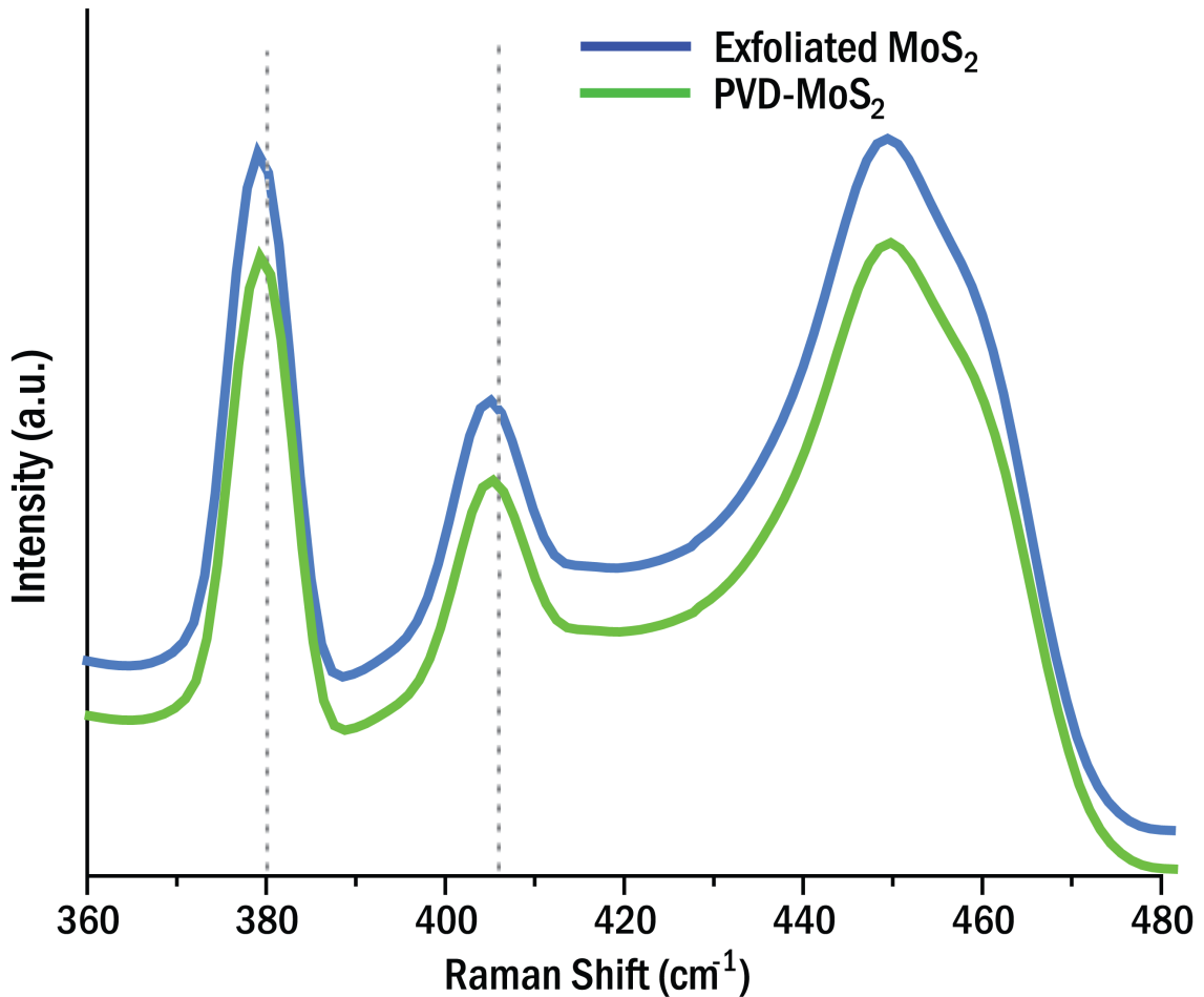
Figure 2.3. Raman spectra of mechanically exfoliated and Physical Vapor Deposited (PVD) MoS 2 , excited with 785 nm light source.
