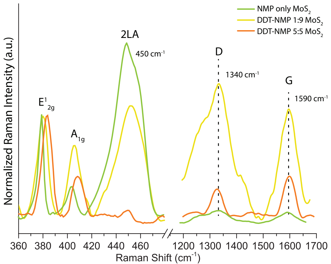
Figure 3.5. The Raman spectra of NMP-MoS 2 and different ratios of DDT-NMP of DDT-MoS 2 functionalized samples on Si/SiO 2 substrates.
