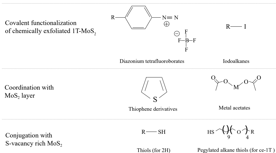
Figure 1.2. Correlation of utilized chemicals and manners of functionalization of TMDs.
