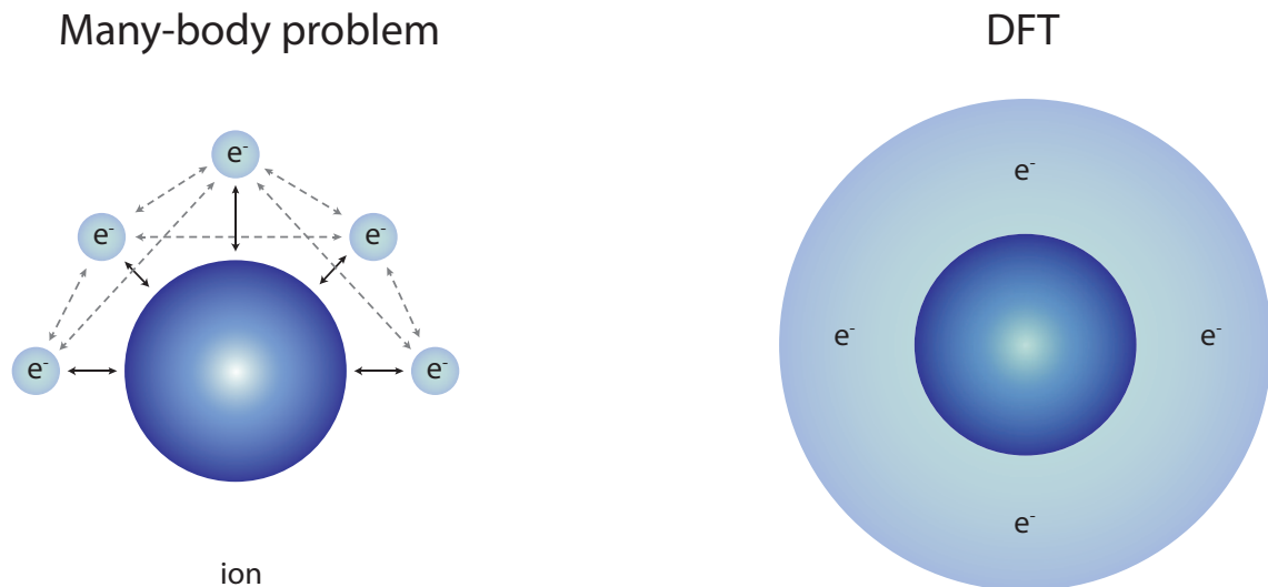
Figure 2.7. Illustration of the many-body interaction problem being addressed by Density Functional Theory (DFT). DFT tackles the complex interactions among electrons in a system by mapping it onto an effective single-particle problem governed by the exchange-correlation functional, enabling the calculation of properties such as electronic structure and energies.
