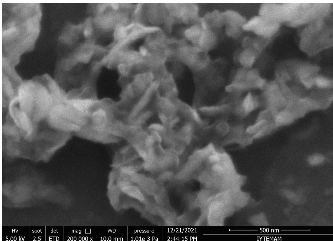
Figure 2.5. The captured Scanning Electron Microscopy (SEM) images of DDT-functionalized MoS 2 (DDT-MoS 2 ) samples on Si/SiO 2 .
