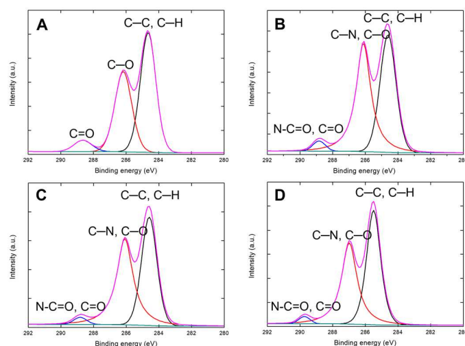
Fig. 4. C1s narrow region XPS spectra of PCL and peptide-conjugated PCL membranes A. PCL, B. PPGCYNTQALEQQ, C. PPGCYNTQALEDDQ, D. PPGCYNTQALEDDQ conjugated membranes
