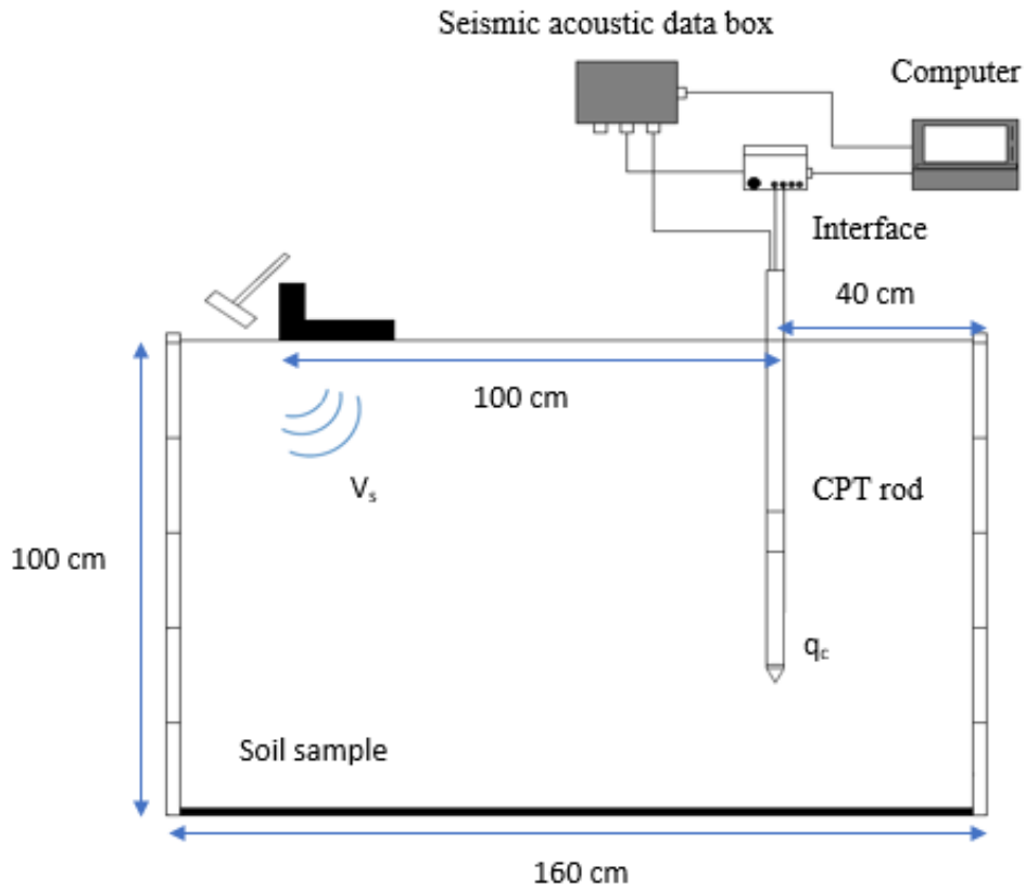
Figure 4.1. Schematic view of SCPT experiments
