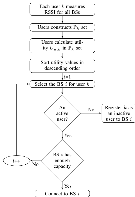
Fig. 1. Flowchart of load based full set cell selection algorithm
