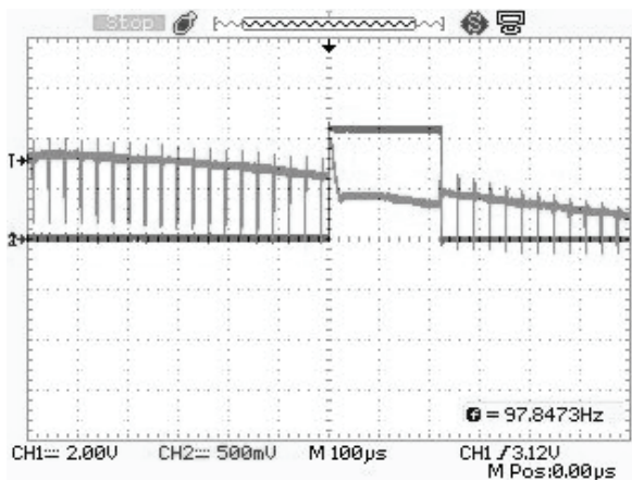
Figure 5.7. Window scale divider is 2 in coasting sense mode.
