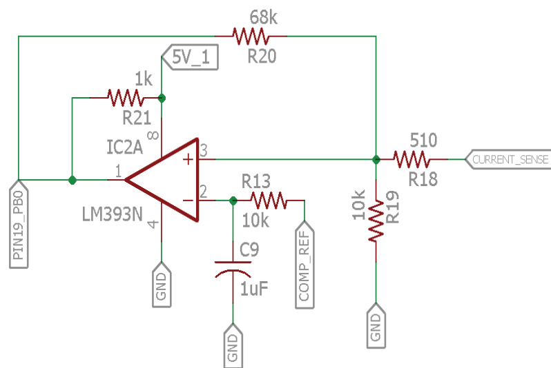
Figure 3.7. Inductive sense circuit.
