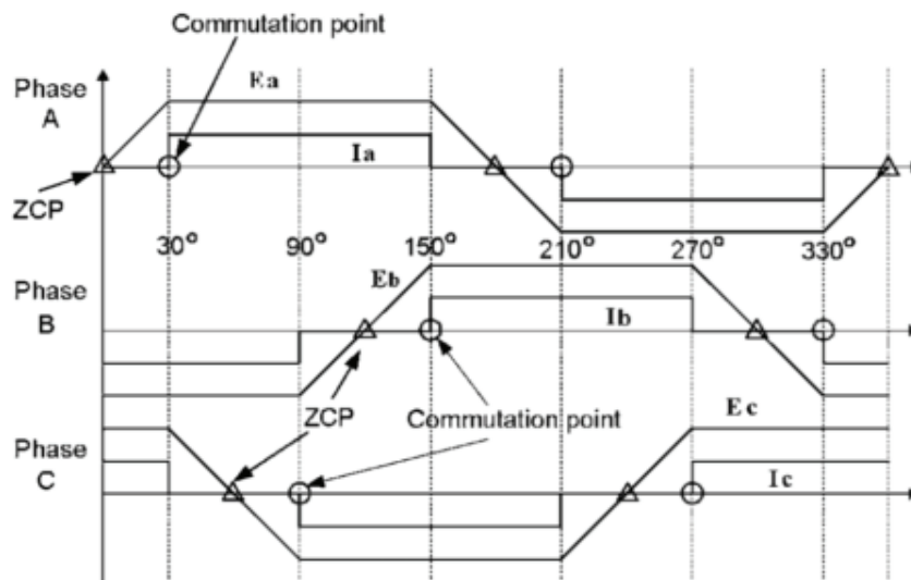
Figure 2.5. Zero cross and commutation points on BEMF signal.
