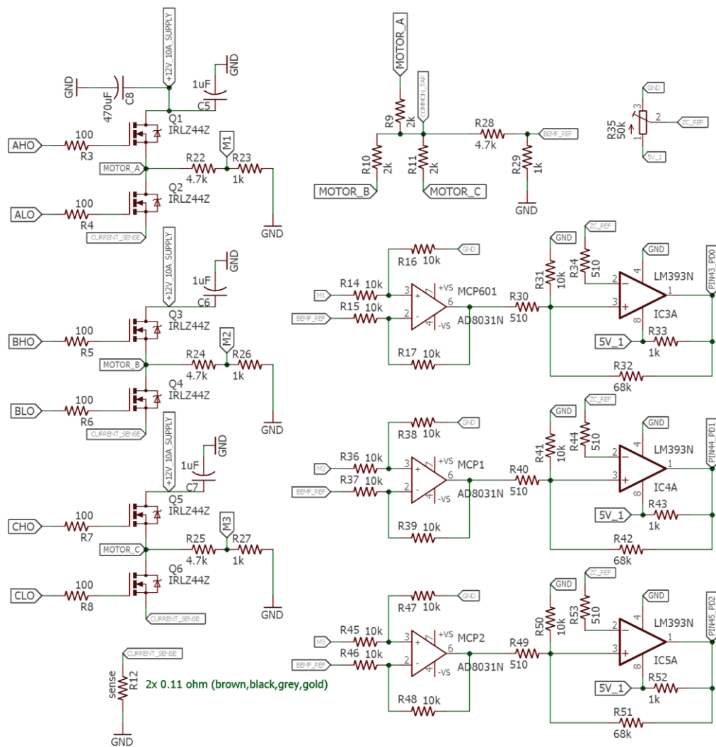
Figure 3.6. BEMF detection circuit.
