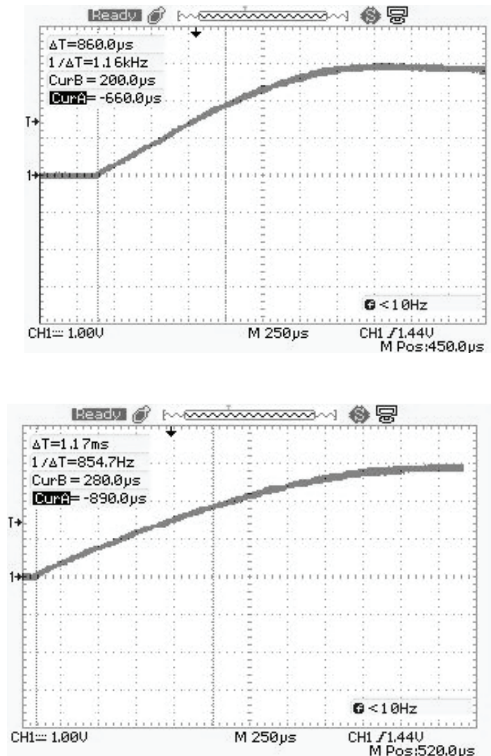
Figure 3.8. Oscilloscope captures of the inductive sense current waveforms; Top: rotor is aligned with the excitation step, Bottom: rotor position is opposite to the applied step.
