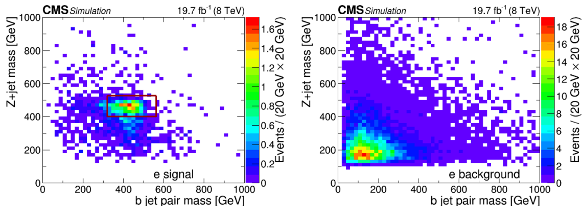
Figure 3. Distributions of Z+jet mass versus b jet pair mass for signal events with m_{G'} = 1100 GeV and m_{\Theta^0} = 478 GeV (left) and background events (right), in the electron channel (distributions are similar in the muon channel). The open red rectangle on left indicates the signal region, as described in the text.
