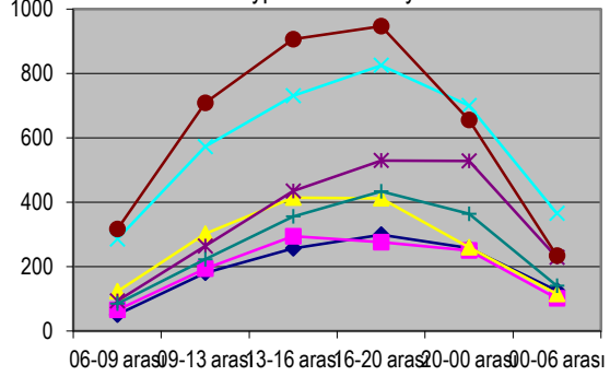
Figure 6. Average Hourly Traffic Flows by Hour Types for Sundays
