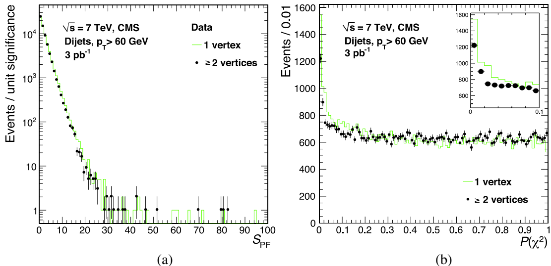
Figure 22. Distributions of the \cancel{E}_T significance (left) and \mathcal{P}(\chi^2) (right) for events with a single interaction vertex (histogram) and multiple interaction vertices (points) in the 60 GeV threshold dijet sample. The inset expands the small \mathcal{P}(\chi^2) region.
