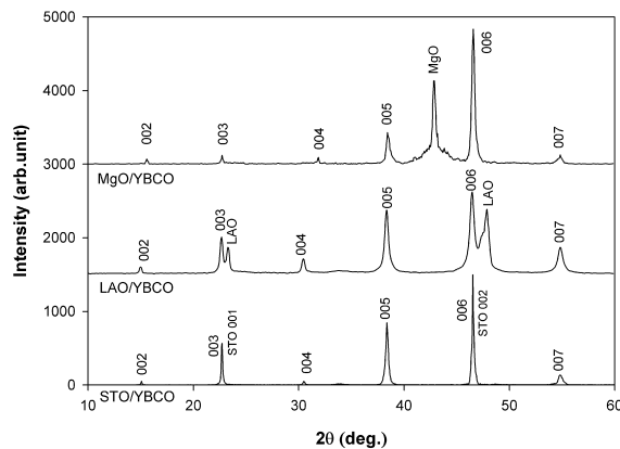
Fig. 3. XRD analysis of YBCO thin films on different substrates.
