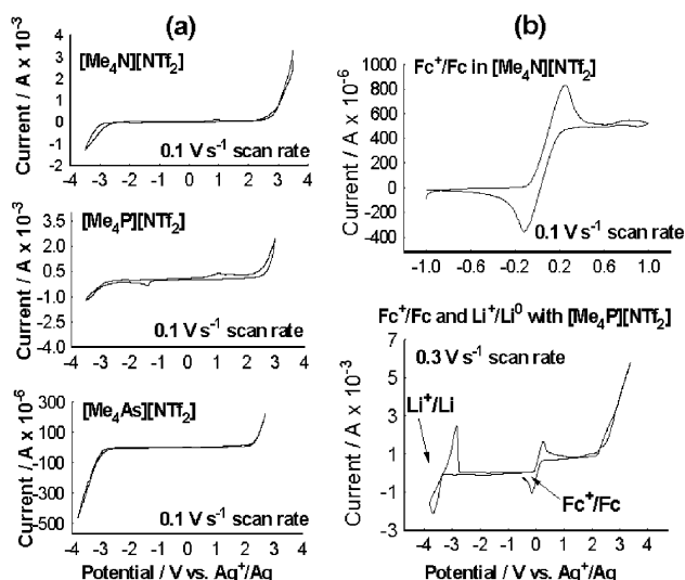
Fig. 1 (a) Cyclic voltammograms of 0.2 mol L -1 [(Me 4 X)N(SO 2 CF 3 ) 2 ] salts in MeCN and (b) cyclic voltammograms of ferrocene and Li[N(SO 2 CF 3 ) 2 ] in MeCN with 0.2 mol L -1 [(Me 4 X)N(SO 2 CF 3 ) 2 ] salts as supporting electrolyte. Note: [NTf 2 ] = [N(SO 2 CF 3 ) 2 ].
