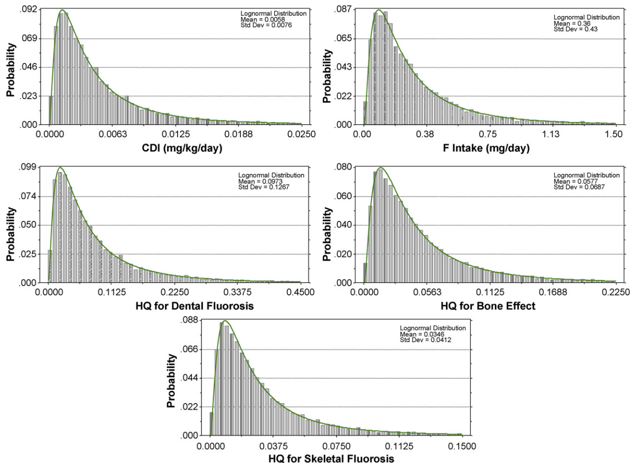
Fig. 2. Population CDI, intake, and HQ distributions for fluoride.
