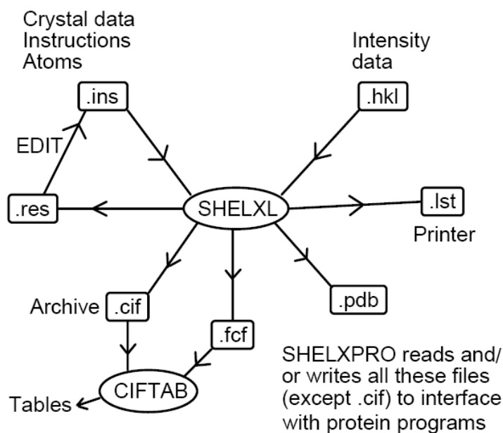
Figure 4.2. Schematic diagram of SHELX program.
