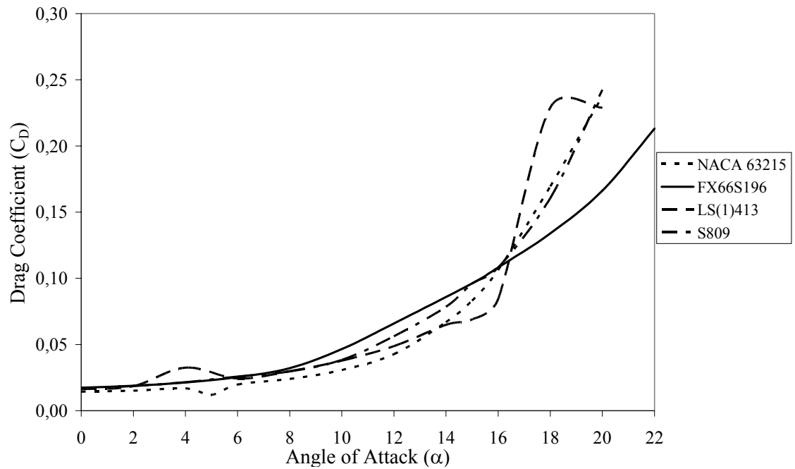
Figure 7.6. Drag coefficients versus angle of attack for Re=5.5e05 .
