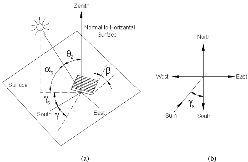
Figure 5. 2. (a) Zenith angle, slope, surface azimuth angle, and solar azimuth angle for a tilted surface. (b) Plan view showing solar azimuth angle (modified from Duffie and Beckman 1991)
