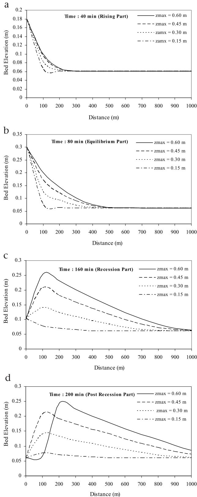
Figure 5. (a) Transient bed profile under different z_{\max} values at rising period of inflow hydrograph and concentration. (b) Transient bed profile under different z_{\max} values at equilibrium period of inflow hydrograph and concentration. (c) Transient bed profile under different z_{\max} values at recession period of inflow hydrograph and concentration. (d) Transient bed profile under different z_{\max} values at postrecession period of inflow hydrograph and concentration.
