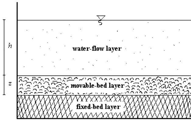
Figure 1. Schematic representation of two-layer system.
