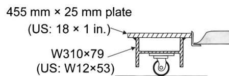
Fig. 6. Cross section of beams from shear frame
