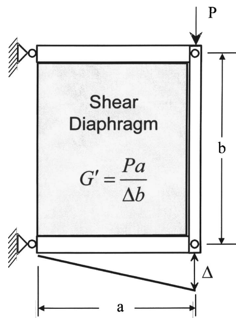
Fig. 3. Cantilever shear frame
