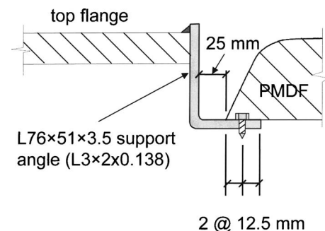
Fig. 8. Support angle-PMDF connection
