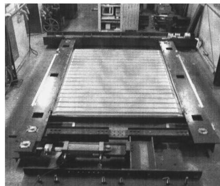
Fig. 5. Test setup for shear tests
