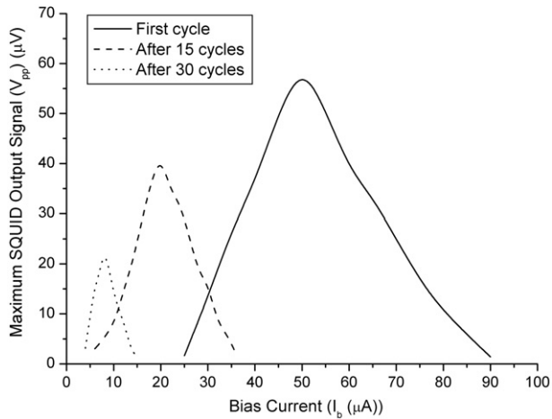
Figure 4. Bias current dependence of unprotected DC-SQUID output voltages during the thermal cycles. Bias current versus V_{pp} dependence showed a single peak in all measurements with reduced current values as well as the maximum peak-to-peak voltage values.
