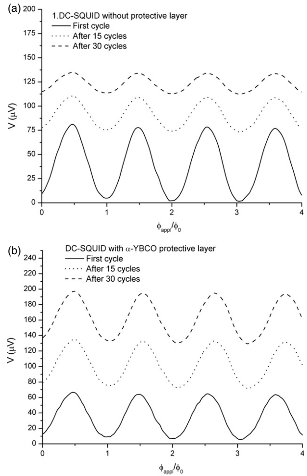
Figure 3. Output signals of the DC-SQUIDS depending on the thermal cycles. The curves are shifted vertically for clarity. (a) Unprotected DC-SQUID, (b) DC-SQUID with 400 nm thick amorphous YBCO layer. Solid, dotted and dashed lines represent the measurements for the first, 15th and 30th thermal cycles, respectively. The SQUIDS were modulated by a three-turn feedback coil by applying 20 Hz AC signal with 1.5 V_{pp} .
