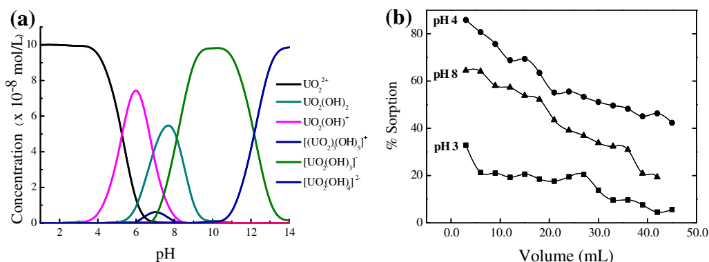
Fig. 5. (a) Speciation diagram of U(VI) and (b) microcolumn study of U(VI) at different pH values. Reaction conditions: initial U(VI) concentration of 100 µg L -1 , 0.15 mL min -1 flow rate, 25.0 mg sorbent.
