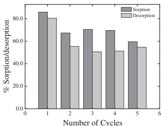
Fig. 9. Consecutive sorption/desorption cycles of amidoximated PAN fiber for 100 \mu\text{g L}^{-1} U(VI) solution using 0.5 \text{ M} \text{NaHCO}_3 as the desorbing agent.
