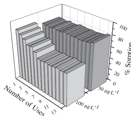
Fig. 7. Variation of percent sorption of uranyl ion with the number of repetitive usages of the same fiber sorbent at the initial U(VI) concentrations of 50 µg L -1 and 100 µg L -1 . Reaction conditions: 3.0 mL sample volume, 0.15 mL·min -1 flow rate, 25.0 mg sorbent, pH 4.0.
