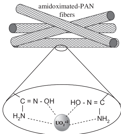
Scheme 2. Speculative binding mechanism.
