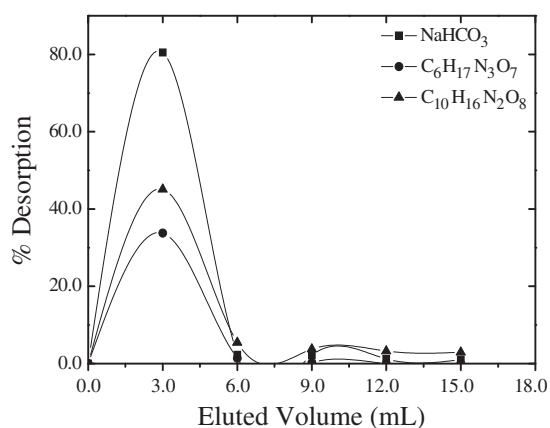
Fig. 8. Uranyl ion desorption as a function of eluted volume. Reaction conditions: initial U(VI) concentration of 100 \mu\text{g L}^{-1} , 0.15 \text{ mL}\cdot\text{min}^{-1} flow rate, 25.0 \text{ mg} sorbent.
