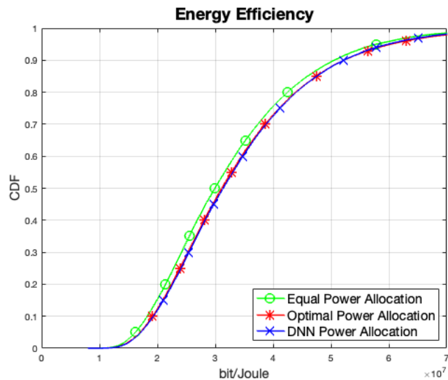
Figure 3.9. Energy efficiency of DNN for power allocation using Algorithm 2, for K=4 , L=9 , N=4 .
