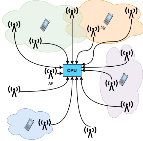
Figure 2.1. Representation of User-Centric Clustering.
