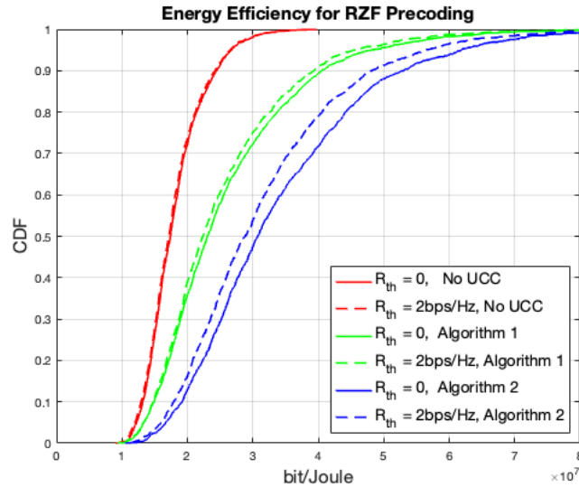
Figure 2.10. Effect of data rate constraints on the performance using RZF precoding, for K=4 , L=9 , N=4 .
