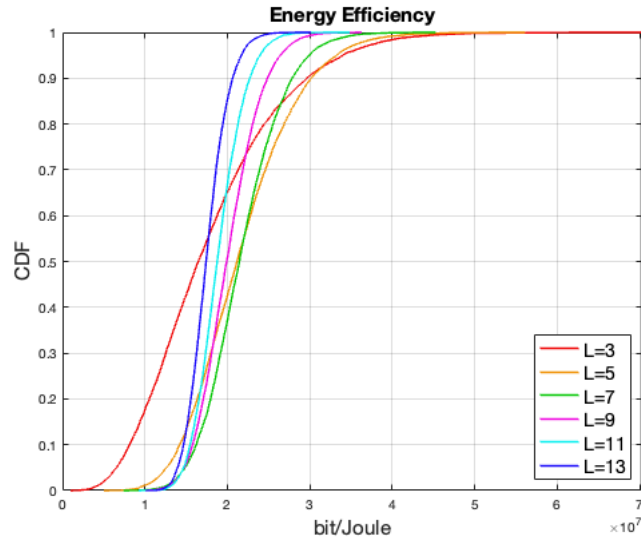
Figure 2.5. CDF of energy efficiency for different number of APs, for K=7 and N=4 .
