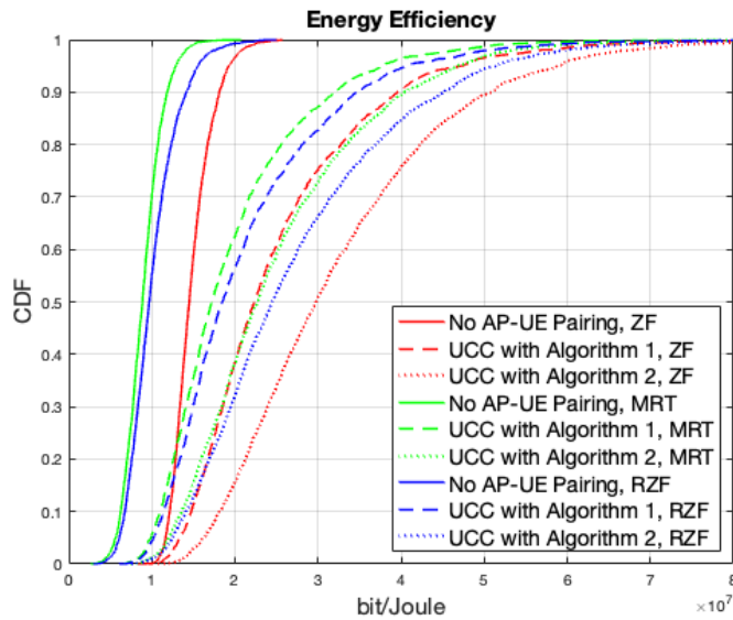
Figure 2.13. Energy efficiency comparison for different user-centric clustering algorithms and precoding schemes, for L=9 , K=4 , N=4 .
