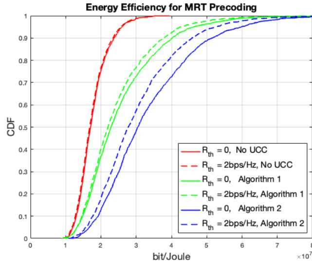
Figure 2.12. Effect of data rate constraints on the performance using MRT precoding, for K=4 , L=9 , N=4 .
