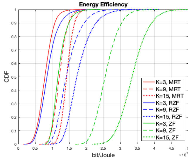
Figure 2.6. Precoding performance comparison for different number of UEs, for L=9 and N=4 .
