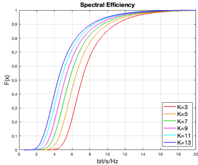
Figure 2.3. CDF of spectral efficiency for different number of UEs, for L=9 and N = 4 .
