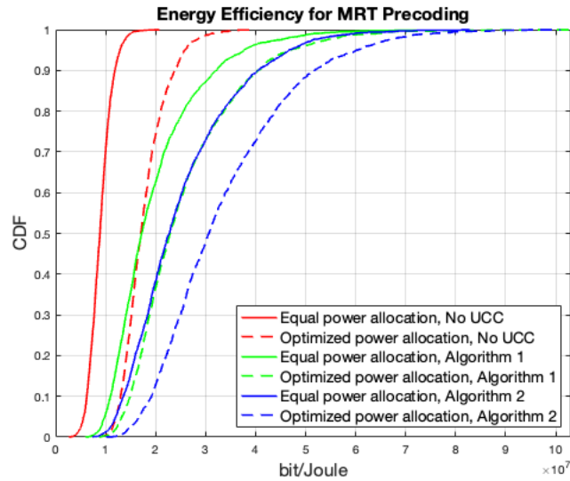
Figure 2.11. Energy efficiency of MRT precoding for equal and optimized power allocations, for K=4 , L=9 , N=4 .
