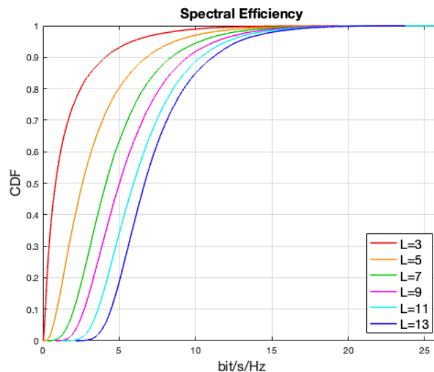
Figure 2.2. CDF of spectral efficiency for different number of APs, for K=7 and N = 4 .
