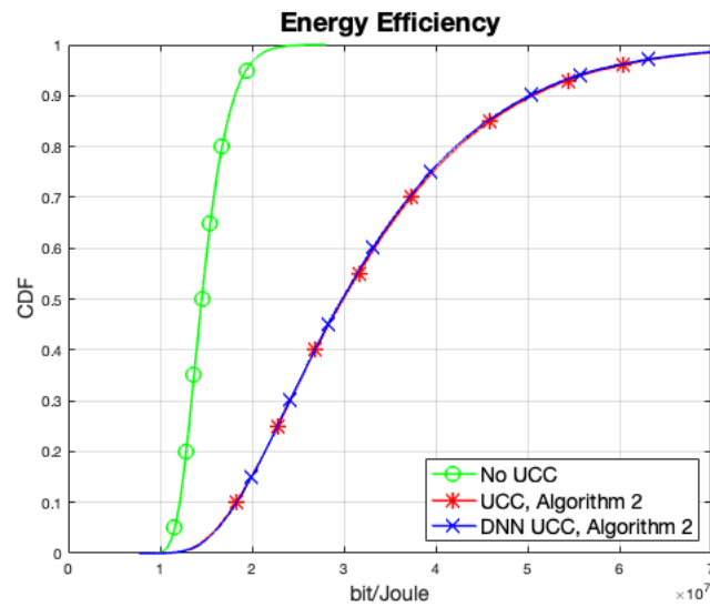
Figure 3.7. Energy efficiency performance of DNN based user-centric clustering using the Algorithm 2, for K=4 , L=9 , N=4 .
