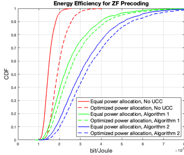
Figure 2.7. Energy efficiency of ZF precoding for equal and optimized power allocations, for K=4 , L=9 , N=4 .
