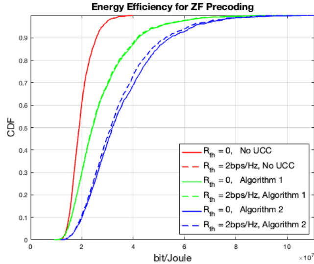
Figure 2.8. Effect of data rate constraints on the performance using ZF precoding, for K=4 , L=9 , N=4 .
