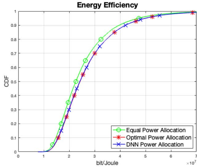
Figure 3.8. Energy efficiency of the DNN for power allocation using Algorithm 1, for K=4 , L=9 , N=4 .
