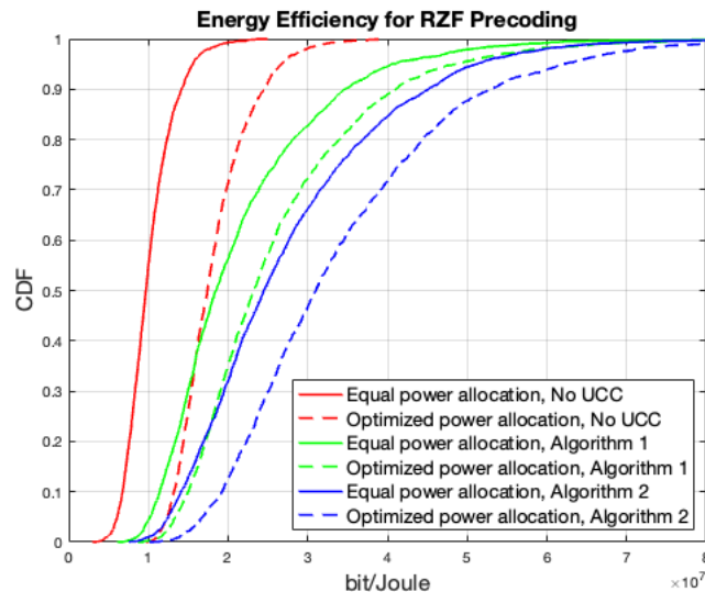
Figure 2.9. Energy efficiency of RZF precoding for equal and optimized power allocations, for K=4 , L=9 , N=4 .
