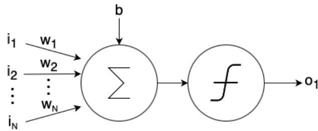
Figure 3.1. Visualization of a neuron.
