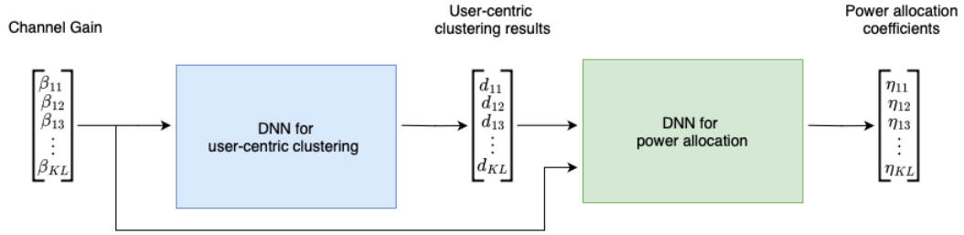
Figure 3.5. Block diagram of the proposed machine learning based resource allocation approach for cell-free massive MIMO systems.
