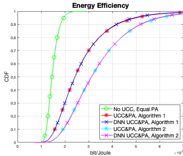
Figure 3.10. Energy efficiency of DNN for joint power allocation and user-centric clustering, for K=4 , L=9 , N=4 .
