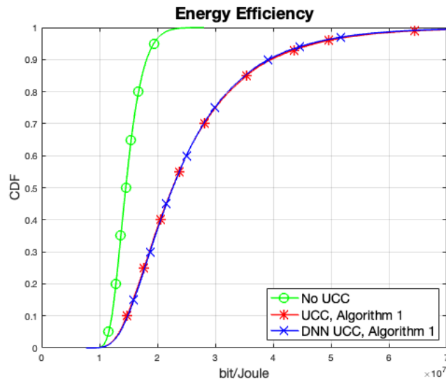
Figure 3.6. Energy efficiency of DNN based user-centric clustering using Algorithm 1, for K=4 , L=9 , N=4 .
