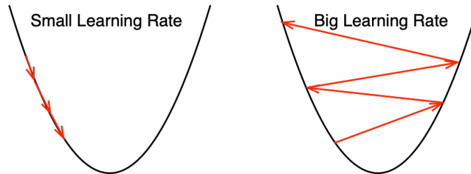
Figure 3.3. Effect of the learning rate.
