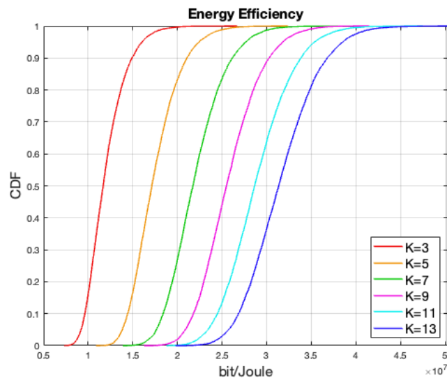
Figure 2.4. CDF of energy efficiency for different number of UEs, for L=9 and N=4 .
