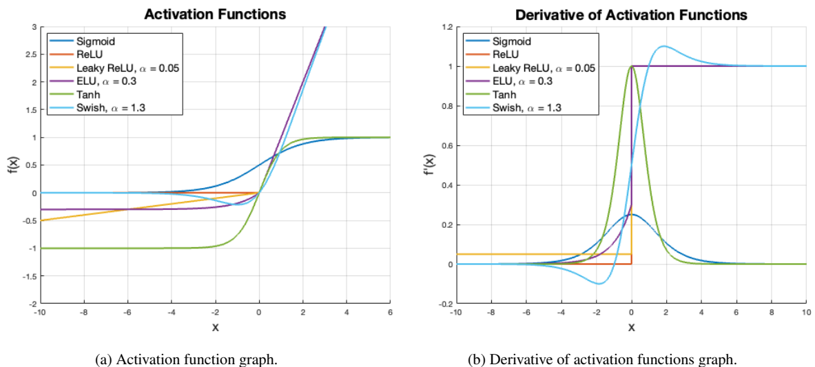
Figure 3.4. Activation Functions.
