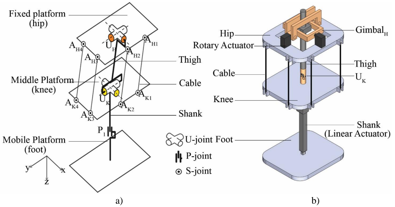
Figure 3. The second conceptual design: a) the kinematic structure, b) the CAD model
