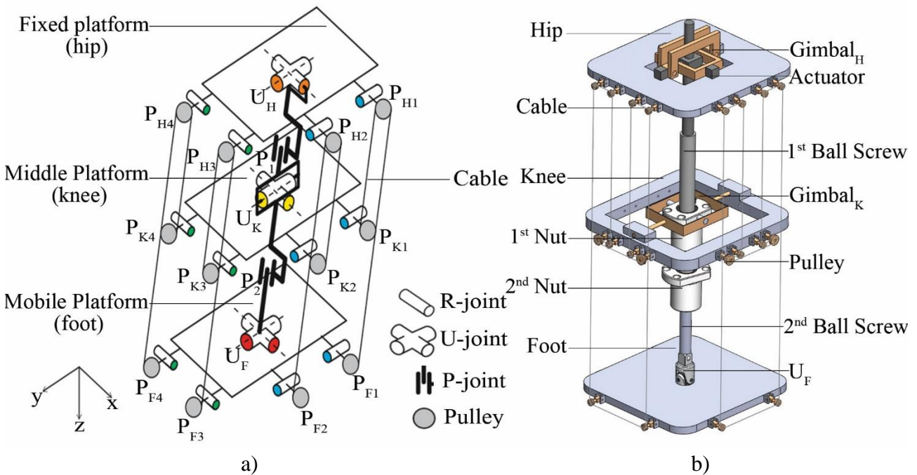
Figure 1. The first conceptual design: a) the kinematic structure, b) the CAD model
