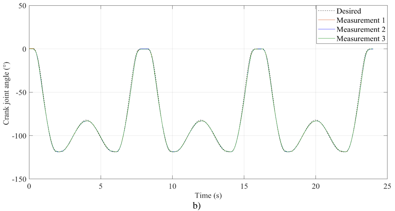
Figure 11. Desired and measured angular displacements of the actuated, a) hip joint ( \theta_{H1} ), b) slider-crank linkage ( \theta_S )
