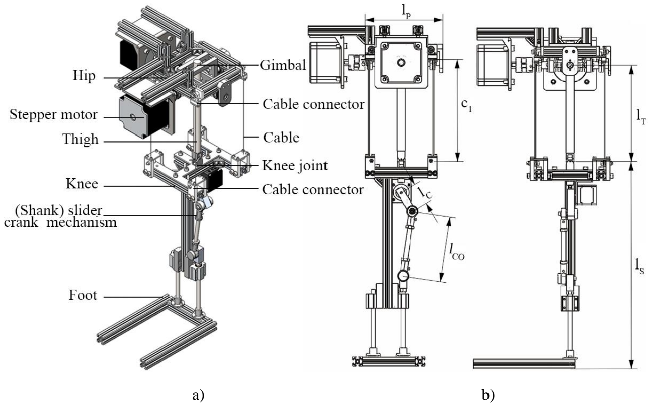
Figure 6. Design and dimension parameters of the leg mechanism: a) the CAD model, b) design parameters
