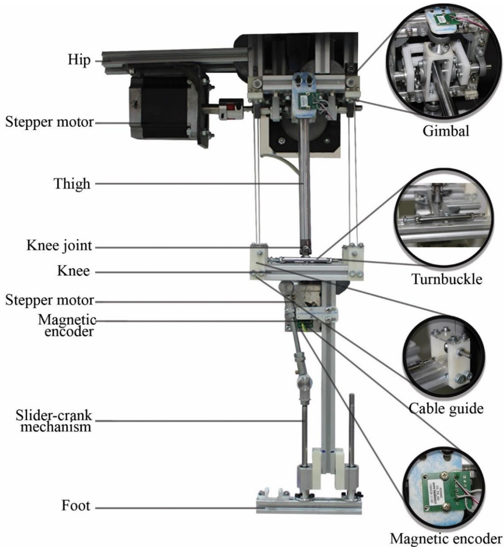
Figure 7. The built prototype of the leg mechanism for validation tests
