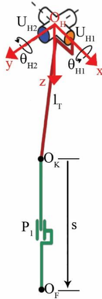
Figure 5. Simplified kinematic model with link and joint parameters
