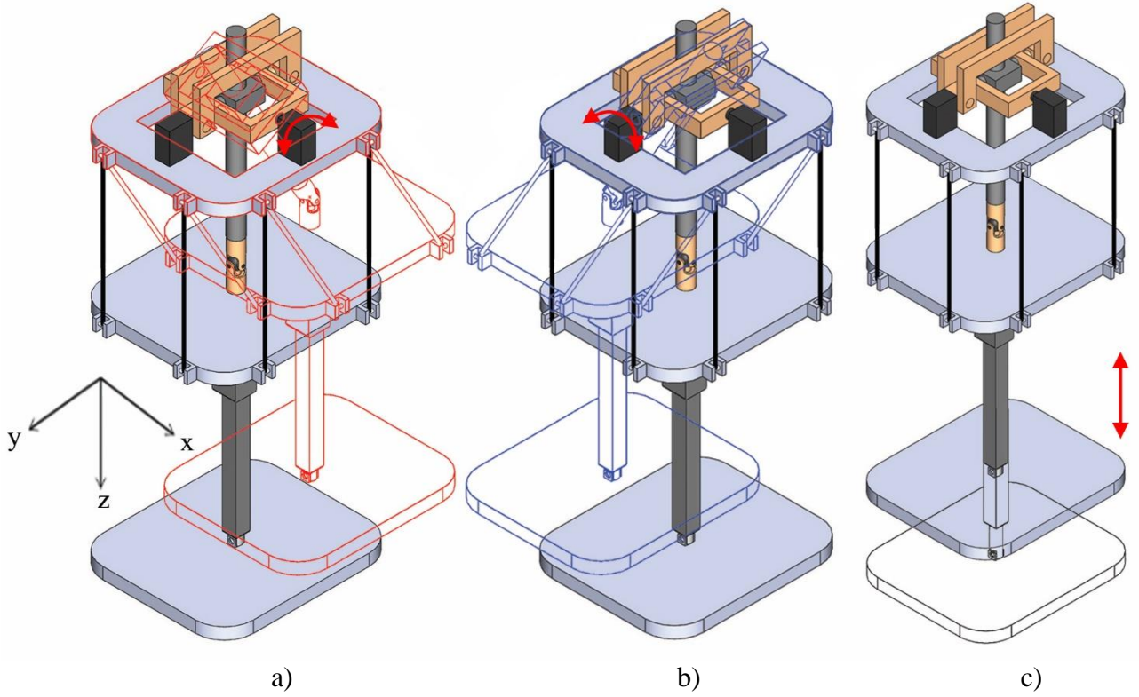
Figure 4. Snapshots of independent motions of the leg mechanism with corresponding actuation inputs: a) \theta_{H1} = 30^\circ , b) \theta_{H2} = -30^\circ , c) s = 50 mm
