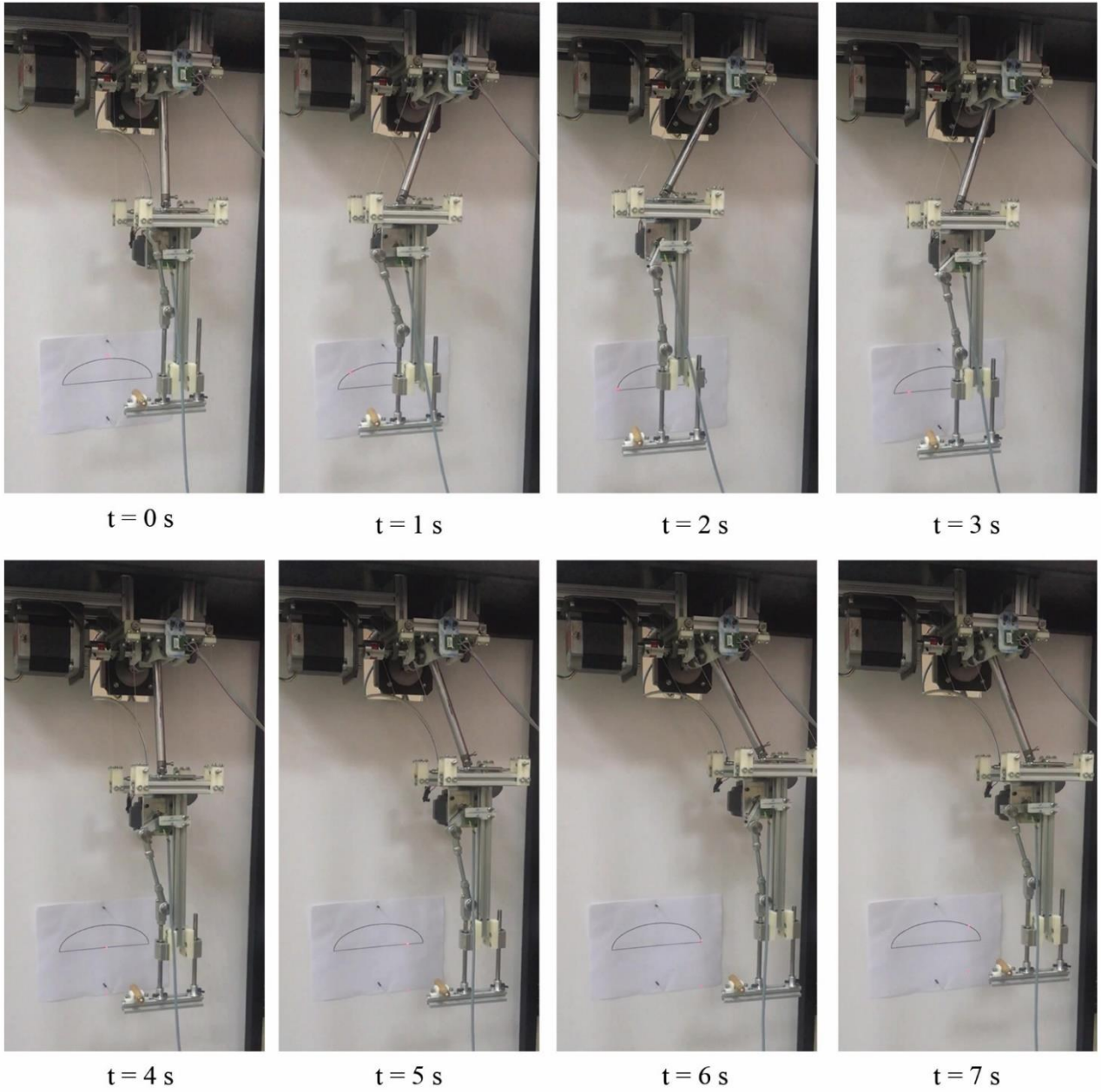
Figure 10. Snapshots of a validation test using the test setup in Fig. 9
