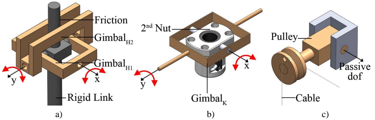
Figure 2. Details of the conceptual design: a) \text{Gimbal}_H , b) \text{Gimbal}_K , c) pulley
