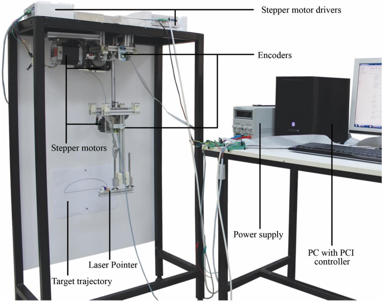
Figure 8. Experimental setup of the leg mechanism prototype in Fig. 7
