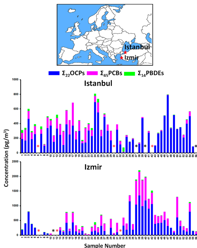
Figure 1. Total concentration of \Sigma_{22} OCPs, \Sigma_{45} PCBs, and \Sigma_{14} PBDEs in (a) Istanbul and (b) Izmir (details of sampling are given in SI Tables S2 and S3) (red *no data due to instrument malfunction; *data < MDL).
