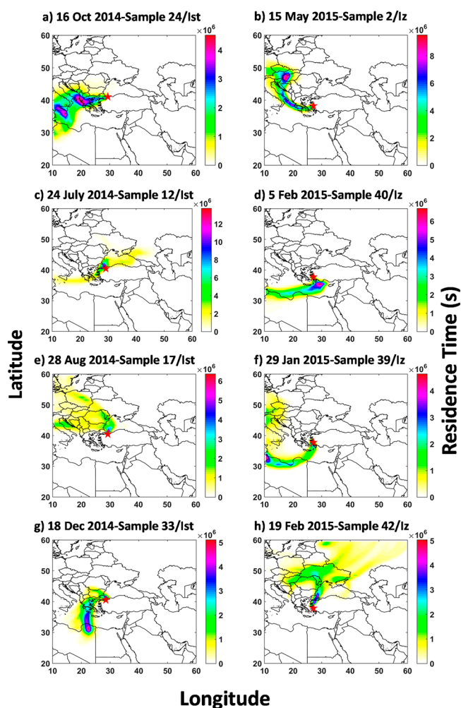
Figure 2. Residence times of air masses received at Istanbul and Izmir stations for the samples with >95th percentile (a,b) \sum DDX, (c,d) \sum HCH, (e,f) \sum_{45} PCBs, and (g,h) \sum_{14} PBDEs gas-phase concentrations (red stars indicate the sampling locations).
