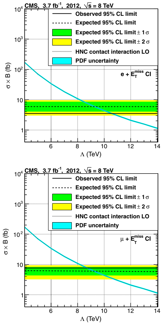
FIG. 6 (color online). Bayesian limits on the cross section times the single channel branching fraction ( \sigma \times \mathcal{B} ) for contact interactions (HNC model) in the electron + E_T^{\text{miss}} (top) and the muon + E_T^{\text{miss}} channel (bottom) based on an integrated luminosity of 3.7 \text{ fb}^{-1} of \sqrt{s} = 8 \text{ TeV} data. The expected limit in either channel excludes values of the new interaction scale \Lambda < 9 \text{ TeV} . The observed limit, driven by the data, excludes \Lambda < 10.5 \text{ TeV} (8.8) in the electron (muon) channel. The signal efficiency is independent of \Lambda .
